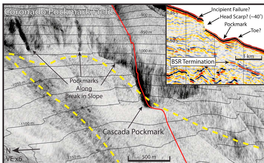
Figure 11. Perspective view of backscatter-drapped bathymetry looking east showing the upper portion of Coronado Pockmark Field and Cascada Pockmark. Dashed yellow line traces the approximate location of the upslope BSR termination. Red line shows location of seismic line shown in the inset. Inset: Seismic line extracted from 3-D volume along the axis of Cascada Pockmark and along the canyon upslope. Note the possible incipient failure and very steep (~40°) slope directly above the pockmark and termination of the BSR below.
