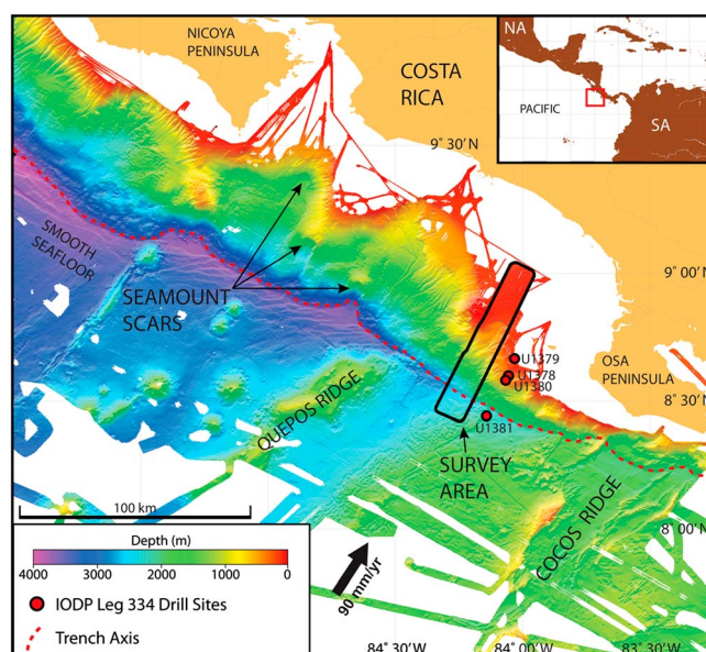
Figure 1. Color-filled multi-beam bathymetry map showing seafloor structure offshore western Costa Rica. Large 100 m grid cell bathymetry dataset collected by IFM-GEOMAR and downloaded from the Marine Geoscience Data System. Location of high-resolution CRISP survey outlined by a solid black line west of Osa Peninsula. Red box within the inset outlines the regional location of base map. White represents gaps in multi-beam coverage, whereas brown denotes land. IODP Leg 334 drill sites labeled with black-rimmed red circles. Note the lack of coverage in shallow water across the continental margin (red colors), except for the CRISP survey.
