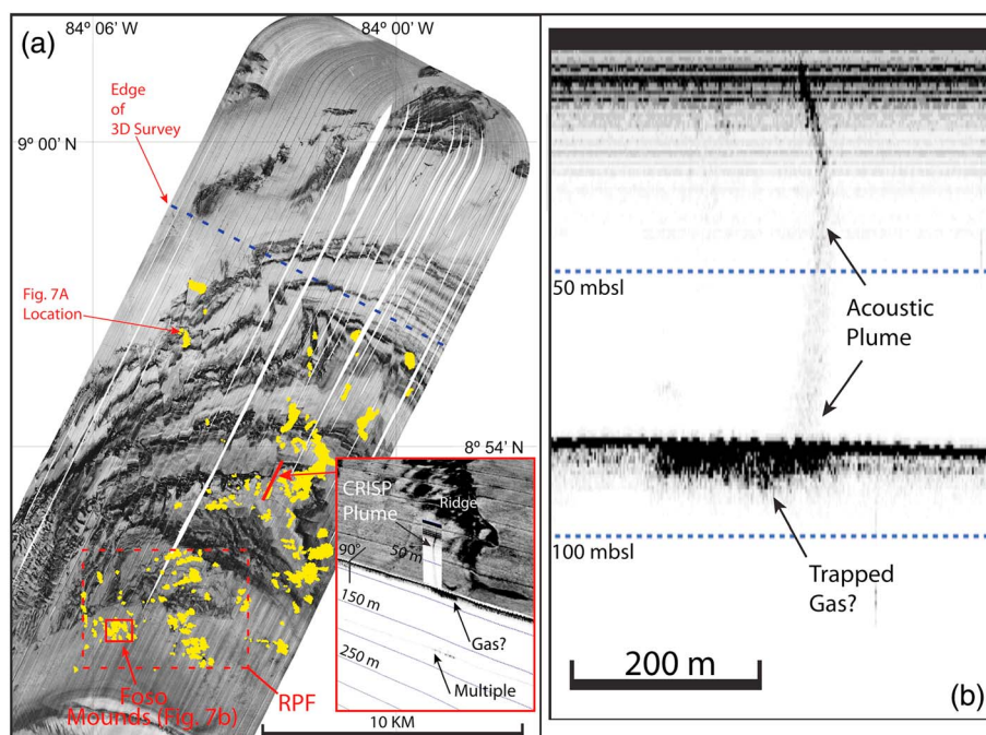
Figure 3. (a) Detailed backscatter mosaic of outer-shelf region. Overlaid yellow patches represent locations of reversed polarity bright spots mapped within the upper 200 m of the 3D seismic volume. Solid red line denotes location of 3.5 kHz profile. Dashed red box outlines location of Racimo Pockmark Field (RPF), which is shown in greater detail on Figure 9a. Solid red box shows location of Foso Mounds (Figure 3b). Dashed blue line traces the edge of the 3-D seismic survey. Inset shows perspective view (red arrow denotes look direction) of backscatter-draped bathymetry and acoustic plume imaged in the water column on a 3.5 kHz profile. (b) 3.5 kHz profile (shown in Figure 3a inset) showing acoustic plume and possible gas trapped below the seafloor.
