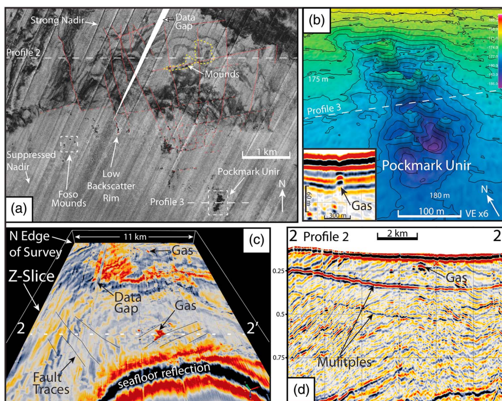
Figure 8. (a) Overhead view of backscatter mosaic showing Racimo Pockmark Field, Foso Mounds, and Pockmark Unir. Solid red lines follow fault traces apparent in exposed beds, and dashed red lines trace faults inferred by linear chains of pockmarks and mounds. Dashed yellow line shows location of large bright spot shown in Figures 8c and 8d. Note how the nadir backscatter artifact is subdued as swath overlap increases to the south with increasing depth. (b) Perspective bathymetric view of Pockmark Unir. Note complicated internal structure of highs and lows. Inset: Profile 3 across Pockmark Unir (inset) shows reverse polarity bright spot directly under the pockmark. (c) Perspective view of 3-D seismic Z-slice approximately 30 m below Racimo Pockmark Field. Dashed white line shows location of Profile 2 in Figure 8d. (d) Seismic Profile 2 located on Figures 8a and 8c. Note the reverse polarity bright spot located at the top of the anticline, just below the seafloor, sliced by the z-slice shown in Figure 8c.
