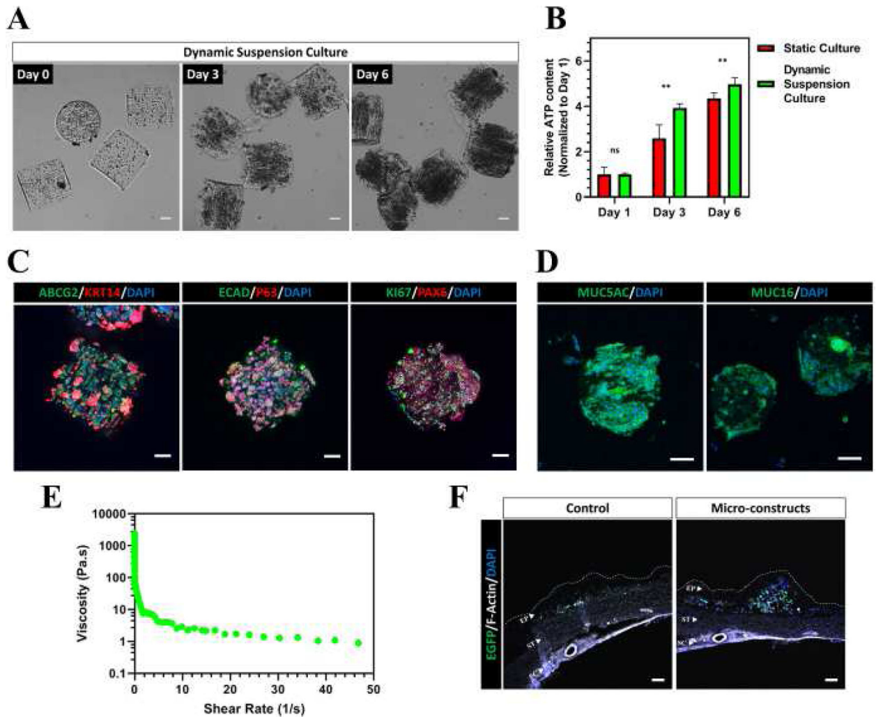
Figure 4. Dynamic Suspension Culture and Subconjunctival Injectable Delivery of CjSC-loaded Hydrogel Micro-constructs.
