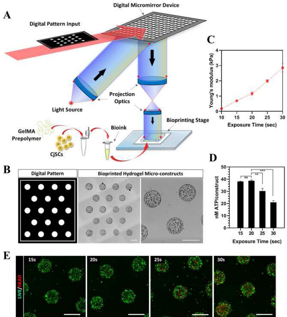
Figure 2. Bioprinting of CjSC-loaded Hydrogel Micro-constructs with Tunable Mechanical Properties.
