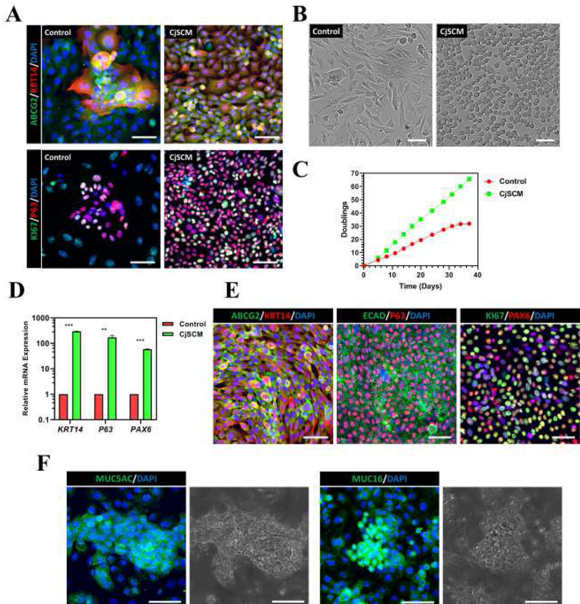
Figure 1. Conjunctival Stem Cell Expansion Medium (CjSCM) with Small Molecule Cocktail Facilitates in vitro Expansion of CjSCs.
