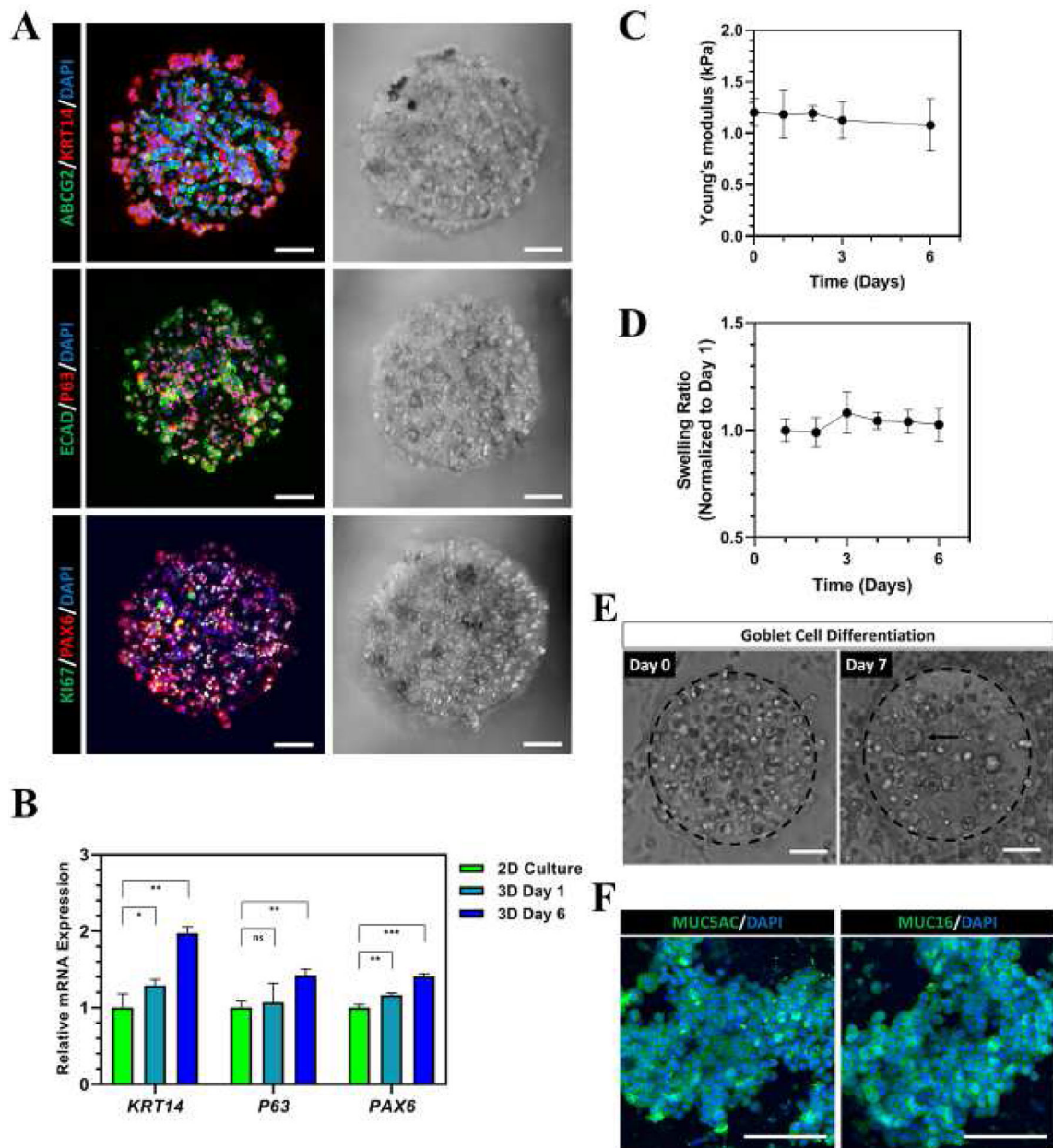
Figure 3. Bioprinted Hydrogel Micro-constructs Support 3D Culture of Functional CjSCs.
