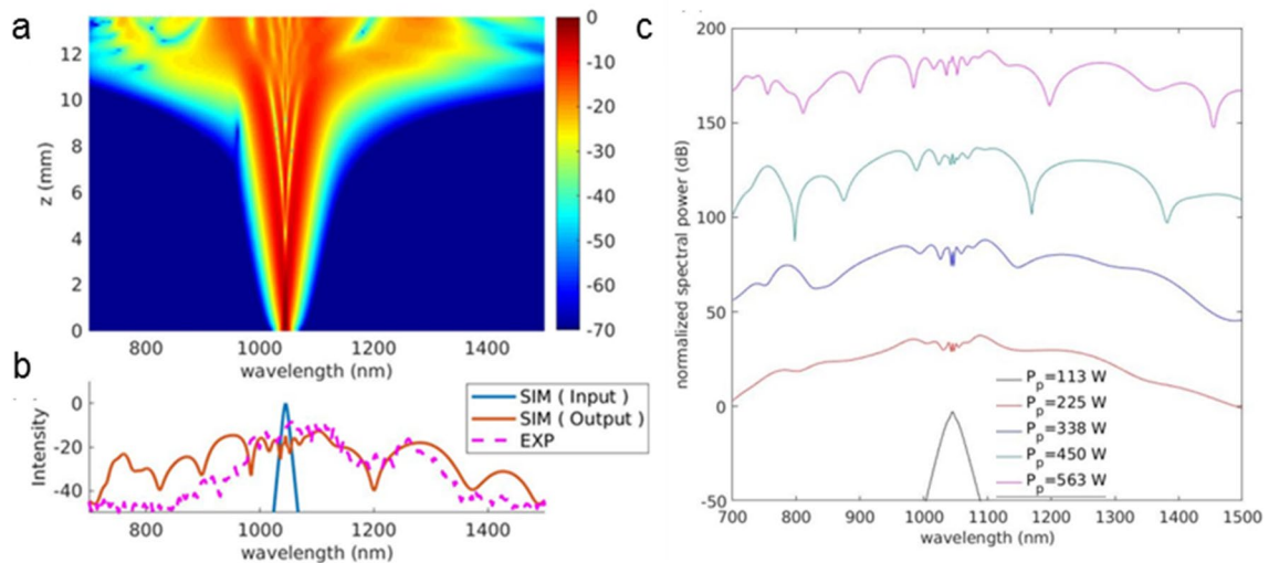
Figure 6. (a) Simulated SCG of TM 10 mode at the peak power of 563 W coupled into the Ta 2 O 5 waveguide: (a) spectral intensity; (b) comparison of the simulated (in red) and measured (in magenta) spectra at the output. The spectrum of the input pulse is shown in blue. (c) Estimated SC spectrum generated with ultrafast pulses of various peak powers coupled to the Ta 2 O 5 waveguide.
