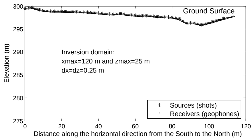
Figure 9. Seismic survey geometry at the NT2 area and the inversion domain
