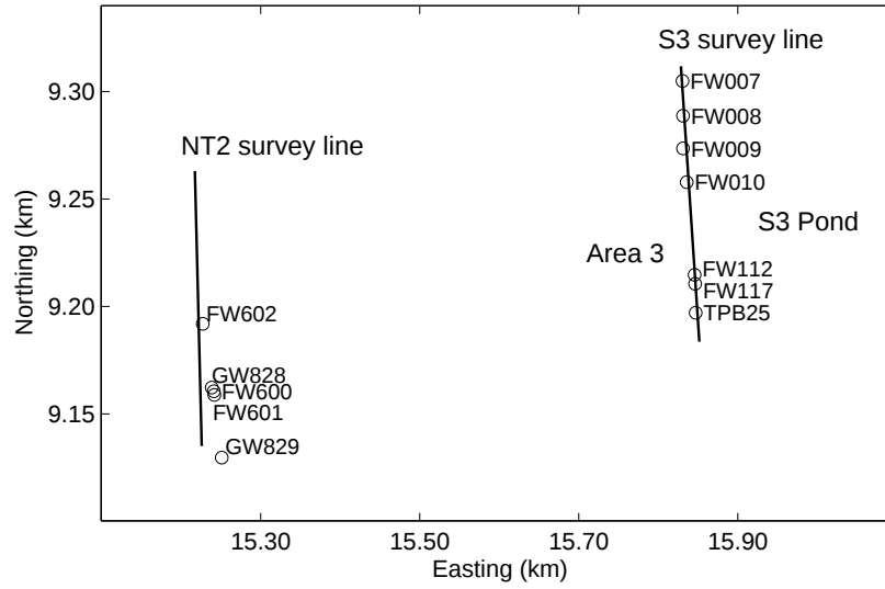
Figure 3. Seismic refraction survey lines and wellbores at the NT2 and S3 pond areas
