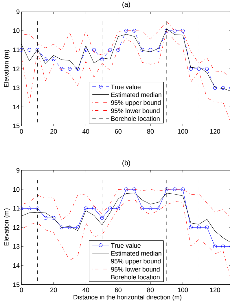
Figure 7. Estimated interface locations (a) with depth constraints and (b) without depth constraints
