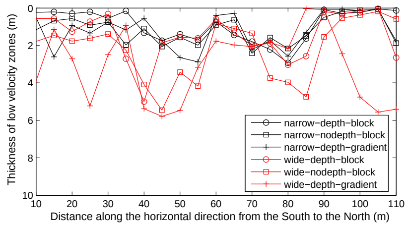
Figure 12. Effects of prior information on the estimates of thickness for the NT2 dataset
