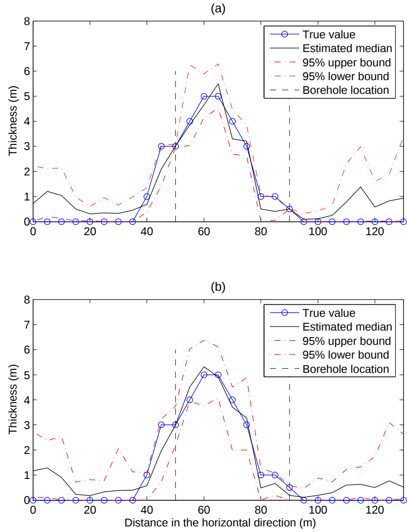
Figure 8. Estimated thickness of low velocity zones (a) with depth constraints and (b) without depth constraints
