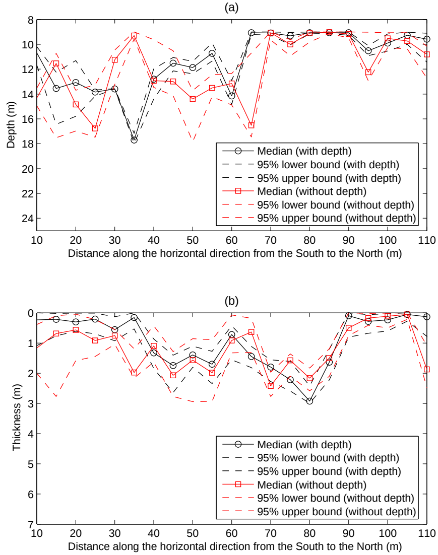
Figure 11. Uncertainty associated with inversion at the NT2 area : (a) interface locations, and (b) thickness of low velocity zones
