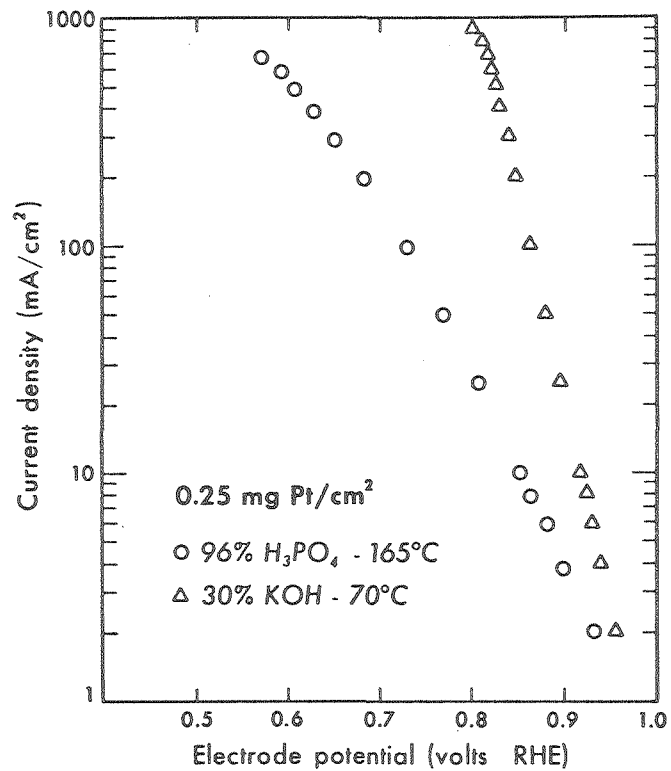
Figure 8. Comparison of the polarization curves for a fuel cell type electrode with colloidal Pt on Vulcan catalyst in acid and alkaline solutions. 1 atm. O 2 .
