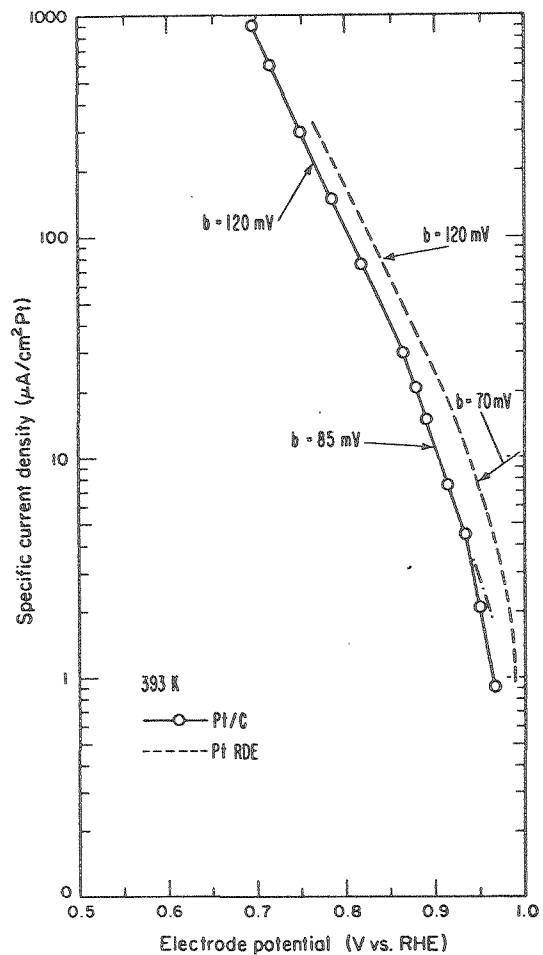
Figure 7. Comparison of the polarization curves for the colloidal Pt on Vulcan carbon catalyst versus a smooth Pt rotating disk electrode. 85% H 3 PO 4 .
