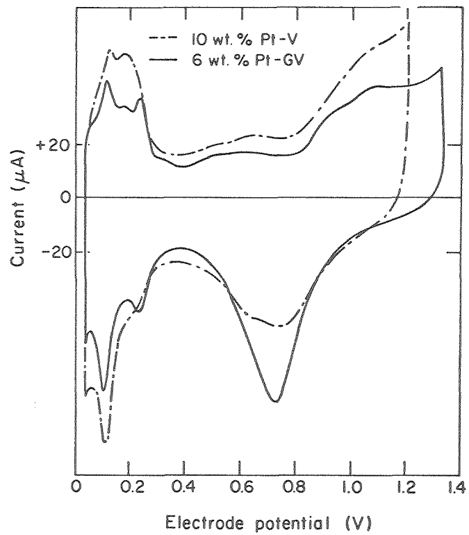
Figures 5 (above) and 6 (right). Cyclic voltammety curves for supported Pt catalysts in acid (above) and for smooth Pt (upper right) and supported Pt (lower) in alkaline solution.
