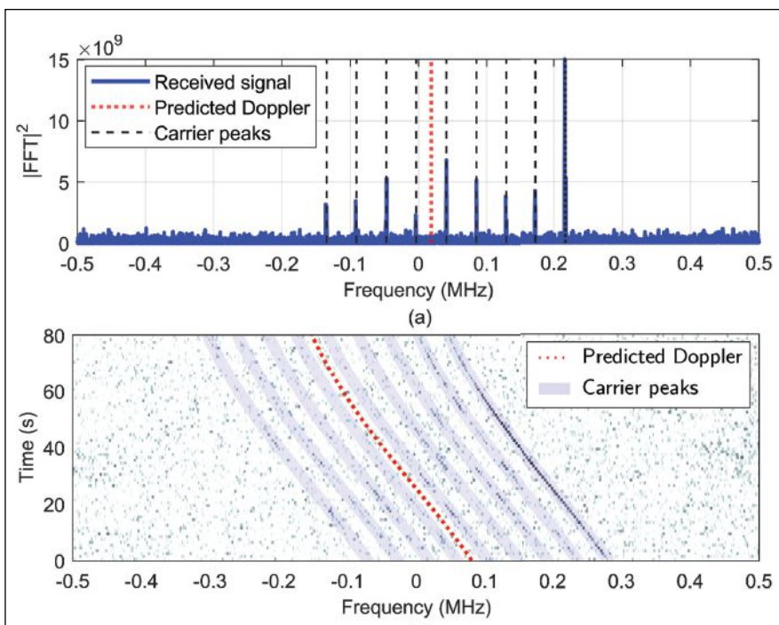
FIGURE 6 (a) the square of the magnitude of the signal's FFT and (b) the Waterfall plot of the FFT over an 80-second interval.
