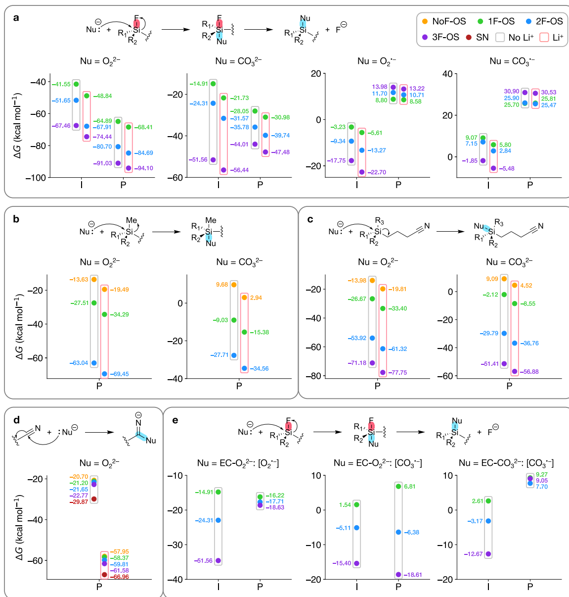
Figure 6. Relative free energies of the intermediate states (I) and products (P) of various chemical reactions between noncoordinated (gray-boxed)/ Li^+ -coordinated (pink-boxed) OS additives and various nucleophiles. (a) Bimolecular nucleophilic substitution ( S_N2 ) via backside attack of an F atom attached to Si. (b) Nucleophilic addition ( A_N ) via backside attack of a methyl group attached to Si. (c) A_N via backside attack of the -(CH_2)_3-C\equiv N moiety attached to Si. (d) A_N via attack of the cyano-C. (e) Same as (a), with the nucleophile being the [O_2^{2-}]/[CO_3^{2-}] part of ethylene carbonate oxide ion and the [CO_3^{2-}] part of ethylene dicarbonate ion. Nonreacting additive moieties are shown as squiggly lines in the molecular structures.
