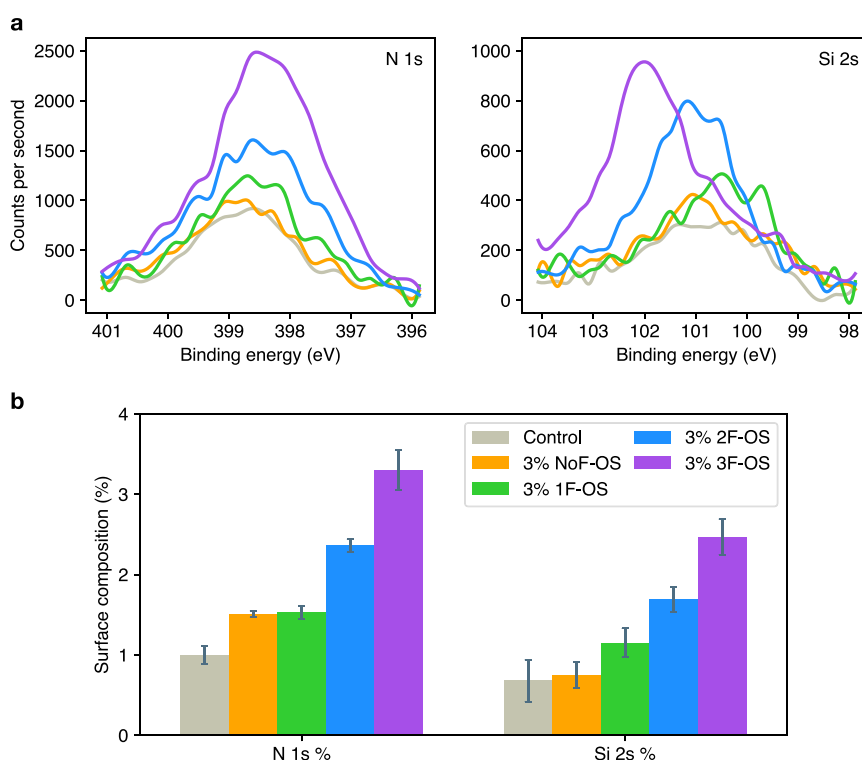
Figure 7. XPS surface analysis of NMC811 cathodes after formation in SC-NMC811/Gr pouch cells for control 1 and 3% NoF-OS/1F-OS/2F-OS/3F-OS electrolytes: (a) N 1s and Si 2s spectral regions; (b) percent composition of nitrogen and silicon out of all surface elements.
