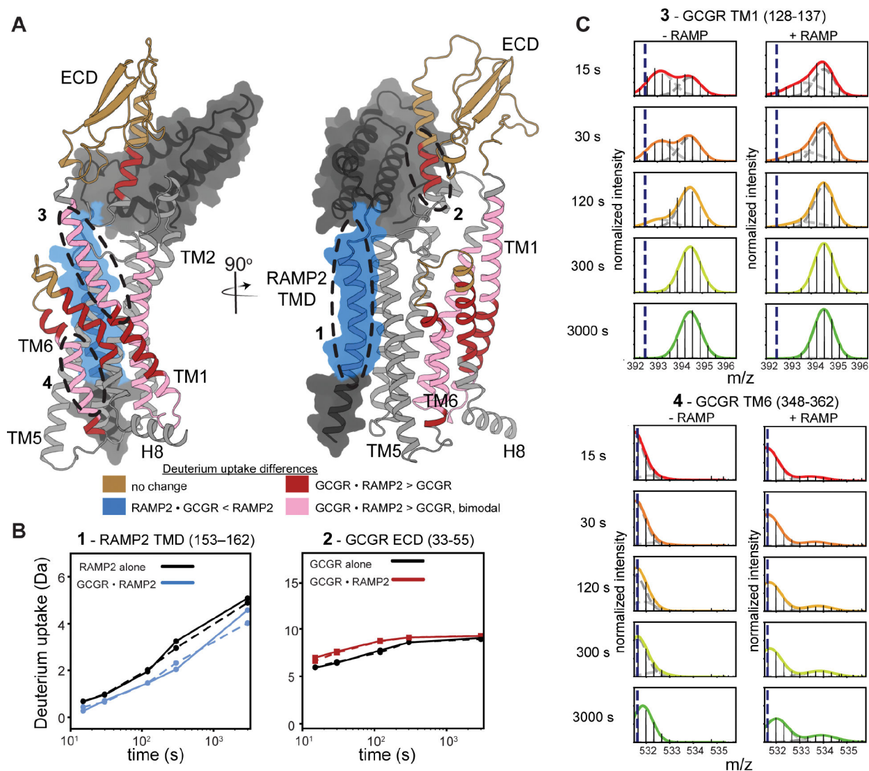
Figure 3. RAMP2 binding broadly increases the conformational heterogeneity in GCGR. (A) AlphaFold model of GCGR-RAMP2 complex onto which changes in HDX upon complex formation are plotted. (B) Example HDX-MS exchange curves in the presence and absence of excess RAMP2 (independent replicates in solid and dashed lines) show that several key regions of the RAMP2 (153–162) and receptor (33–55) are impacted by heterodimer complex formation. (C) HDX-MS plots showing bimodal distribution in GCGR TM1 (residues 128–137), an indication of conformational heterogeneity. This heterogeneity is increased in the presence of RAMP2. Though not present in the absence of RAMP2, a bimodal distribution is induced in TM6 (348–362) upon addition of RAMP2.
