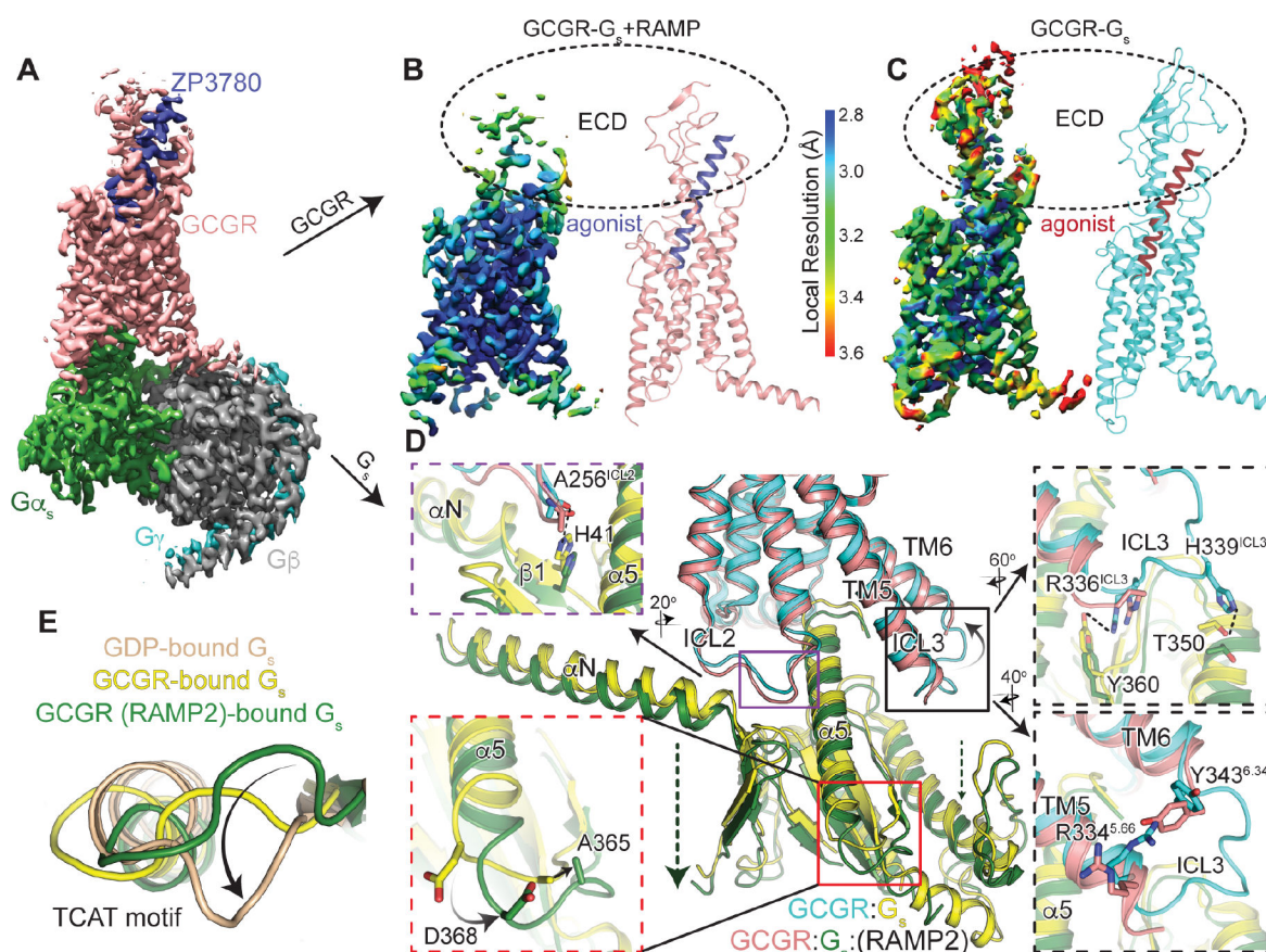
Figure 5. Structure of GCGR-G s in the presence of RAMP2.
