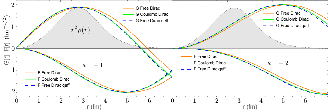
Figure 2: The Dirac Coulomb solutions G(r) and F(r) for the highly relativistic outgoing electron produced in \mu \rightarrow e conversion in ^{27}\text{Al} (green line) are compared to the free solution (orange) and to the free solution evaluated with \vec{q}_{\text{eff}} (blue dashed), for low partial waves ( \kappa = -1, -2 ). The nuclear charge distribution is shown by the shading (arbitrary normalization). The agreement between the Coulomb and plane wave solutions evaluated with q_{\text{eff}} is quite good, particularly over the relevant region where the nuclear density is concentrated.
