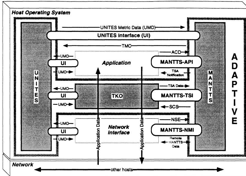
Figure 1: ADAPTIVE System Architecture
