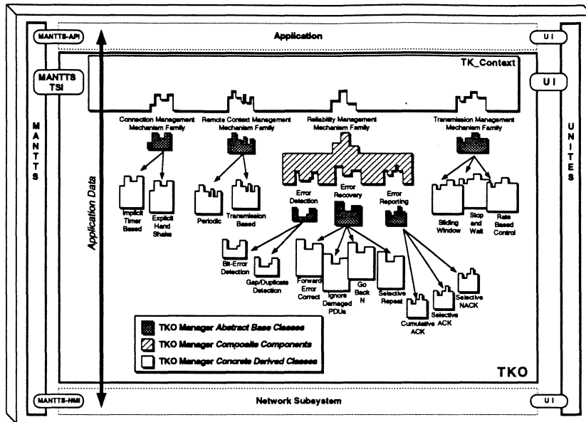
Figure 5: TKO Mechanism Class Library
