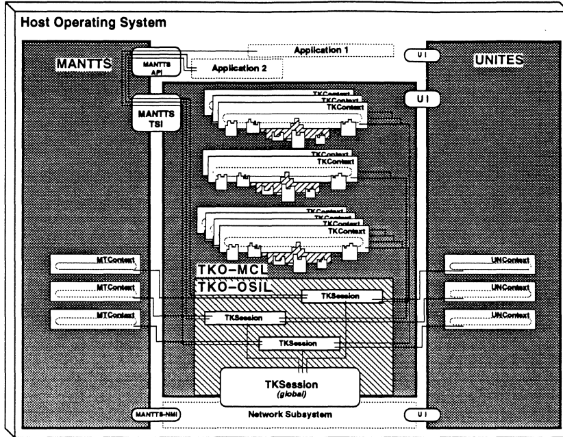
Figure 4: Transport Kernel Objects
