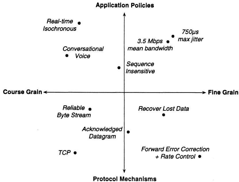
Figure 2: Hierarchical Specification
