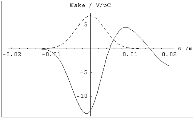
Figure 2: Short-range longitudinal wake potential.
