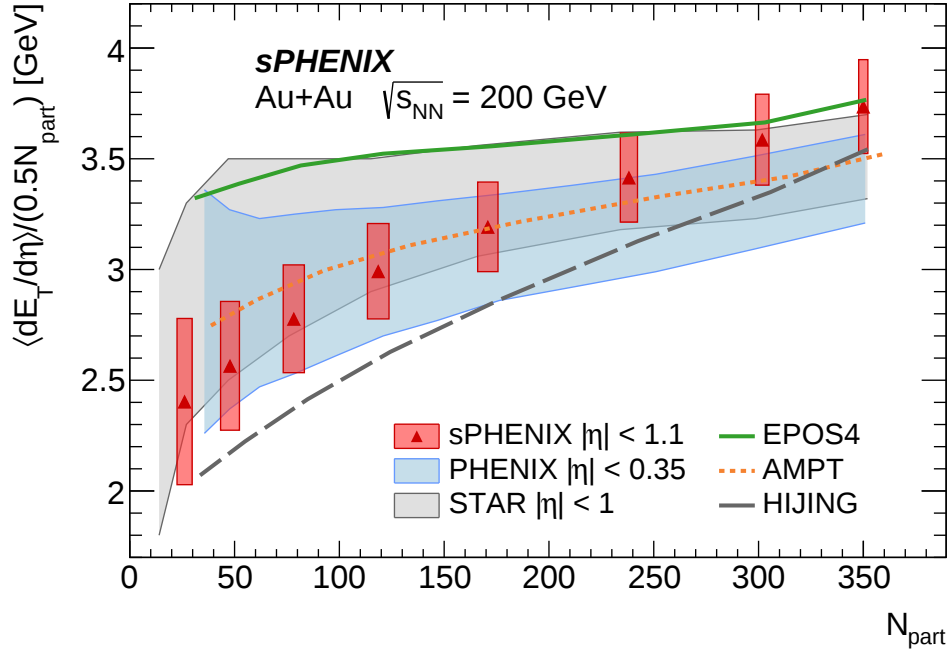
Figure 6: Measured dE_T/d\eta normalized by the estimated number of participant pairs ( 0.5N_{\text{part}} ), as a function of N_{\text{part}} , using the full calorimeter system (red triangles). The vertical size of the boxes indicates the total uncertainty, which includes the uncertainty in N_{\text{part}} . Measurements by PHENIX [4] (blue band) and STAR [5] (gray band) are shown for comparison, with the vertical size of the band indicating the uncertainty range. MC event generator predictions are shown for EPOS4 (solid green line), AMPT (dotted orange line), and HIJING (dashed black line).
