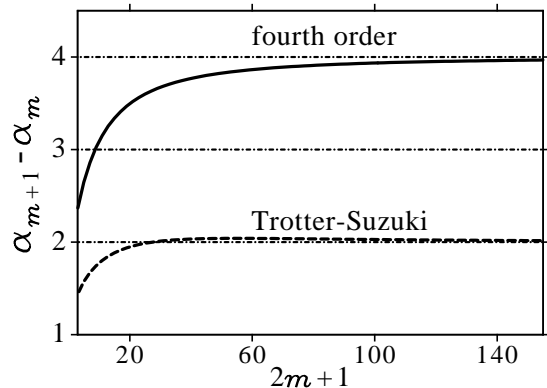
FIG. 1: Numerical demonstration that the convergence order of the short-time approximation given by Eq. (11) is 4, at least for the He cage problem. For comparison, the convergence order of the trapezoidal Trotter-Suzuki approximation is also featured.
