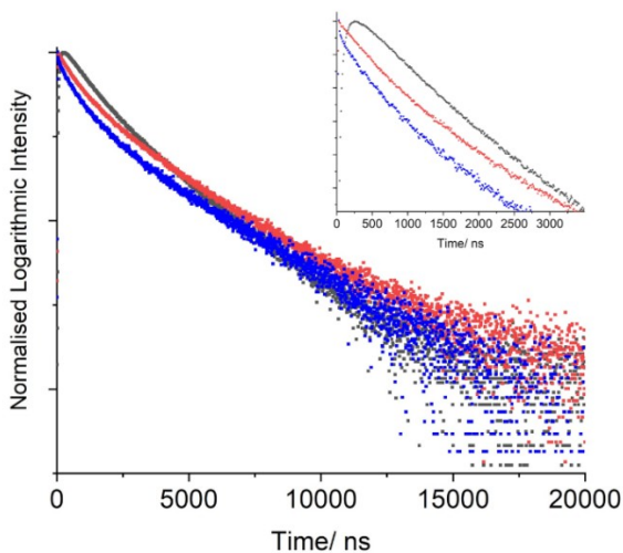
Figure 8. Decay of [NdYb] with \lambda_{exc} = 584 nm (black trace), [NdYb] with \lambda_{exc} = 375 nm (red trace) and [GdYb] ( \lambda_{exc} = 375 nm) (blue trace) at 980 nm in the solid state. Inset: zoom on time to highlight the rise time.
