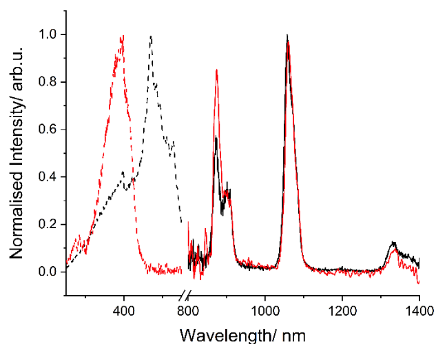
Figure 6. Normalised excitation ( \lambda_{em} = 1060 nm) (dotted trace) and emission ( \lambda_{exc} = 375 nm) (full trace) spectra of [NdNd] in the solid state (black trace) and in methanol (red trace) at room temperature.
