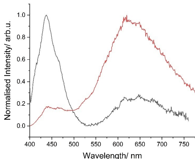
Figure 3. Emission spectra of [GdGd] ( \lambda_{\text{exc}} = 375 nm) in methanol at room temperature (black trace) and 77K (red trace).
