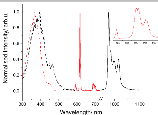
Figure 5. Normalised excitation at \lambda_{em} = 616 nm (dotted black trace) and \lambda_{em} = 980 nm (dashed red trace) and emission ( \lambda_{exc} = 375 nm) (full red and black trace) spectra of [EuYb] ( 2 ) in methanol at 77 K.
