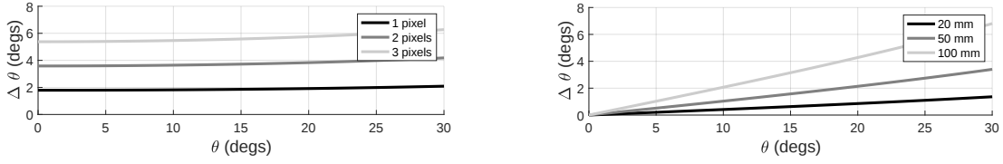
Figure 2.6: Gaze direction error \Delta\theta as a function of gaze direction \theta for: (a) different values of error in \mathbf{pc}_x - \mathbf{pec}_x (1, 2, 3 pixels); (b) different values of errors in D (20, 50, 100 mm.)
