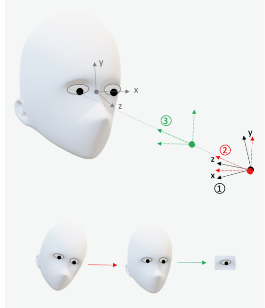
Figure 2.3: Data normalization
