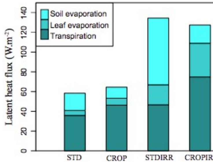
Fig. 8 Simulated 2004–2006 averaged latent heat flux partitioned into three components for the four models
