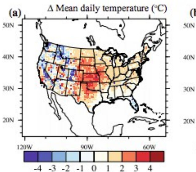
Fig. 4 Averaged (2004–2006) difference between th temperature, and c precipitation
