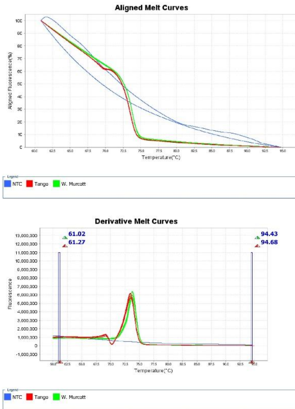
Figure 2.19 Real-Time PCR of DC-7 Short Deletion. Aligned melt curves (upper panel) and derivative melt curves (lower panel) of five W. Murcott leaf DNA samples (green) and five Tango leaf DNA samples (red) with NTC control (blue).
