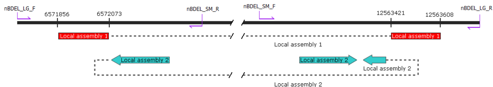
Chromosome 2 Breakpoints
