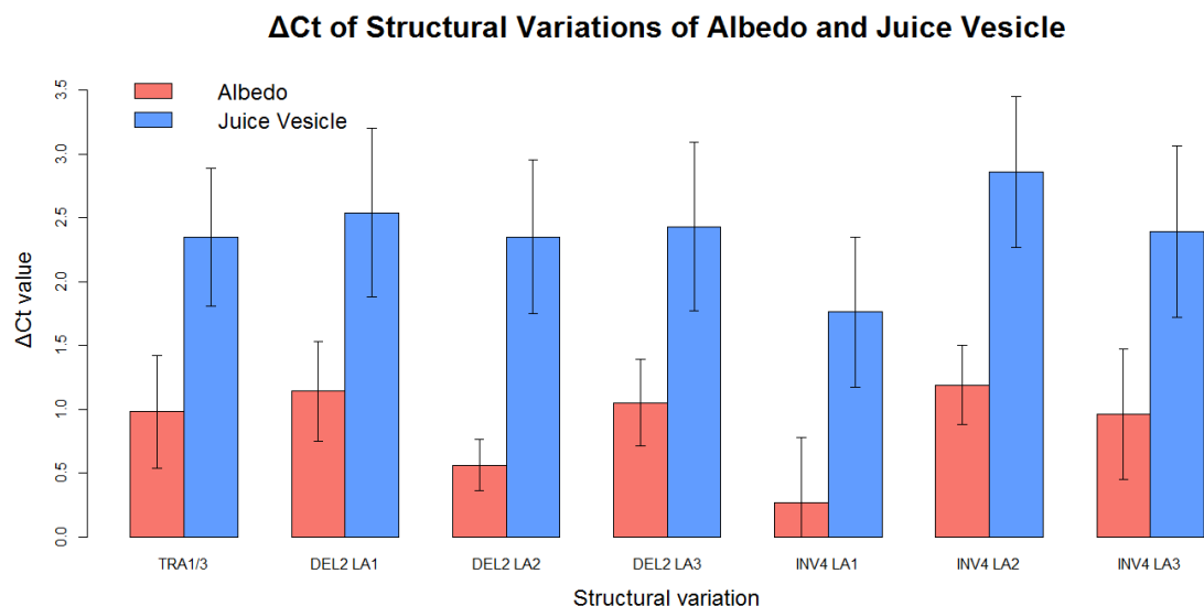
Figure 4.16 Comparison of Mean \Delta Ct Values of Seven Local Assemblies (LA) of Three Putative Structural Variations (TRA1/3, DEL2 and INV4) Between Albedo DNA (Red Bars) and Juice Vesicle DNA (Blue Bars) of Tango. Primer pairs used for amplification were TRA1/3: NB13 and NB14, DEL2 LA1: NB81 and NB18, DEL2 LA2: NB87 and NB88, DEL2 LA3: NB93 and NB94, INV4 LA1: NB143 and NB144, INV4 LA2: NB115 and NB116, and INV4 LA3: NB153 and NB154. Error bars represent standard deviation.
