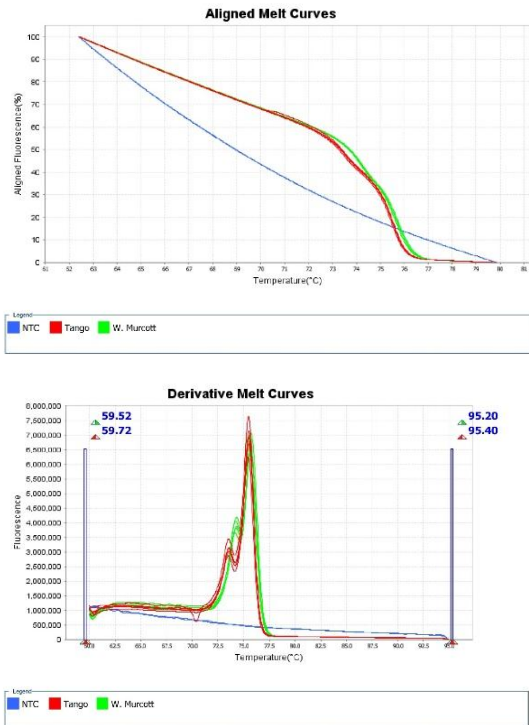
Figure 2.21 Real-Time PCR of Del3 Short Deletion. Aligned melt curves (upper panel) and derivative melt curves (lower panel) of five W. Murcott leaf DNA samples (green) and five Tango leaf DNA samples (red) with NTC control (blue).
