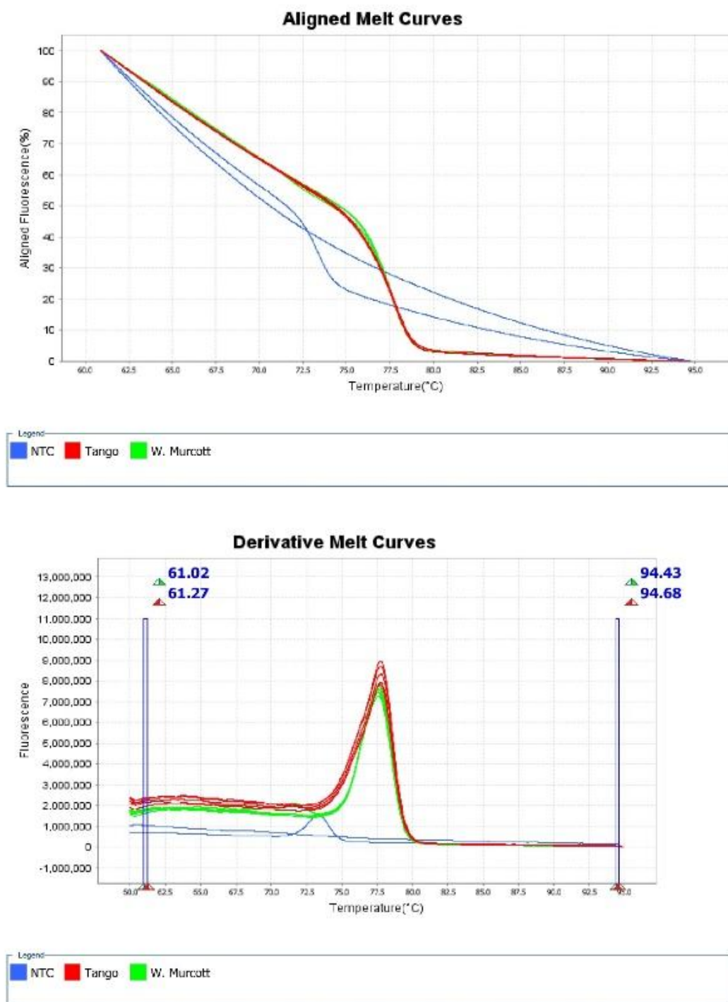
Figure 2.23 Real-Time PCR of Del3-3 Short Deletion. Aligned melt curves (upper panel) and derivative melt curves (lower panel) of five W. Murcott leaf DNA samples (green) and five Tango leaf DNA samples (red) with NTC control (blue).
