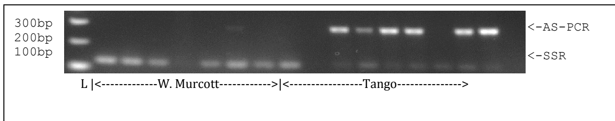
Figure 2.13 Allele-Specific PCR for DC-1 Short Deletion. Eight W. Murcott leaf DNA samples and eight Tango leaf DNA samples amplified with DC-1 short deletion primer sets (DC1_deletion_ASPCR_F and DC1-R) and background control (SSR#133 CF-ATG05) primer sets (SSR#133 forward and SSR#133 reverse).
