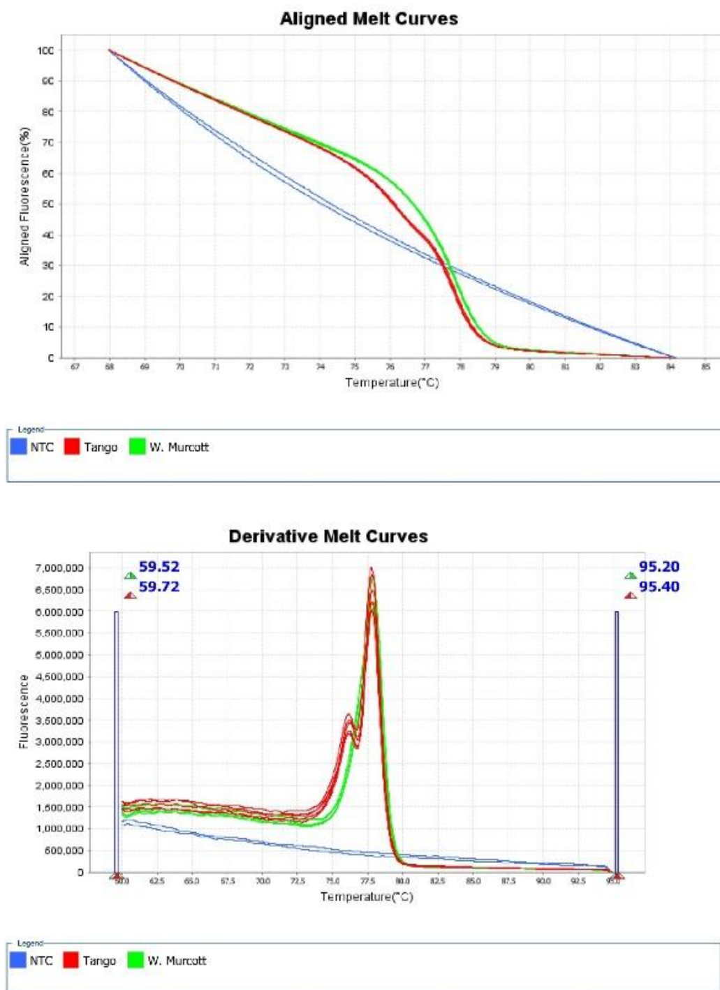
Figure 2.20 Real-Time PCR of Del2 Short Deletion. Aligned melt curves (upper panel) and derivative melt curves (lower panel) of five W. Murcott leaf DNA samples (green) and five Tango leaf DNA samples (red) with NTC control (blue).
