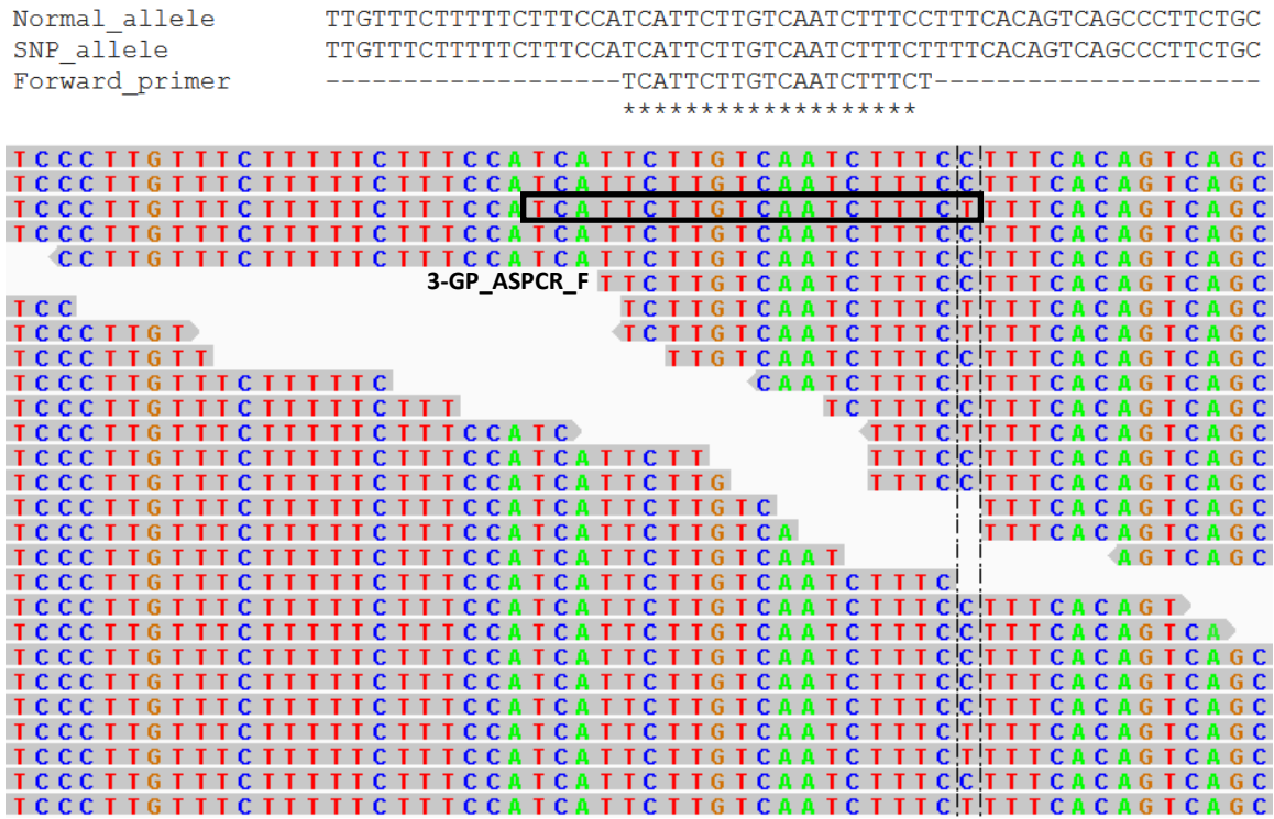
Figure 2.3 3-GP SNP Forward Primer Design. Illumina reads from Tango leaf DNA are aligned to Citrus clementina reference genome v1.0. Figure shows the region spanning the SNP position of 3-GP (C/T in dashed box) and SNP-specific primer position (black box). The SNP position is contained at the 3'-end of the sequence of 3GP_ASPCR_F primer TCATTCTTGTCAATCTTTCT, where T is a Tango-specific nucleotide in this locus.
