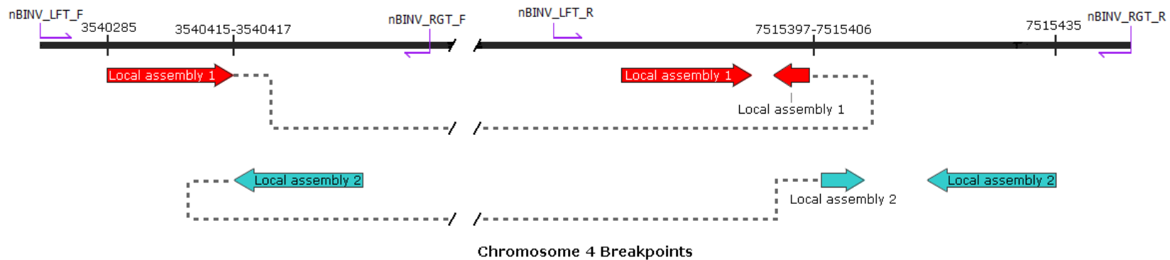
Figure 3.15 Schematic Diagram of INV4 with Two Local Assemblies and Conventional PCR Primer Sets. Two breakpoints at approximately 3540415 th bp - 3540417 th bp and 7515397 th bp - 7515406 th bp on chromosome 4 are shown on the reference genome (top black line). The approximate alignment positions of local assembly 1 (red) and local assembly 2 (teal) to the reference genome are shown, where arrows indicate there are unknown inner nucleotides between the two ends of the assembly (not to scale). The dashed lines indicate the consecutive sequence of local assemblies were split-aligned to two positions on the chromosome. The position and direction of conventional PCR primer sets are shown in purple arrows (not to scale).
