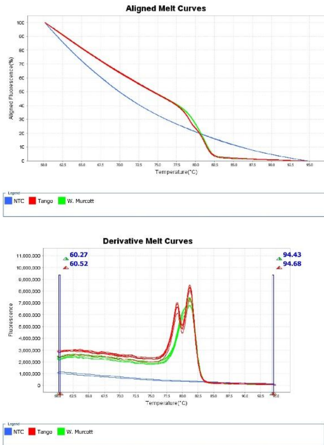
Figure 2.24 Real-Time PCR of Del2-3 Short Deletion. Aligned melt curves (upper panel) and derivative melt curves (lower panel) of five W. Murcott leaf DNA samples (green) and five Tango leaf DNA samples (red) with NTC control (blue).
