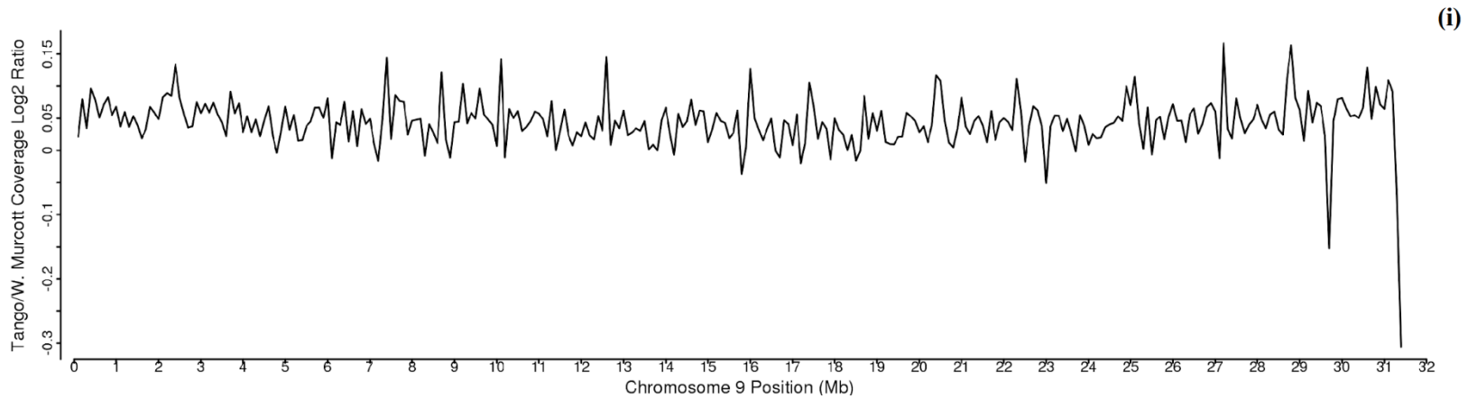
Figure 3.1 Log2 Ratio of Read Depth of Tango versus W. Murcott. (a) – (i) Nine chromosomes are divided into consecutive windows of 100 kb in size. The alignment read depth of Tango and W. Murcott within each window were counted and the log2 ratio was calculated as \log_2 \frac{\text{Tango read depth}}{\text{W. Murcott read depth}} and plotted on nine chromosomes.
