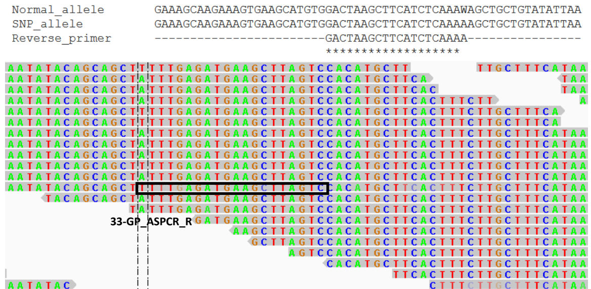
Figure 2.5 33-GP SNP Reverse Primer Design. Illumina reads from Tango leaf DNA are aligned to Citrus clementina reference genome v1.0. Figure shows the region spanning the SNP position of 33-GP (T/A in dashed box) and SNP-specific primer position (black box). The SNP position is contained at the 3'-end of the sequence of 33-GP_ASPCR_R primer GACTAAGCTTCATCTCAAAA, where A is a Tango-specific nucleotide in this locus.
