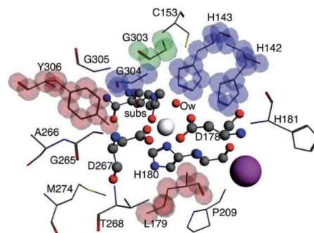
Figure 13. Structure about the active site of HDAC8 as modeled with clusters of 3–7 Å. The 3 Å system consists of the central \text{Zn}^{2+} ion (white sphere), substrate (subs), water molecule (Ow), D178, H180, and D267, all shown in ball and stick model. The 4 Å system adds L179 and Y306, shown with stick model highlighted in red. Five Å adds H142, H143, and G304, stick model highlighted in blue. Six Å includes G303, highlighted in green. The largest 7 Å system includes a \text{K}^+ ion (purple sphere) and C153, H181, P209, G265, A266, T268, M274, and G305, shown with nonhighlighted stick model. Reproduced from ref 122 with permission from the Royal Society of Chemistry.
