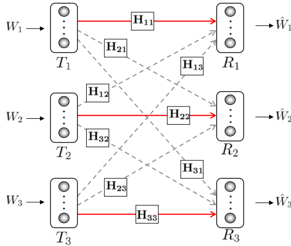
Figure 1: Three-User Interference Channel
