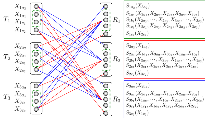
Figure 15: Three-User 4 \times 5 MIMO Interference Channel
