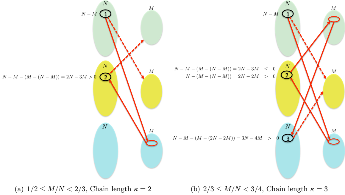
Figure 4: Subspace alignment chains leading to the M -bound, \text{DoF} \leq \frac{\kappa}{2\kappa-1}M per user. Dashed arrows indicate zero-forced interference. Numbered signal spaces shown in black ovals indicate the position of the signal space in the alignment chain. The directions of the solid arrows indicate the progression of the alignment chain.
