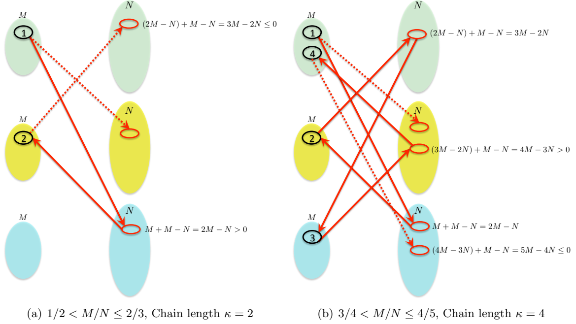
Figure 3: Subspace alignment chains leading to the N -bound, \text{DoF} \leq \frac{\kappa}{2\kappa+1}N per user. Dashed arrows indicate unaligned interference. Numbered signal spaces shown in black ovals indicate the position of the signal space in the alignment chain. The directions of the solid arrows indicate the progression of the alignment chain.
