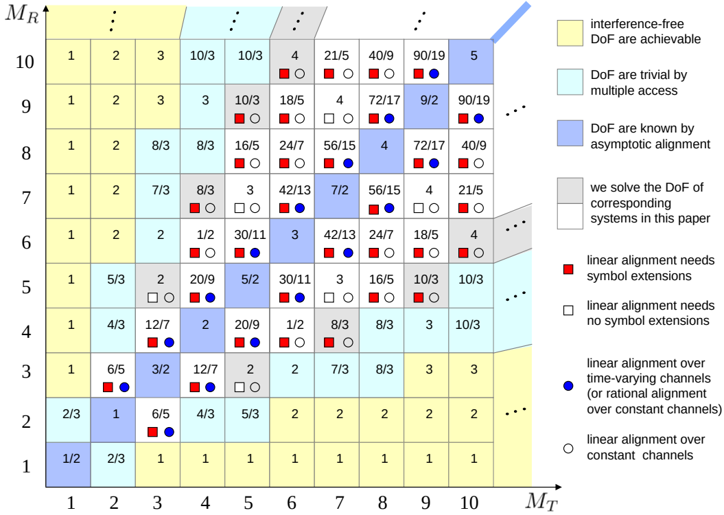
Figure 2: DoF per User (without space-extensions) of the Three-User M_T \times M_R MIMO Interference Channel
