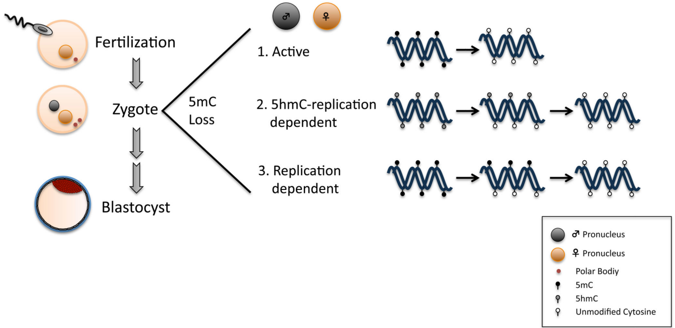
Figure 1. The male and female pronucleus each use three different mechanisms to remove 5mC from the genome (1-3). The specific pathway/s required for active removal of 5mC and 5hmC from the genome remain to be determined. DNA demethylation downstream of 5hmC occurs predominantly in the paternal pronucleus mostly by a 5hmC-replication dependent pathway. The female pronucleus mostly uses replication-dependent demethylation with a small contribution through 5hmC.
