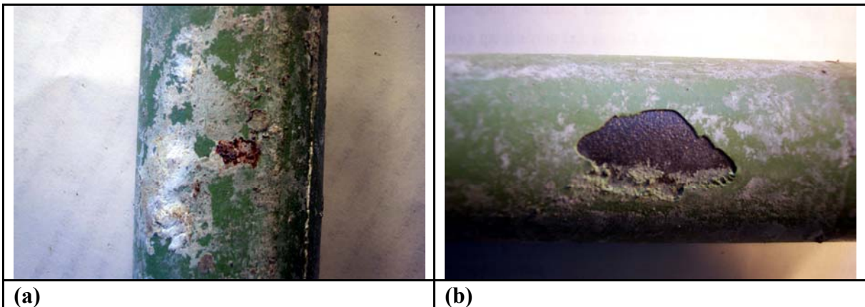
Figure 43. Corrosion product concentrated in a defective area in the epoxy coating (a); part of the epoxy coating was removed in order to observe the state of the carbon steel beneath the coating (b).
