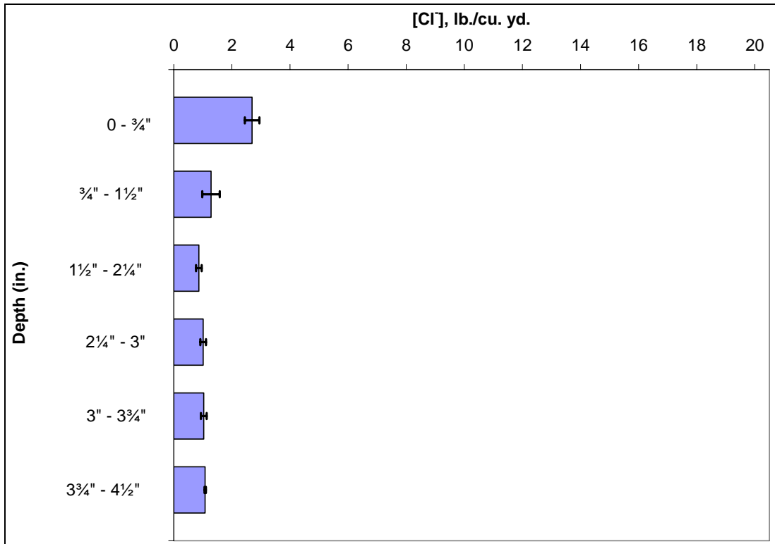
Figure 61. Chloride profile for I-5 MP 166.00 (downtown Seattle).
