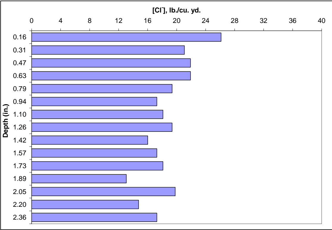
Figure 66. Chloride profile on the concrete of a carbon steel specimen.
