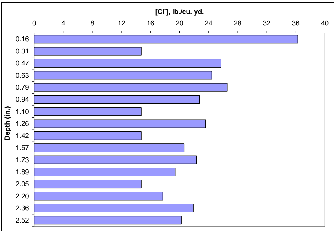
Figure 70. Chloride profile on the concrete of a non-flexible (purple) epoxy-coated specimen.
