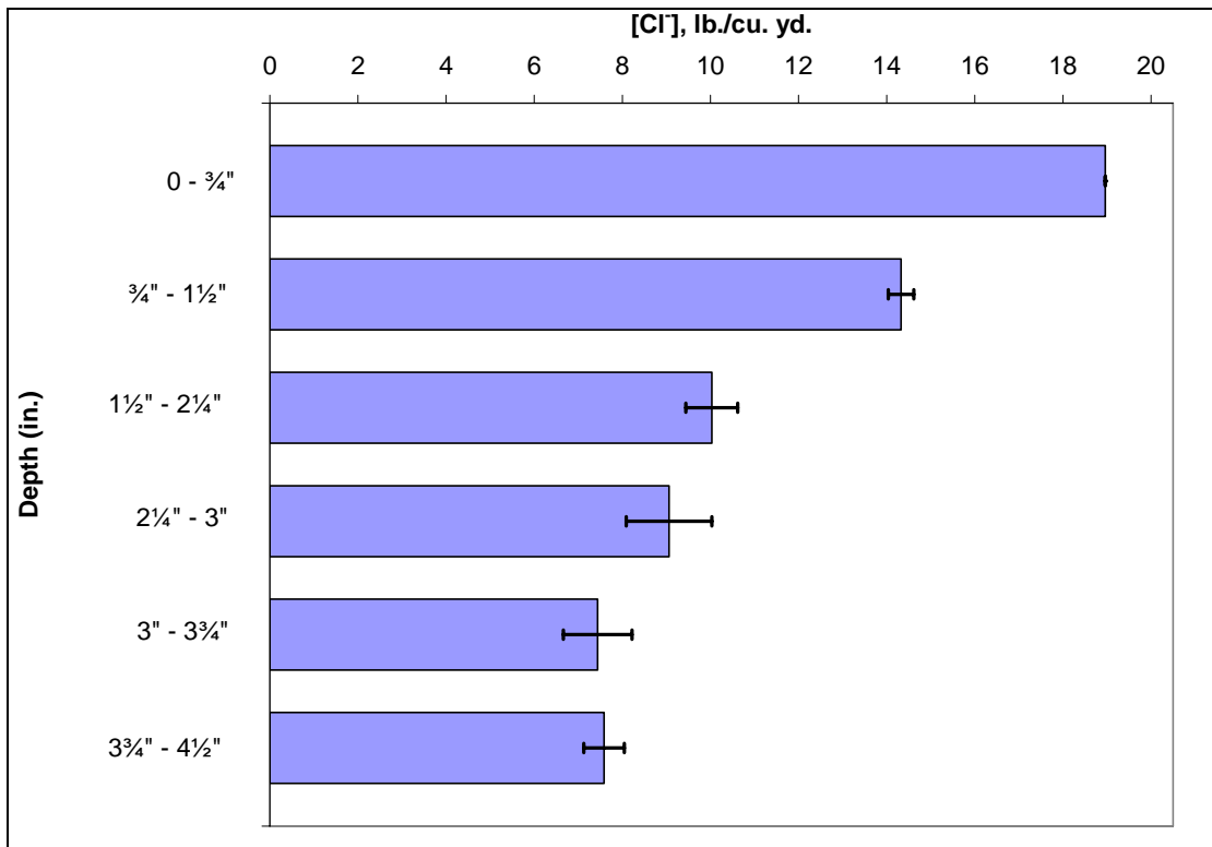
Figure 63. Chloride profile for I- 90 MP 61.304 (Price Creek).
