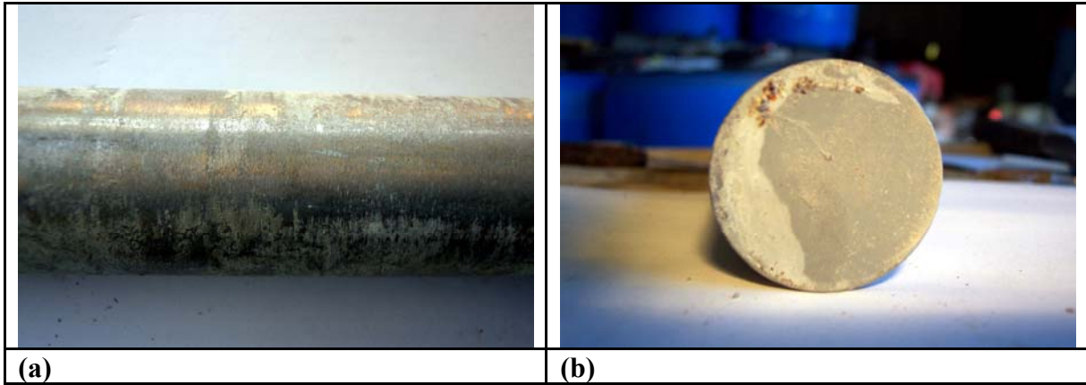
Figure 38. Stainless clad dowels. (a) General view of the center region below joint; (b) End region showing corrosion between the carbon steel core and the stainless steel outer layer.
