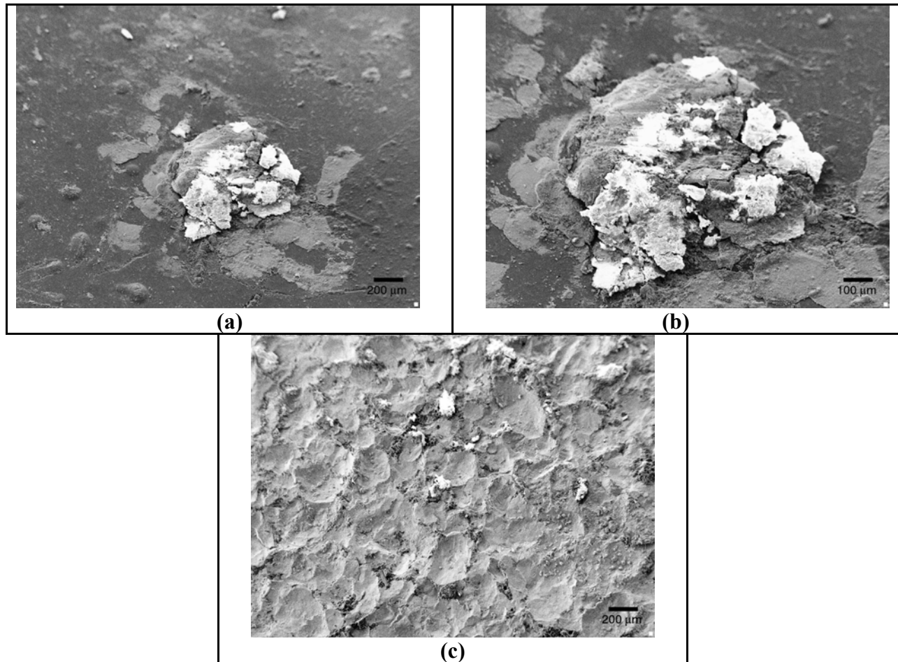
Figure 50. Purple epoxy-coated samples: (a) general view of the surface with corrosion products accumulated in a holiday, 100×; (b) zoom in the same region, 200×; and (c) condition of the steel underneath the epoxy, 200×.
