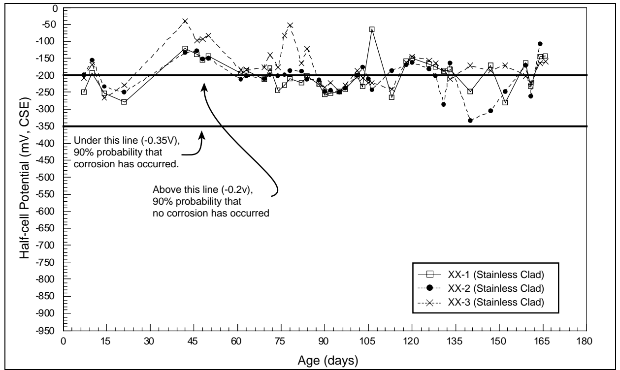
Figure 19. Half-cell potentials of stainless clad steel bars in chloride ponding at 4.4°C.
