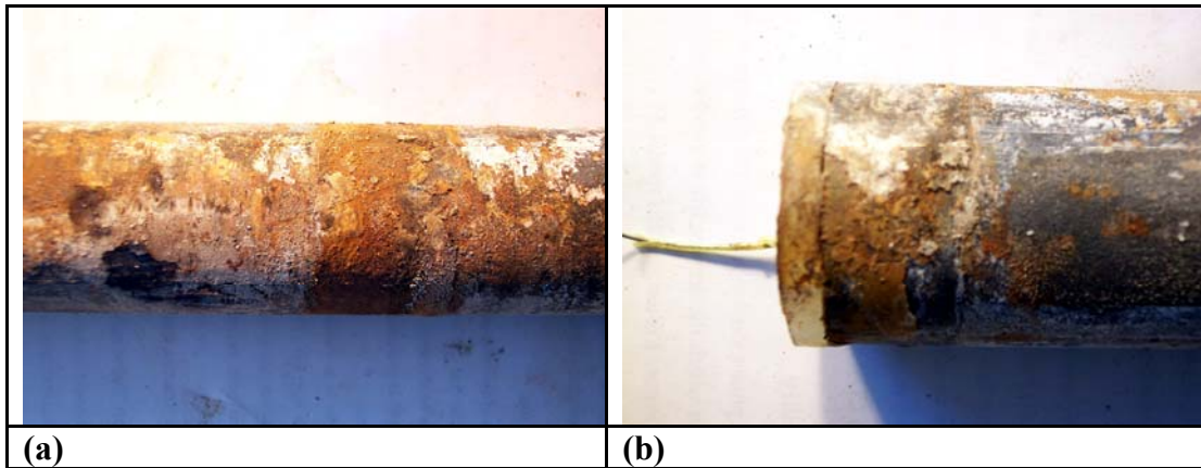
Figure 36. Carbon steel dowels. (a) Center region below joint; (b) End with electrical connection.
