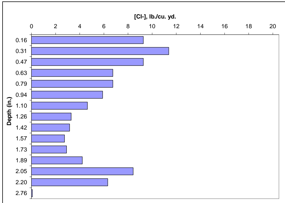
Figure 60. Chloride profile of the grout around the pavement joint (Core #6).
