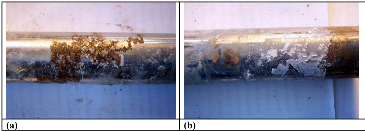
Figure 37. Microcomposite steel dowels. (a) General view of the center region below joint; (b) End region.
