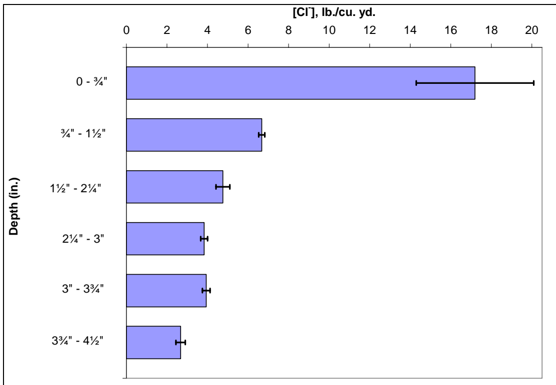
Figure 62. Chloride profile for I-90 MP 91.324 (Elk Heights).
