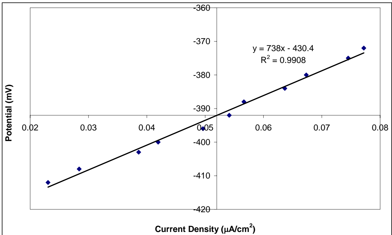
Figure 53. Linear Polarization Resistance, WSDOT slab, Specimen C.
