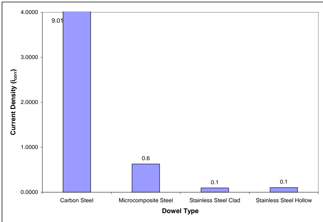
Figure 35. Comparative column plots showing average results of polarization resistance ( R_p ) and corrosion current density ( i_{corr} ) for non-coated dowels.
