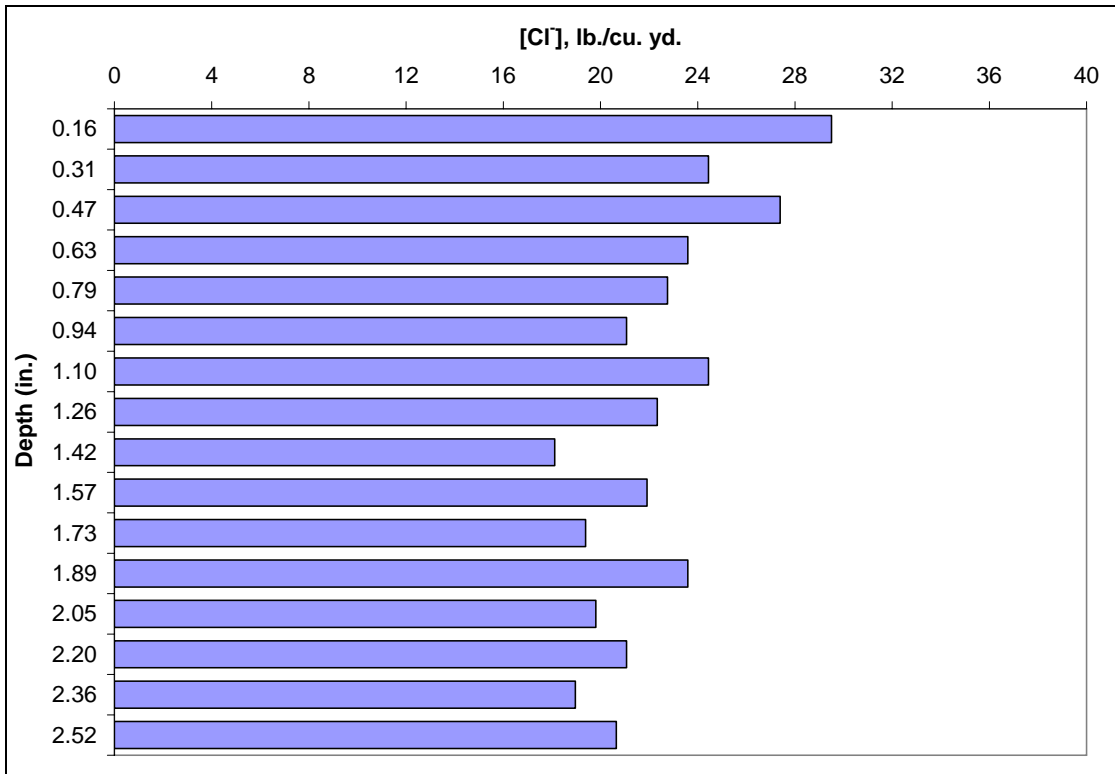
Figure 71. Chloride profile on the concrete of a microcomposite steel specimen.
