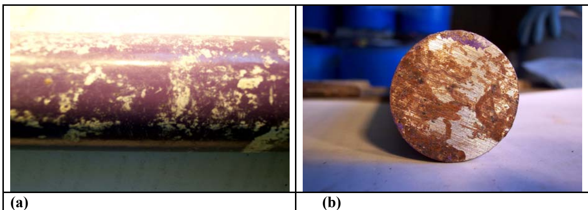
Figure 40. Epoxy-coated dowel (purple). (a) General view of the center region; (b) Corrosion was verified at the end region, underneath the epoxy seal.
