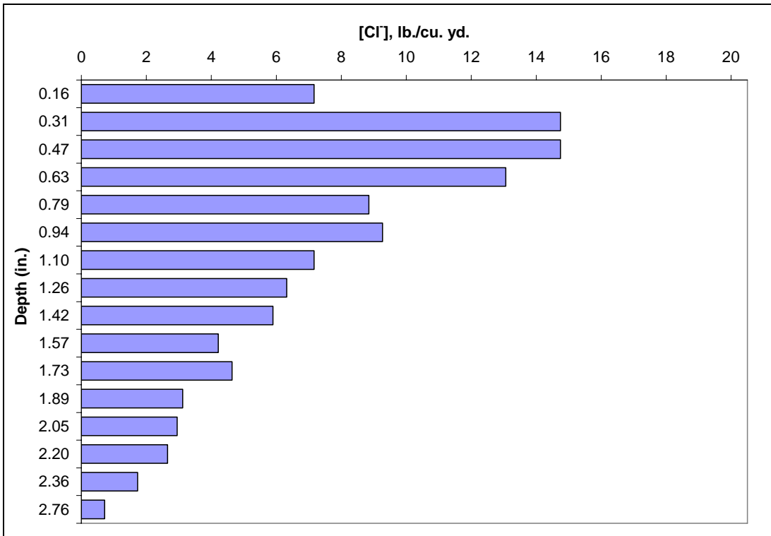
Figure 56. Chloride profile of the slab concrete (Core #1).
