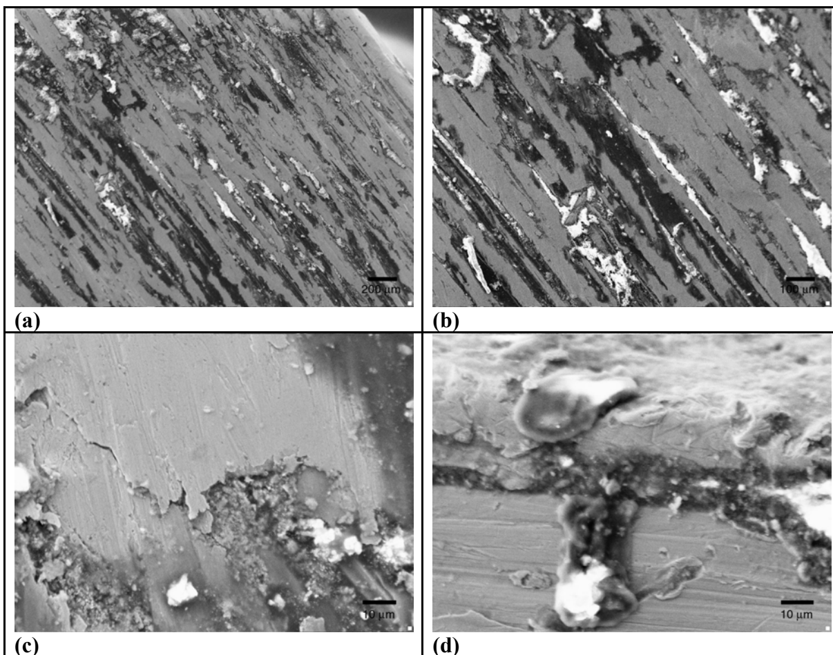
Figure 47. Stainless steel-clad samples: (a) aspect of corrosion along the surface, in a region close to the end of the dowel, 100×; (b) zoom around same region, 200×; (c) details of corrosion at the surface, interface between sound and corroded area, 2,390×; and (d) detail of corrosion at an edge, 2,320×.
