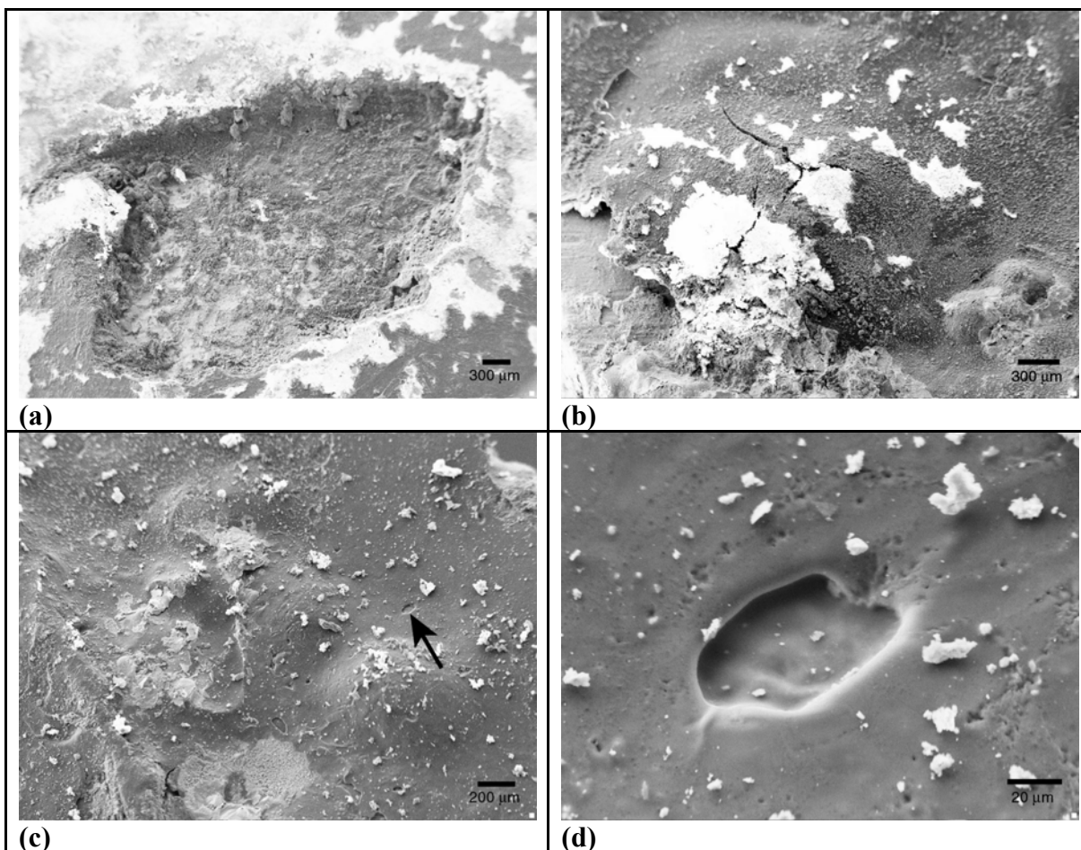
Figure 48. Gray epoxy-coated samples: (a) view of a defect in the coating, with corroded area inside, 50×; (b) another region, at an edge, where coating is lifted 75×; (c) general view of the surface, 100×; and (d) detail of a pinhole present in image (c) (see arrow), 1,500×.
