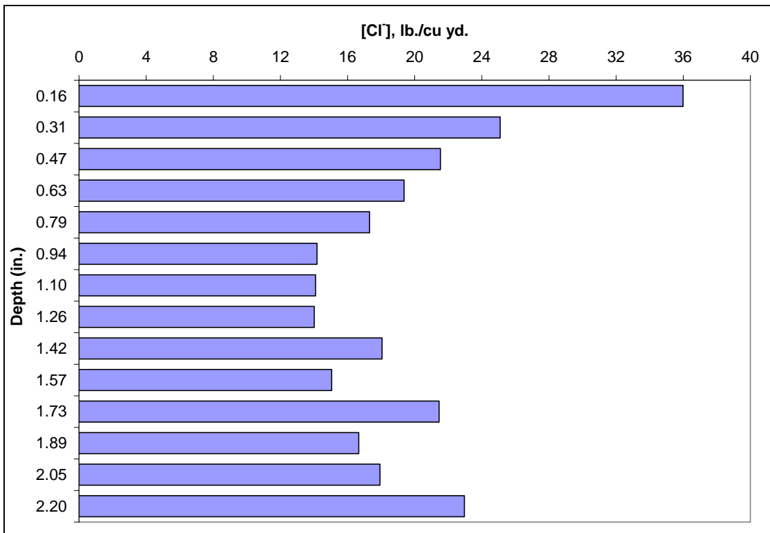
Figure 68. Chloride profile on the concrete of a stainless hollow specimen.
