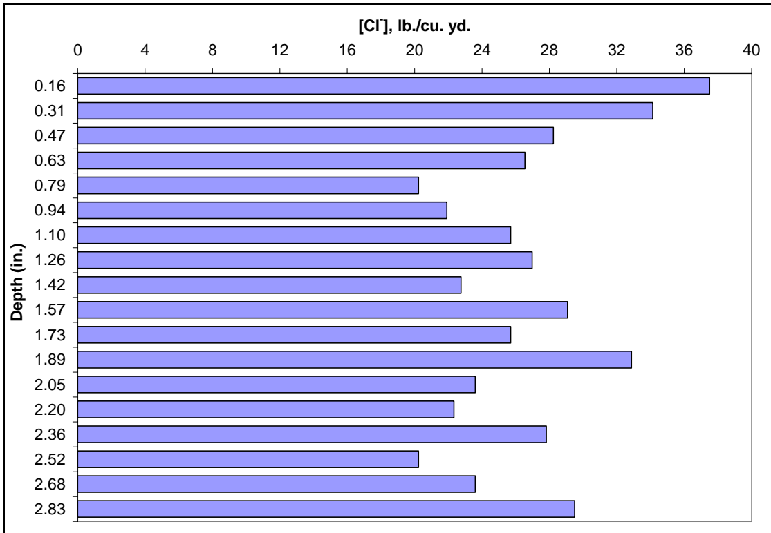
Figure 67. Chloride profile on the concrete of a stainless clad specimen.
