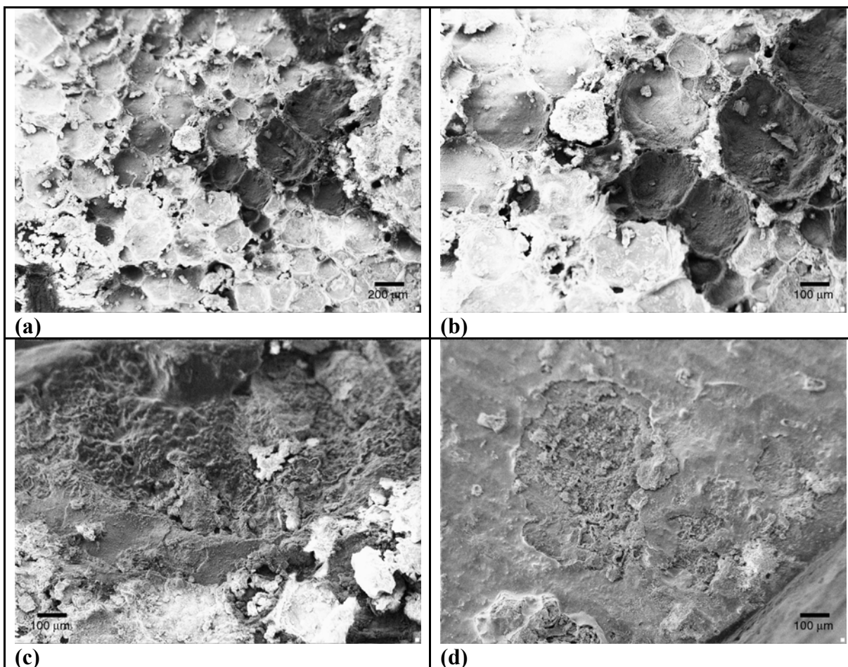
Figure 44. Carbon steel samples: (a) heavy corrosion along the dowel surface, magnification = 100×; (b) same region, 200×; (c) different region at the surface, 200×; and (d) corrosion at the bar end, 100×.
