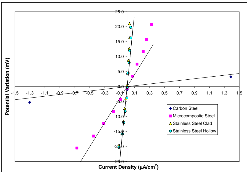
Figure 34. Detail of the region around the half-cell potential. The greater the slope, the higher the corrosion resistance.
