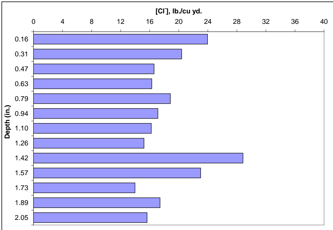
Figure 69. Chloride profile on the concrete of a flexible (green) epoxy-coated specimen.
