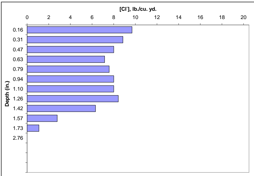
Figure 59. Chloride profile of the grout around the pavement joint (Core #5).
