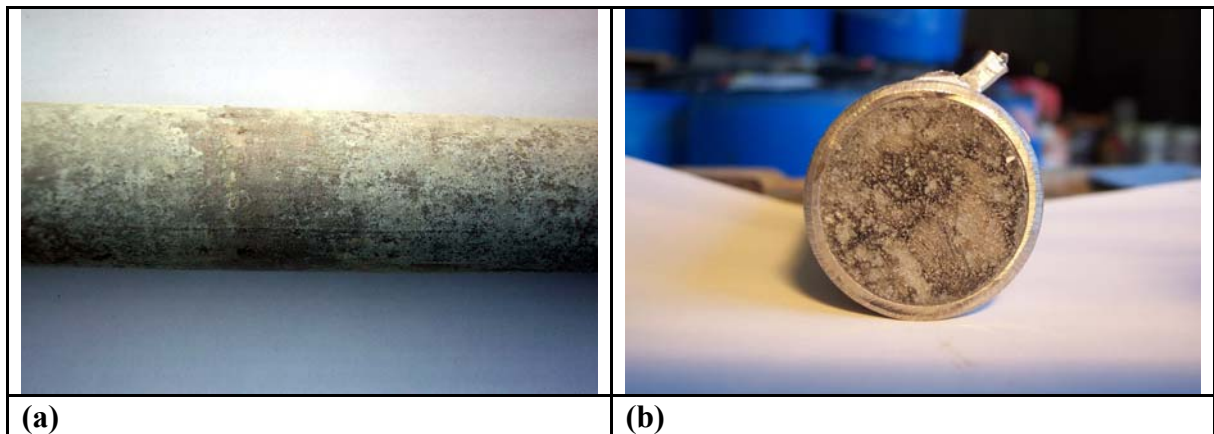
Figure 39. Stainless hollow dowels. (a) General view of the center region below joint; (b) End region showing grouted core.
