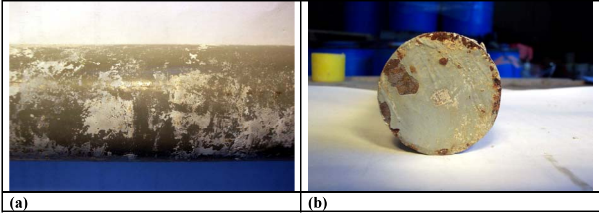
Figure 41. Epoxy-coated dowel (gray). (a) General view of the center region; (b) Corroded edges at the end of dowels.
