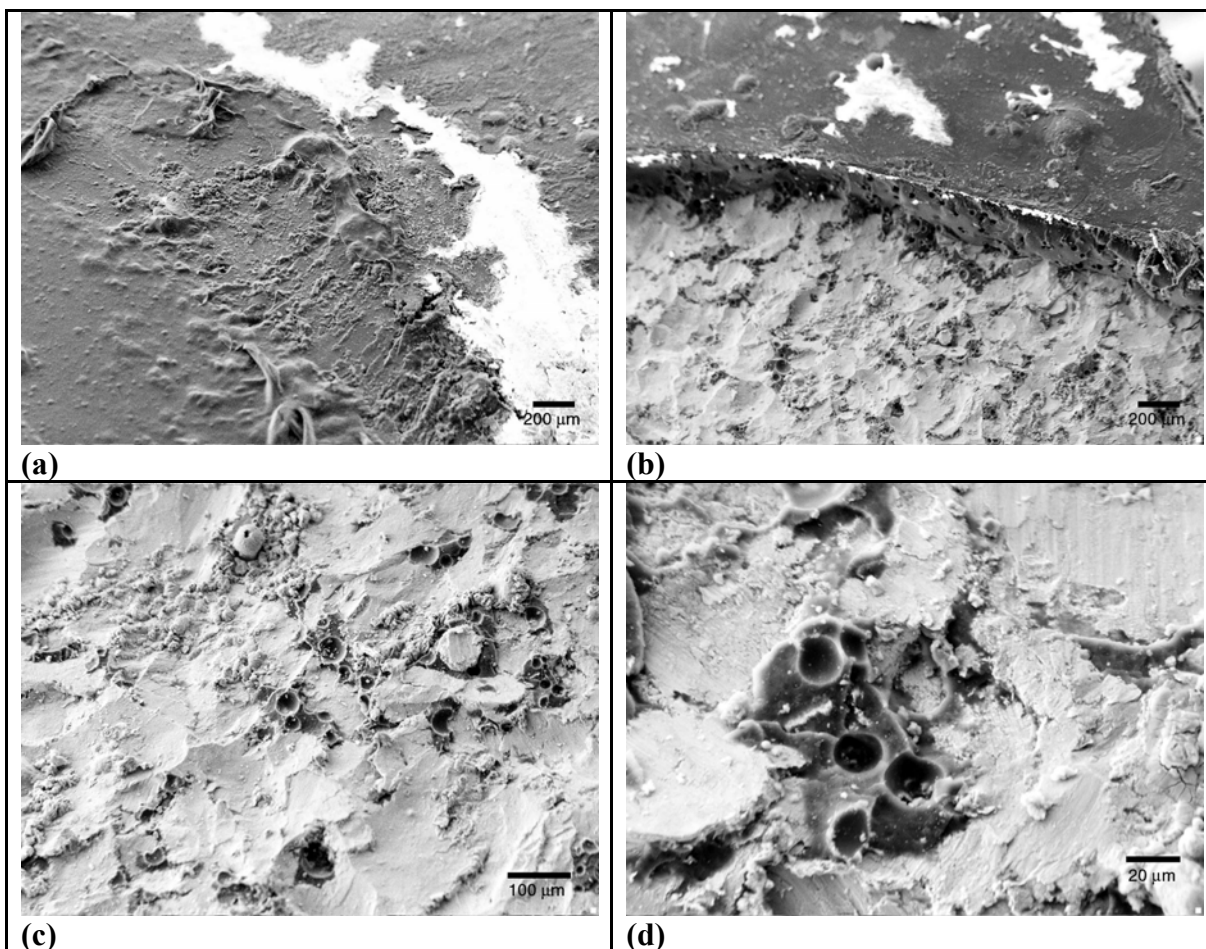
Figure 49. Green epoxy-coated samples: (a) general view of the surface, 100×; (b) region where part of the epoxy coating was removed, 100×; (c) condition of the steel underneath the epoxy, 302×; and (d) detail of corroded area and pits present under the coating, 1,330×.
