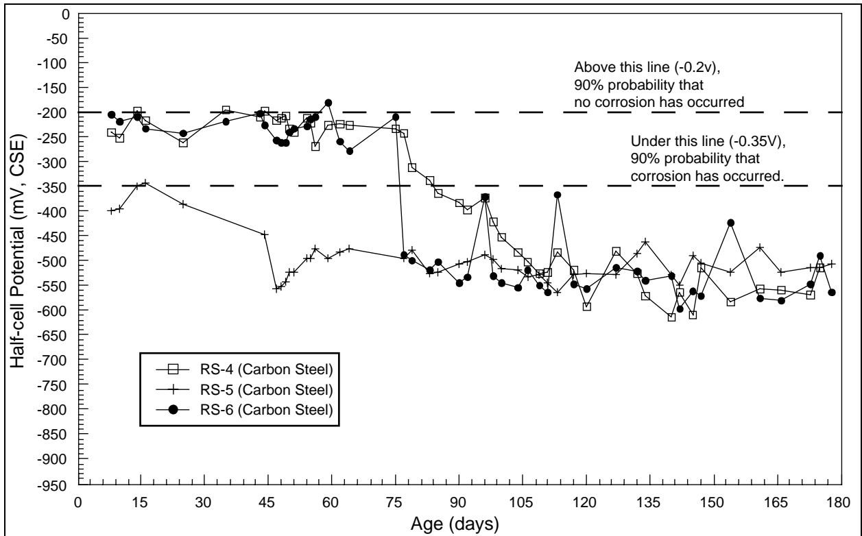
Figure 12. Half-cell potentials of carbon steel bars in chloride ponding at 40–43°C.
