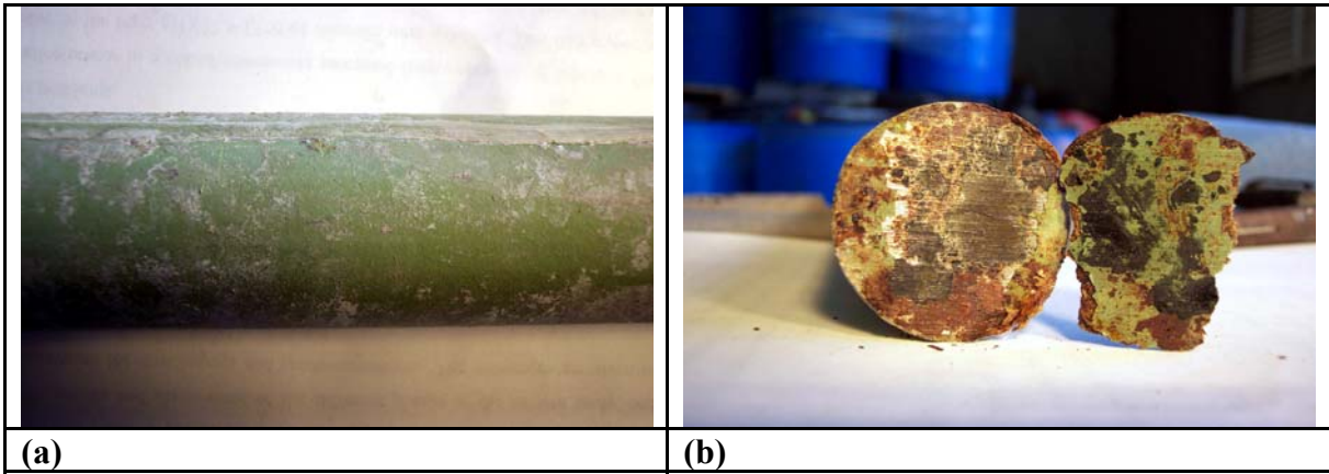
Figure 42. Epoxy-coated dowel (green). (a) General view of the center region; (b) Corroded edges and corrosion underneath coating at the end of dowels.
