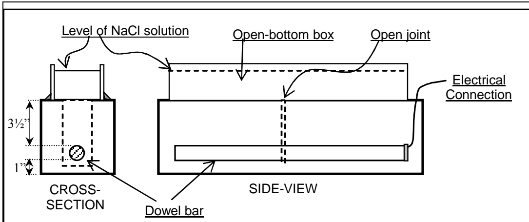
Figure 9. Experiment setup to accelerate corrosion using chloride ponding.
