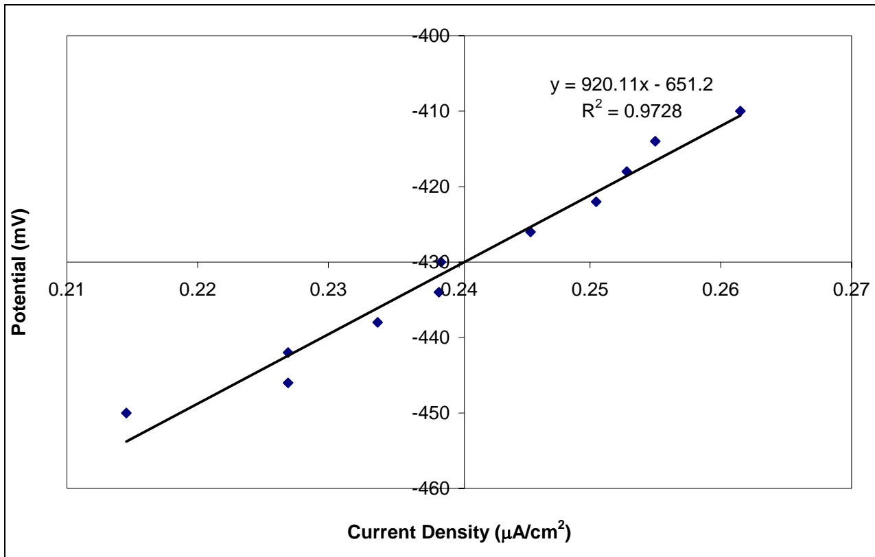
Figure 51. Linear Polarization Resistance, WSDOT slab, Specimen A.
