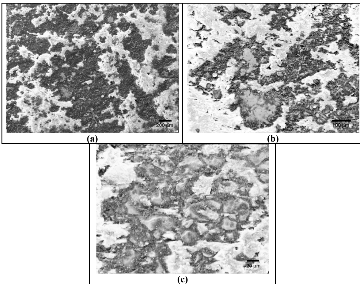
Figure 46. Hollow stainless steel samples: (a) view at the surface, 100×; (b) same region, 300×; and (c) detail of the surface condition, 1,000×. The surface appears rough, but no signs of corrosion damage were observed.
