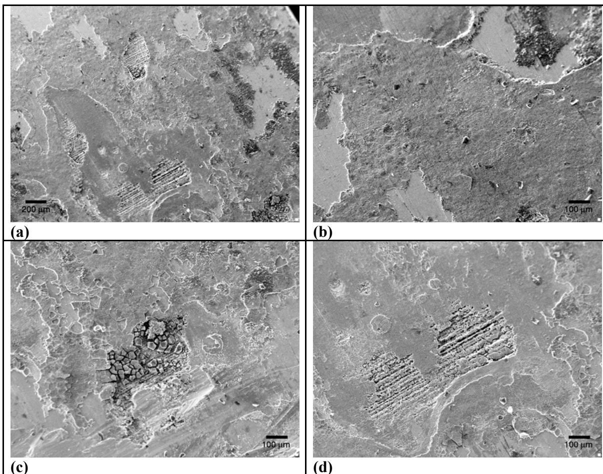
Figure 45. Microcomposite steel samples: (a) aspect of corrosion along at the surface, 100×; (b) same region, 205×; (c) and (d) details of characteristic corrosion sites, 205×.
