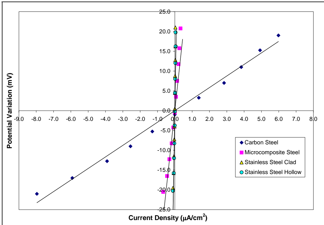
Figure 33. Summary plot showing the variation of potential and current density about the half-cell potential, for different dowels.
