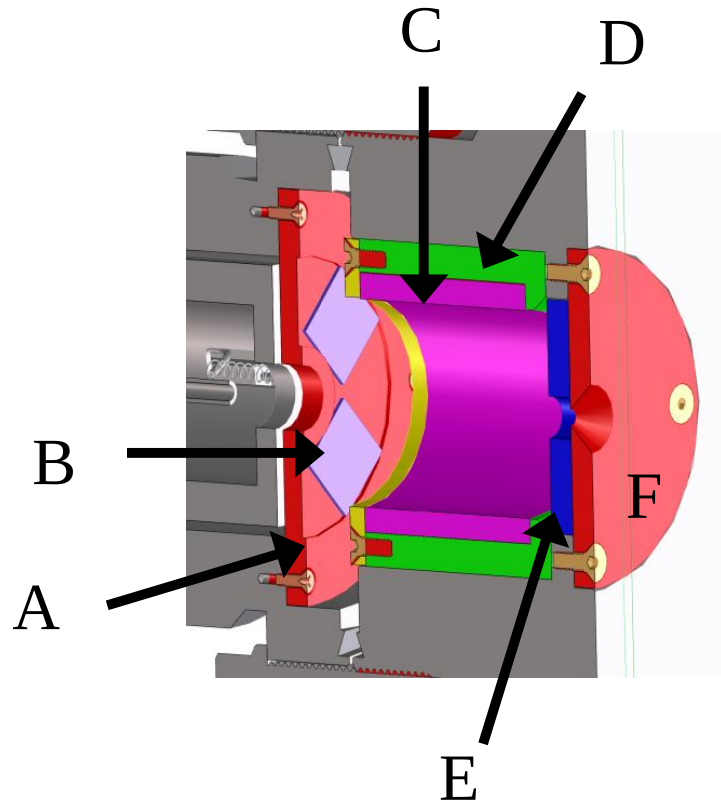
A–Backplate cathode D–Insulator B–Field emitter array E–Cathode shield C–Anode F–Extraction aperture
