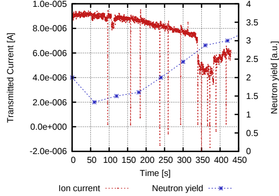
Figure 3.31: Time dependent behavior of ion transmission with corresponding time-averaged neutron yield. The 40 keV, 20 \mu A D_2^+ ion beam is transmitted through a tapered Pyrex tube with taper angle of 16 mrad. The decreasing transmitted ion current may be due to inadequate suppression of electrons, as the increasing neutron yield is consistent with a transmission efficiency of 50%.
