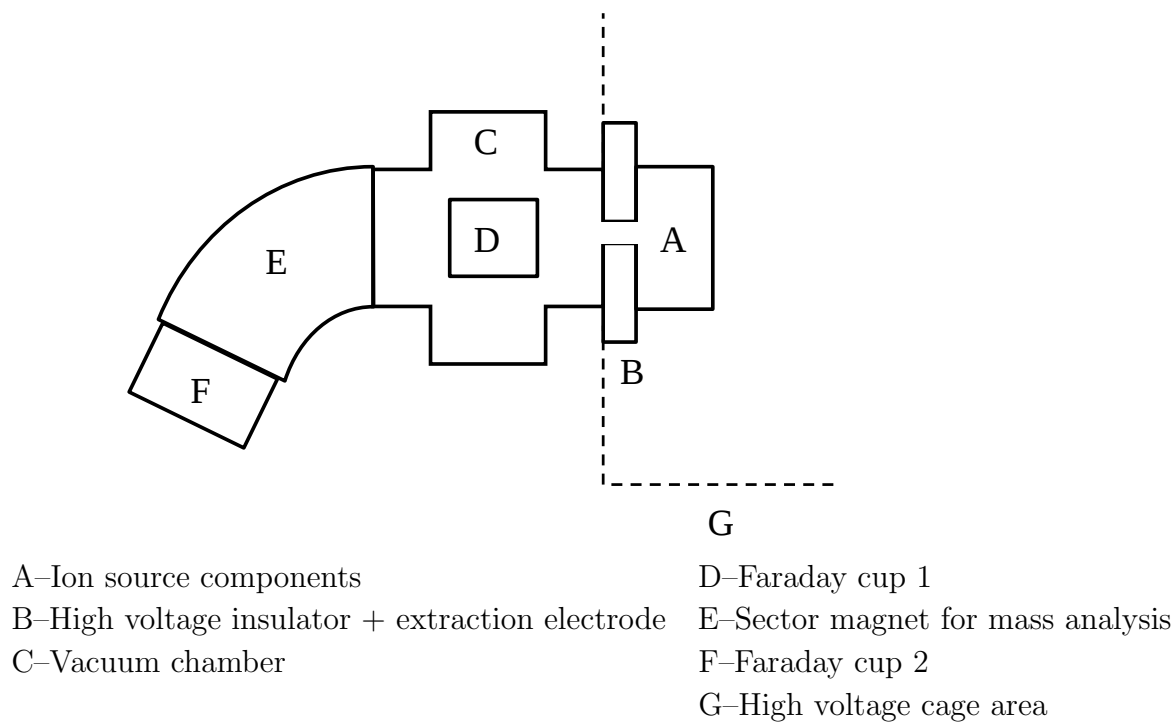
Figure 2.5: Schematic of experimental test stand apparatus. Faraday cup 1 is retractable and can be moved out of the line of sight of the extracted ion beam.
