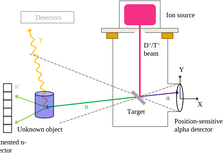
Figure 1.1: Schematic of the API method. Here, D-T fusion reactions at the target create a neutron and associated alpha particle that is detected at the position-sensitive alpha detector. The neutron interacts with a nucleus in the object of interest, emitting a gamma ray that is detected at the external detector array. The dashed lines indicate the spatial extent of the accepted alpha particle trajectories and the resultant extent of the interrogation space. For fissionable materials, the neutron may also induce fission events resulting in neutron multiplicity events; the additional neutrons are detected with segmented neutron detectors.
