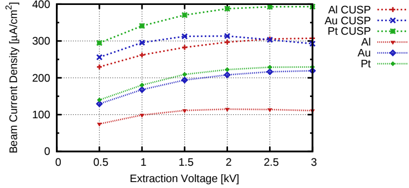
Figure 2.27: Comparison of extracted ion current densities for BLP discharges combining multi-cusp magnetic confinement with various electrode materials.
