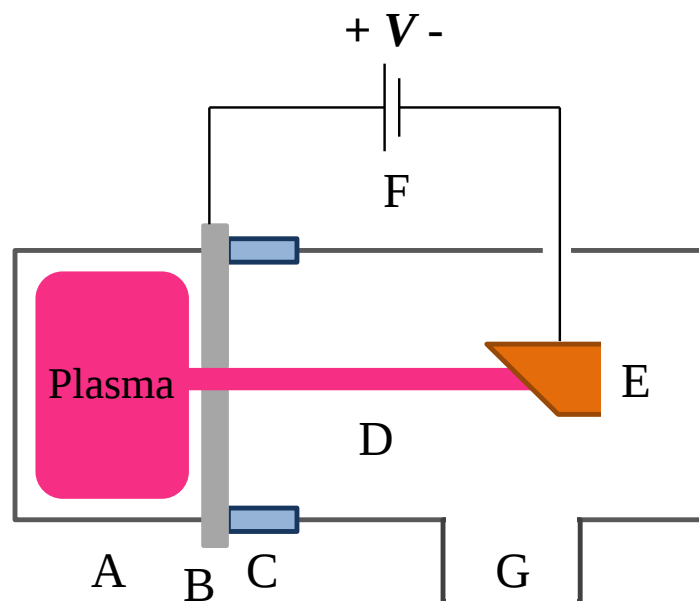
A–Ion source B–Plasma electrode C–High voltage insulator D–Ion beam E–Neutron production target F–Applied high voltage G–Port for pumping, etc.
