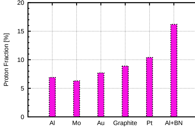
Figure 2.12: Proton fraction in extracted ion beams from hydrogen discharges for BLP source operation with various electrode materials. The plasma interactions with boron nitride result in a factor of two increase in the proton fraction over basic BLP source operation.
