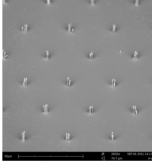
Figure 2.14: SEM image of carbon nanofiber array [43].
