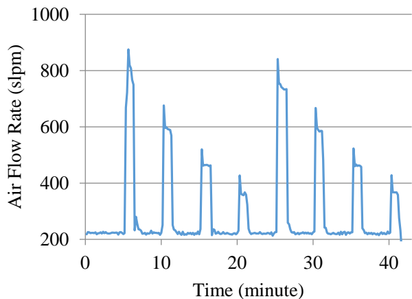
Figure 8. The cathode air flow rate during the series of step load changes.
