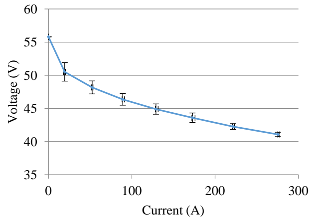
Figure 2. Stack I-V polarization curve of the 12kW in-rack PEMFC system. Error bars in the data indicate \pm one standard deviation from 5 different measurements.
