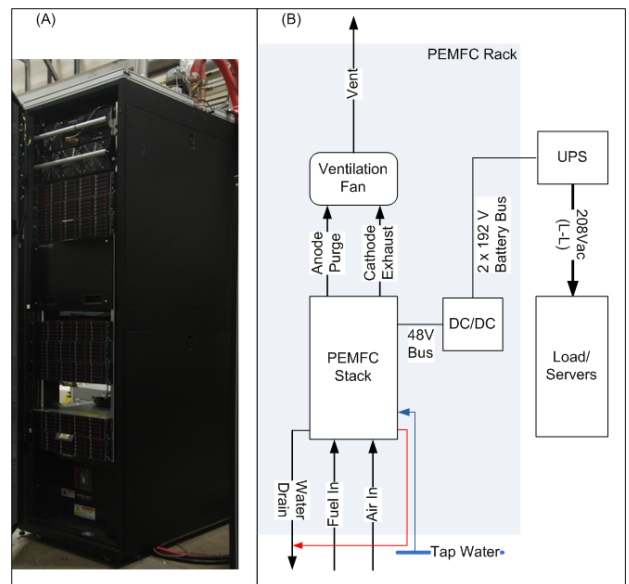
Figure 1. (A) 10kW in-rack PEMFC system and (B) System schematic.
