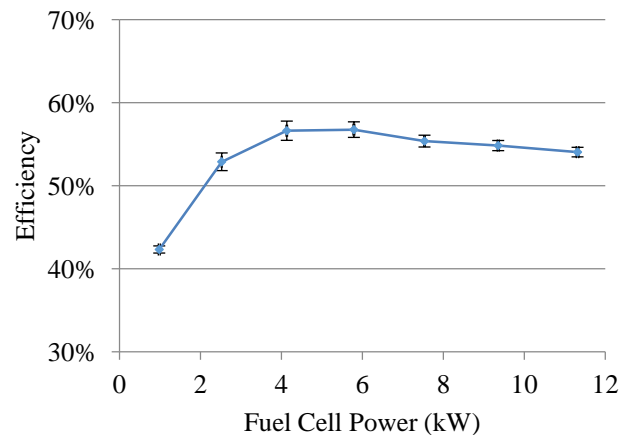
Figure 3. The efficiency curve of the 12kW in-rack PEMFC system. Error bars in the data indicate \pm one standard deviation from 5 different measurements.
