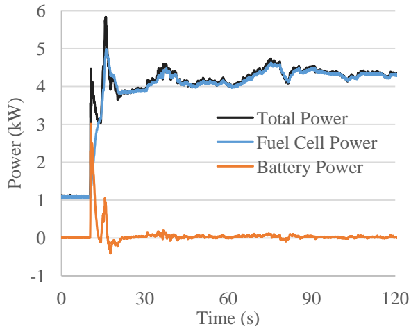
Figure 10. The hybrid system transient responses to server dynamic operation, 9 servers were turned on at t=10 .
