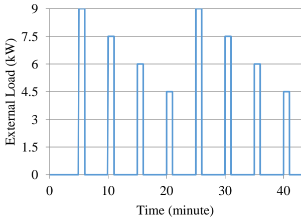
Figure 6. Power profile of the external load with a series of step changes.
