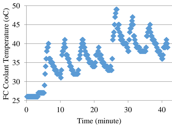
Figure 7. The fuel cell coolant temperature profile during the series of step load changes.
