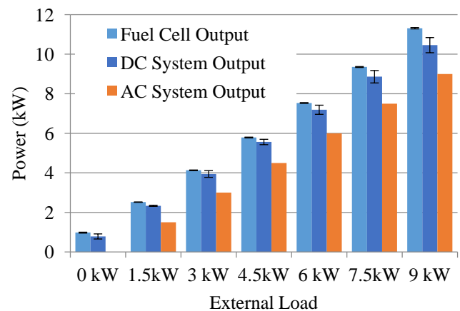
Figure 11. The power outputs of the 12kW in-rack PEMFC system under various external loads. Error bars in the data indicate \pm one standard deviation from 5 different measurements.
