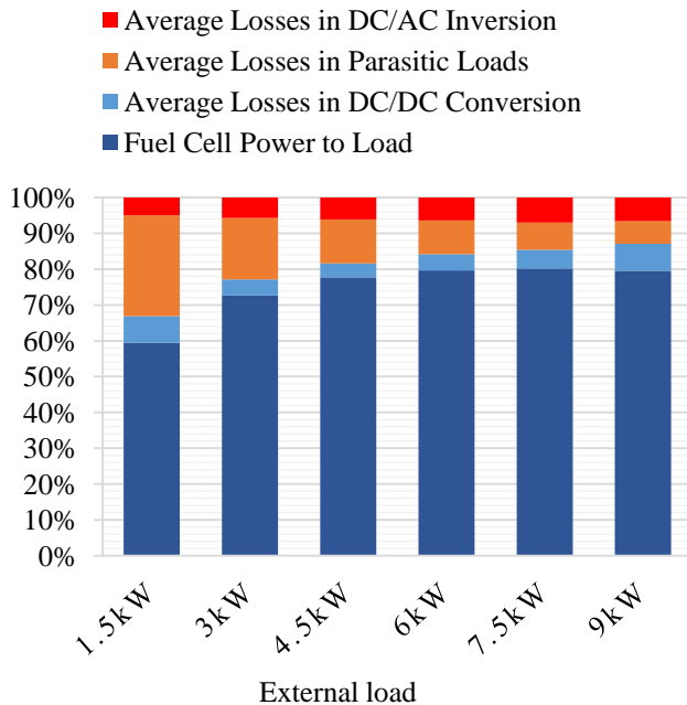
Figure 12. The percentage of power losses of the 12kW in-rack PEMFC system under various external loads.
