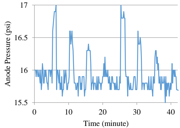
Figure 9. The anode pressure during the series of step load changes.
