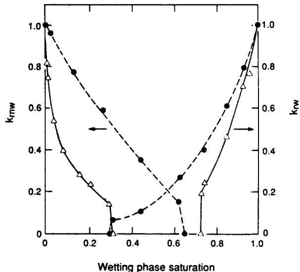
Figure 5. Simulated relative permeabilities for flow in the x-direction (dashed line) and y-direction (solid line) (see Fig. 3).
