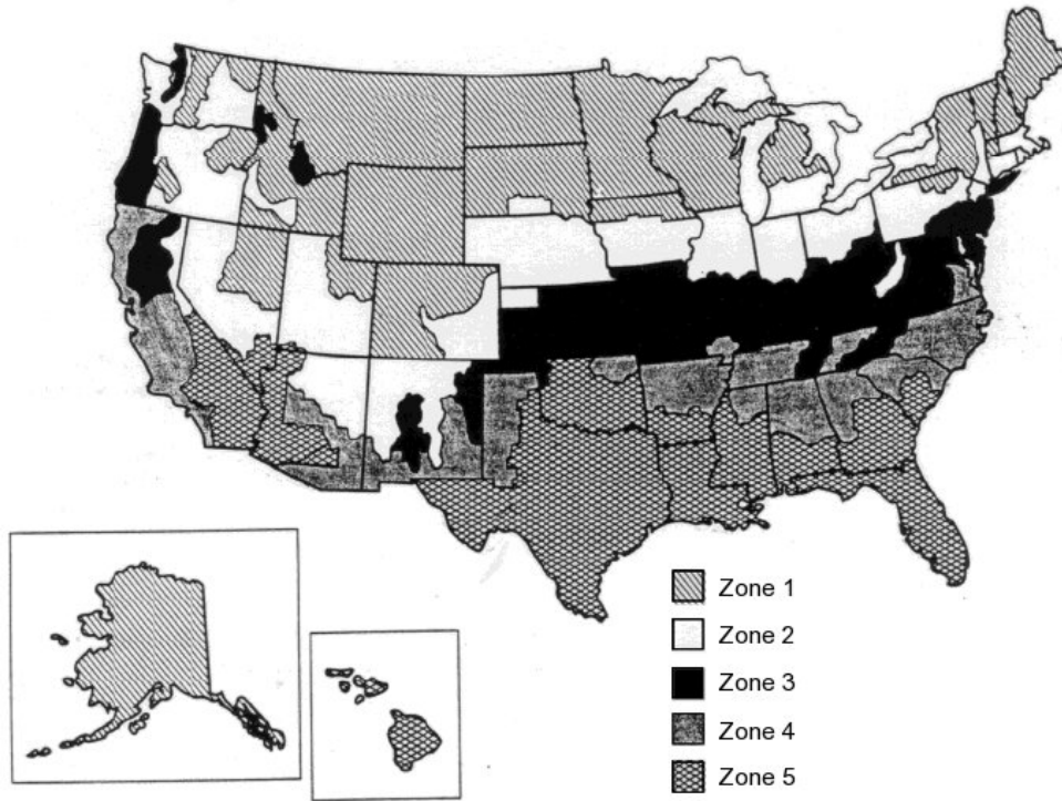
Figure 5 – CBECS Climate Zones for DOE-2 Simulation of Prototypical Commercial Buildings
