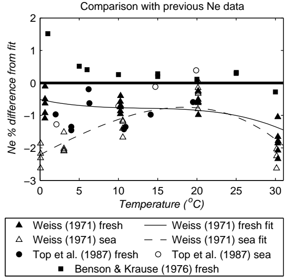
Figure 5: Each symbol shows the percent difference between Ne solubility data from the literature and our proposed solubility curve at the actual temperature and salinity of each data point (heavy center line at 0%). Fresh (filled symbols) indicates data from distilled water, while sea (open symbols) indicates data from experiments with salinity > 25 (PSS). The differences between the fits proposed by Weiss (1971b) and this study are also shown for salinities of 0 and 35.
