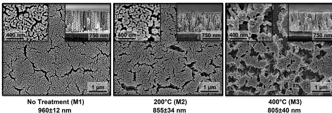
Fig. 2 Scanning electron microscope images of top (main), magnified top (left inset), and cross-sectional (right inset) views of np-Au films treated at different temperatures to obtain various morphologies. Corresponding film thicknesses are included below the images.
