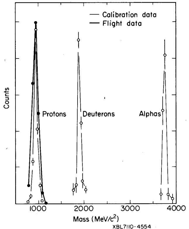
Fig. 2. Mass resolution of the particle identifier used in the high-altitude rocket experiments.
