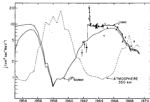
Fig. 1. Computed proton flux j(t)_{60 \text{ MeV}} at h_{\text{min}} = 350 km, beginning 1953.0, assuming source S_{\text{obs}} is constant, and initial flux values j(1953) = 9.2 and 3.2 \text{ cm}^{-2} \text{ sec}^{-1} \text{ MeV}^{-1} . Unique solution is obtained at this altitude after 1958.5. The Starfish redistribution on 9 July 1962, the 3-yr "steady-state" from 1963 to 1966, and the abrupt solar-cycle decrease in the proton flux after mid-1966 are reproduced in these calculations. The data denoted by open circles are from work by Filz and Holeman; the x's, this experiment. The data points are limited to h_{\text{min}} = 350 \pm 50 km. Solar-cycle behavior of atmosphere at 350 km altitude is given by the dashed curve. (XBL-6910-5954)
