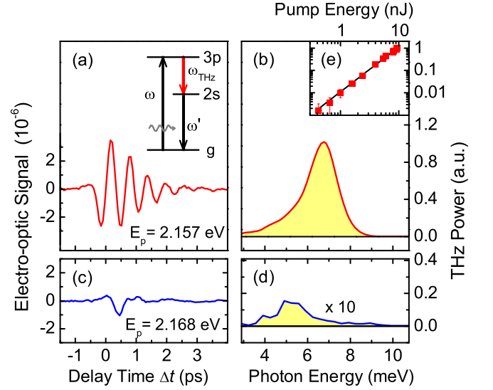
FIG. 4: (color online). THz generation in \text{Cu}_2\text{O} : (a) Real time trace and (b) normalized power spectrum of THz pulses (FWHM: 1.7 meV) obtained with the pump centered at 2.157 eV (close to the 3p resonance). The spectral width of the pump pulse is 12 meV (FWHM). Inset: term scheme of the underlying quantum process. (c), (d) THz emission for pump centered at 2.168 eV. (e) The emitted THz power for excitation at 2.157 eV scales quadratically as a function of the pump pulse energy.
