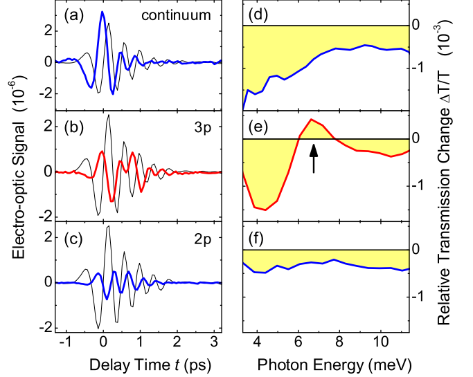
FIG. 2: (color online). (a)-(c) Pump-induced changes \Delta E_{\text{THz}} (thick lines) at \Delta t = 1 ps after excitation, and reference THz fields E_{\text{THz}} (thin lines) without excitation. The reference fields are downscaled by a factor of 500 for better visibility. Pump spectra are centered (a) in the continuum at 2.206 eV, (b) at the yellow 3p exciton line, and (c) at the 2p exciton line. (d)-(f) Corresponding relative transmission changes \Delta T/T . Arrow: enhanced transmission at 6.6 meV.
