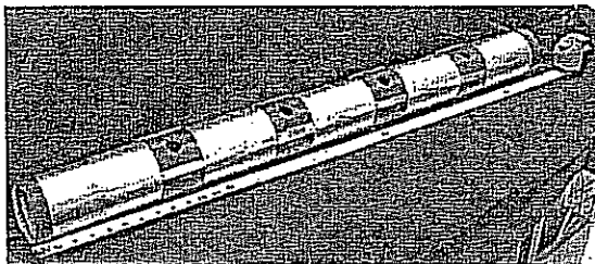
Figure 2 The one-meter-long BaTiO 3 FEPS consists of 5 individual sources with diagnostic ports between the sources.
