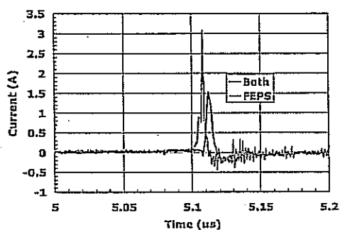
Figure 3: Time trace of the longitudinally compressed ion beam with charge neutralization with the FEPS and with both plasma sources.
