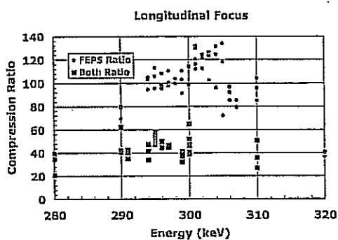
Figure 4: Longitudinal compression using the FEPS for charge neutralization yields a 120 compression.
