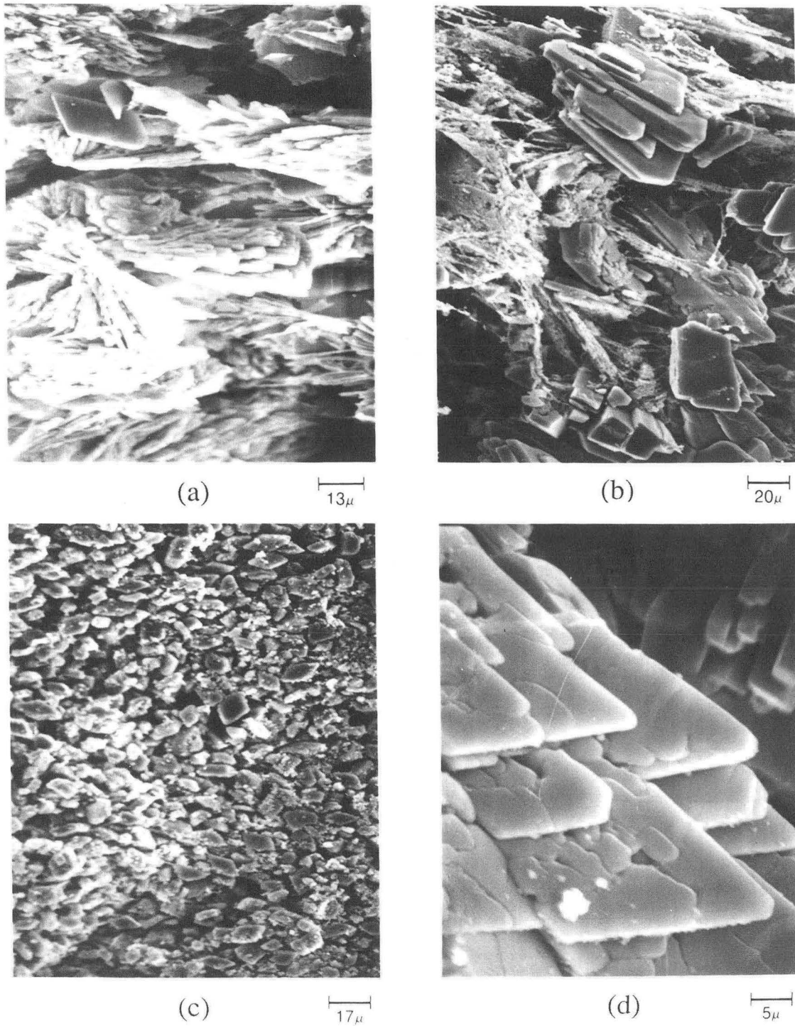
Figure 38. Morphology of area 3 in zinc electrodes with \text{Ca}(\text{OH})_2 . (a, c & d) Calcium zincate crystals are found everywhere with very little powder present. (b) PTFE filaments can be seen binding the crystals together.
