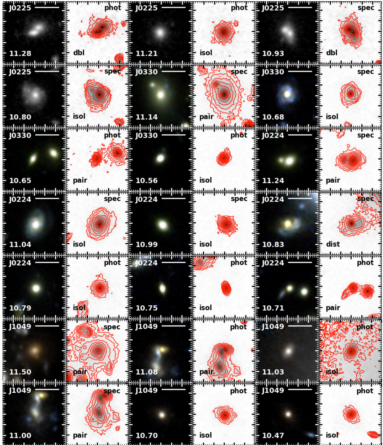
FIG. 2.— Simplified 6'' \times 6'' stamps of a subset of cluster members. The left panels show the cluster name in the top left, a horizontal bar indicating a distance of 20 kpc physical at the cluster redshift, and the log stellar mass in the lower left. The left images show grayscale F160W stamps for J0225, three-filter RGB (F105W, F140W, F160W) for clusters J0330 and J0224, and two-filter RGB in (F105W, F105W+F160W, F160W) for J1049. The right panels for all objects show grayscale F160W images with surface brightness contours starting at 24.5 \text{ mag arcsec}^{-2} and increasing by 0.5 \text{ mag arcsec}^{-2} . The text in the upper right indicates whether the object was spectroscopically or photometrically selected, and the label in the lower left indicates the classification (isolated, pair, disturbed, or double nucleus).
