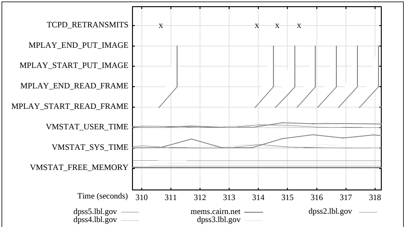
Figure 7: NetLogger real time analysis of JAMM managed Sensor data
