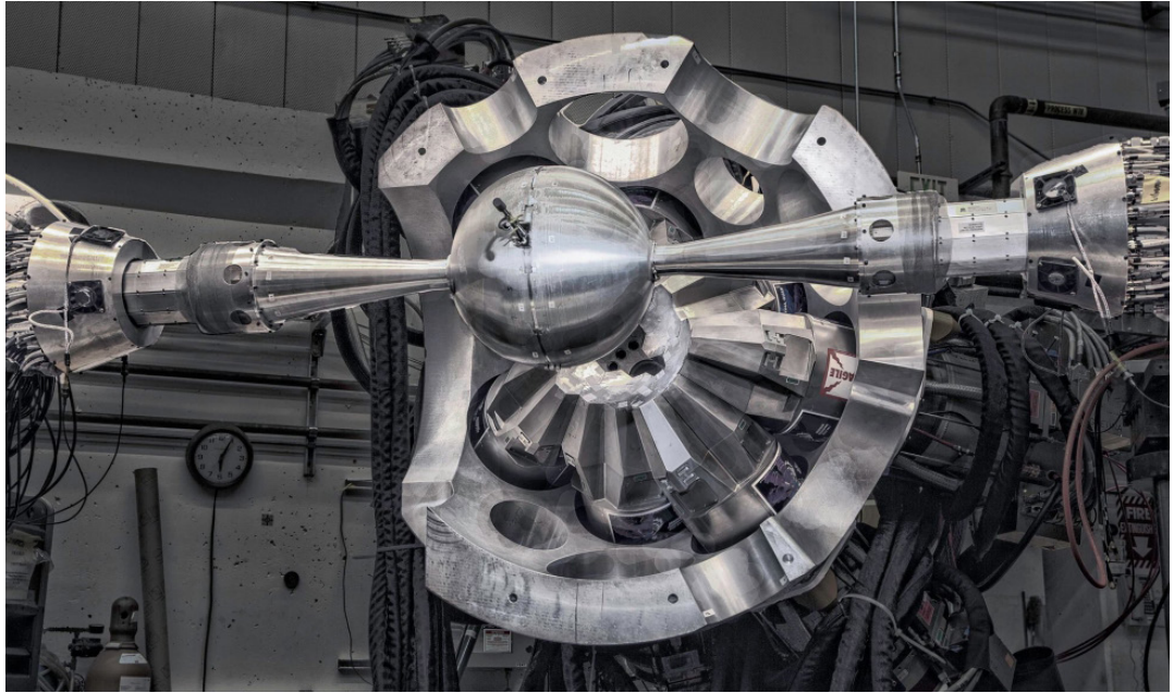
Figure 3-10. GREINA is the predecessor for the GRETA gamma-ray tracking detector array. The construction of GRETA, a full 4\pi coverage device, with increased rate requirements, coupled with the need for real-time processing, requires significant I/O, CPU, memory, and storage resources. (Image by Kevin Bailey of Argonne National Laboratory; reproduced with permission from Shaofei Zhu.)
