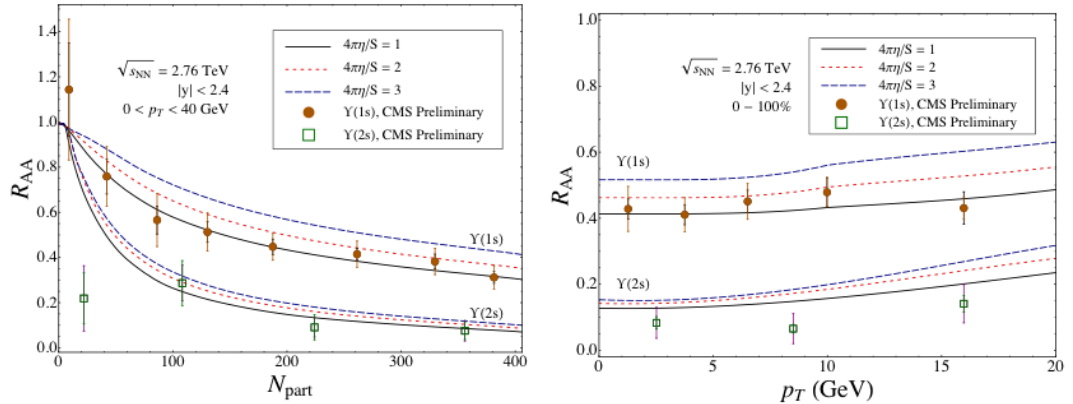
Figure 3-42. Nuclear suppression factor R_{AA} for the Y(1s) and Y(2s) bottomonia states as a function of the number of nucleons participating in the heavy ion collision ( N_{part} ) (left) and particle transverse momentum ( p_T ) (right). Data are provided by the CMS and ALICE collaborations (CMS Collaboration 2015; Abelev et al. 2014). The curves are the predictions of a theoretical model that uses viscous anisotropic hydrodynamics to model the QGP evolution and takes into account the in-medium QGP decay width of the various Y states (Krouppa et al. 2015). The level of Y -suppression seen is much larger than that which would be generated by cold nuclear matter effects. This observation can be seen as an indication of QGP-induced suppression of bottomonia.
