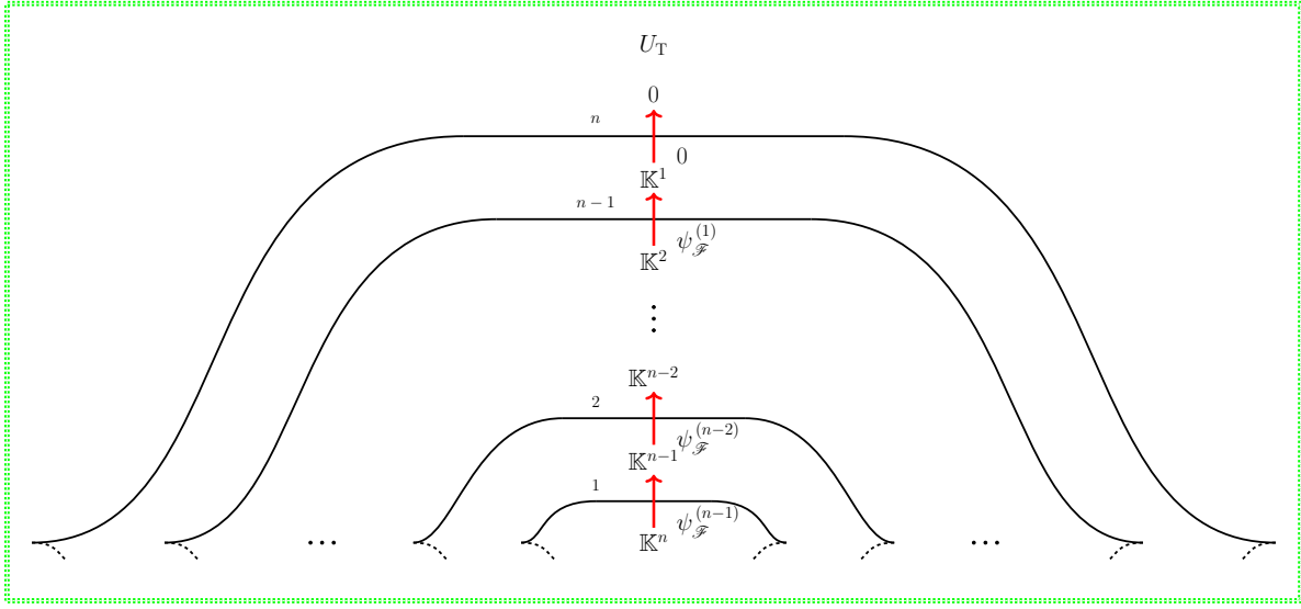
FIGURE 3.9. An object \mathcal{F} of the cohomological category H^\bullet(\mathcal{S}h_1(\Lambda(\beta), \mathbb{K})_0) on the region U_T .
