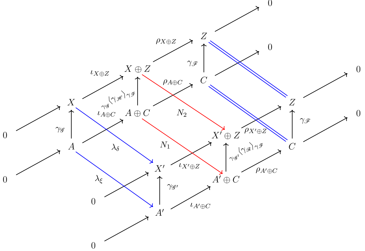
FIGURE 4.16. Commutative diagram between the block extensions \gamma_{\mathcal{G}} \langle \gamma_{\mathcal{H}} \rangle_{\gamma_{\mathcal{F}}} and \gamma_{\mathcal{G}'} \langle \gamma_{\mathcal{D}} \rangle_{\gamma_{\mathcal{F}}} .
