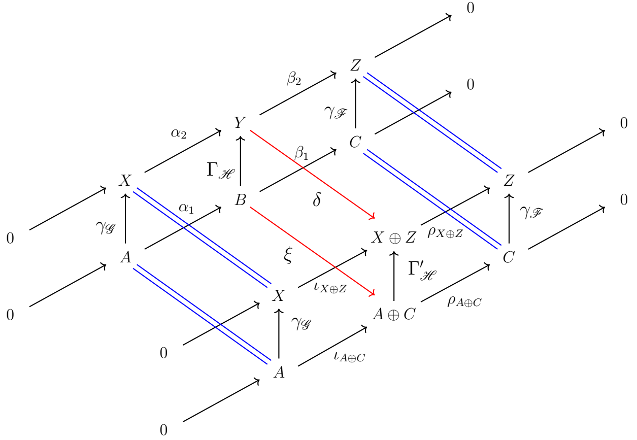
FIGURE 4.9. Two equivalent extensions \Gamma_{\mathcal{H}} and \Gamma'_{\mathcal{H}} of \gamma_{\mathcal{F}} by \gamma_{\mathcal{G}} .
