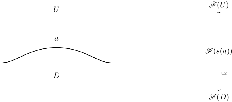
(a) Strata configuration near an arc.
