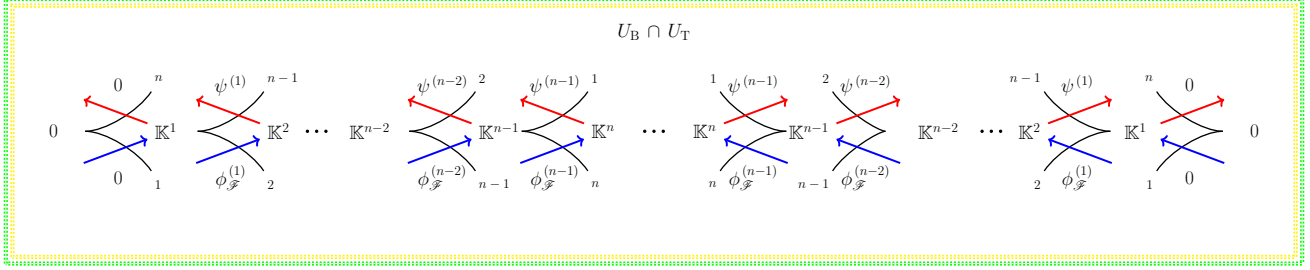
FIGURE 3.5. An object \mathcal{F} of the category H^\bullet(Sh_1(\Lambda(e_n), \mathbb{K})_0) on the intersection U_B \cap U_T .
