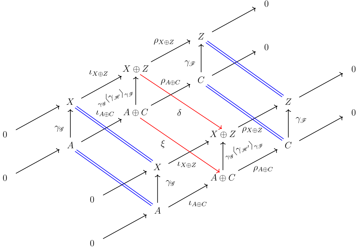
FIGURE 4.10. Two equivalent extensions \gamma_{\mathcal{G}} \langle \gamma_{\mathcal{H}} \rangle_{\gamma_{\mathcal{F}}} and \gamma_{\mathcal{G}} \langle \gamma_{\mathcal{H}'} \rangle_{\gamma_{\mathcal{F}}} of \gamma_{\mathcal{F}} by \gamma_{\mathcal{G}} .
