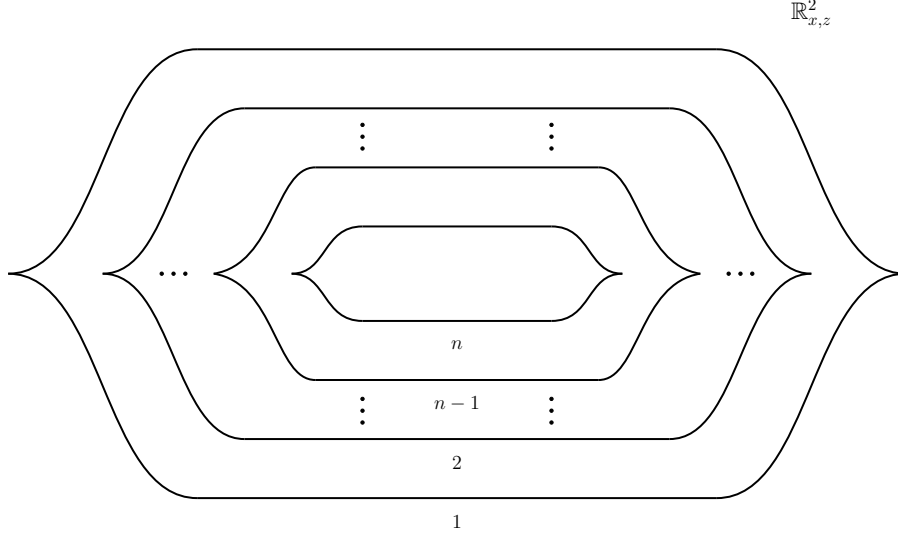
FIGURE 2.1. Front projection \Pi_{x,z}(\Lambda(e_n)) \subset \mathbb{R}^2 of the Legendrian unlink \Lambda(e_n) \subset (\mathbb{R}^3, \xi_{\text{std}}) on n strands.
