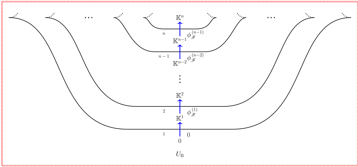
FIGURE 3.4. An object \mathcal{F} of the category H^\bullet(\mathcal{S}h_1(\Lambda(e_n), \mathbb{K})_0) on the region U_B .
