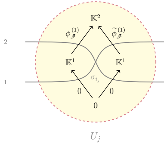
FIGURE 3.16. Commutative diagram for the linear maps defining a sheaf \mathcal{F} on the region U_j in the case k = i_j = 1 .
