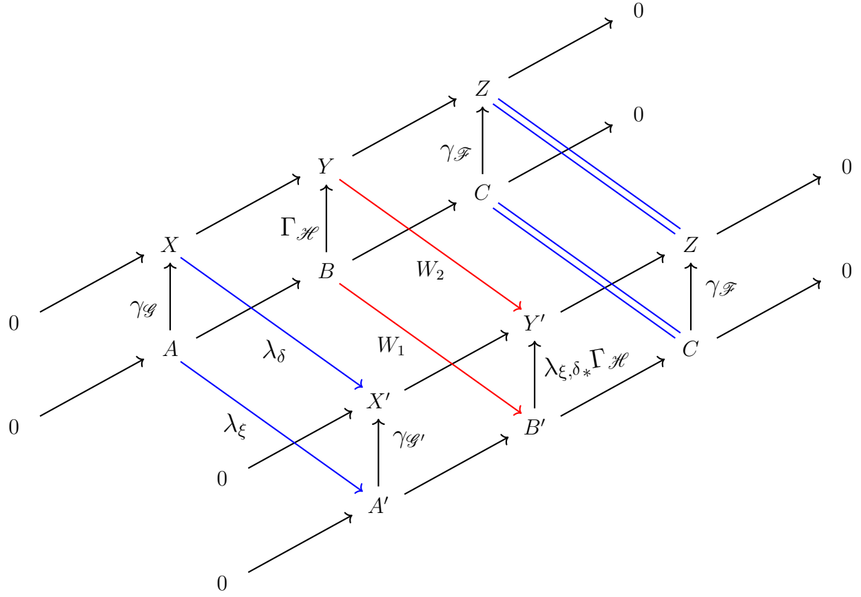
FIGURE 4.14. The push-out \lambda_{\xi,\delta*}\Gamma_{\mathcal{H}} of the extension \Gamma_{\mathcal{H}} of \gamma_{\mathcal{F}} by \gamma_{\mathcal{G}} via the morphism \lambda_{\xi,\delta} between \gamma_{\mathcal{G}} and \gamma_{\mathcal{G}'} .
