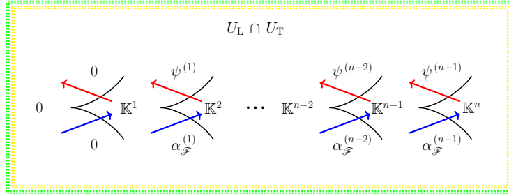
FIGURE 3.10. An object \mathcal{F} of the cohomological category H^\bullet(\mathcal{S}h_1(\Lambda(\beta), \mathbb{K})_0) on the intersection U_L \cap U_T .
