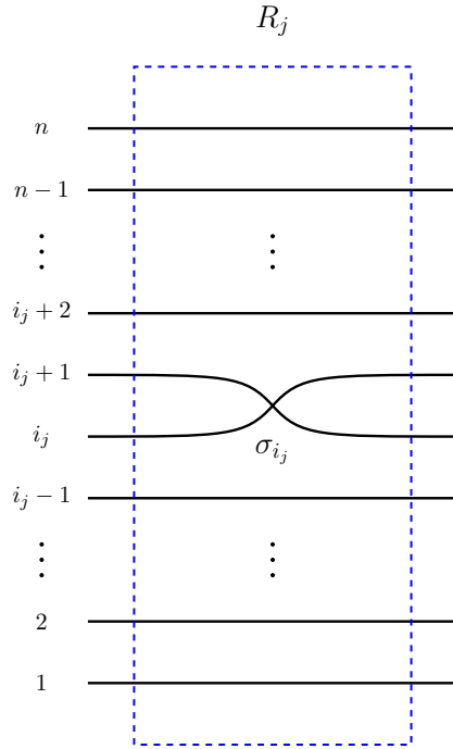
FIGURE 3.13. Intersection of an open vertical strap R_j in \mathbb{R}^2 with the front projection \Pi_{x,z}(\Lambda(\beta)) \subset \mathbb{R}^2 .
