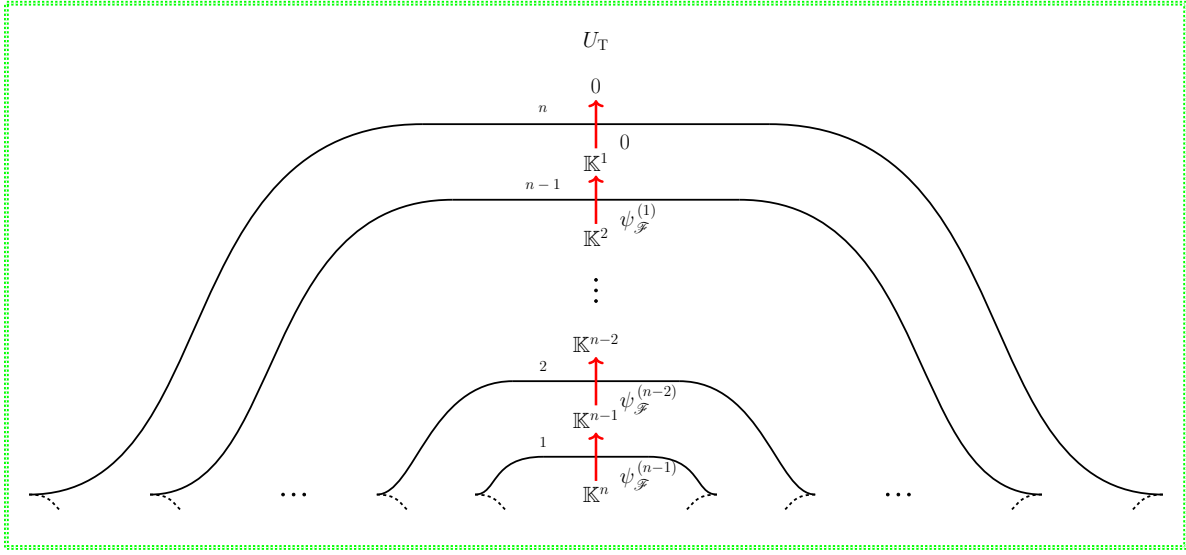
FIGURE 3.3. An object \mathcal{F} of the category H^\bullet(\mathcal{S}h_1(\Lambda(e_n), \mathbb{K})_0) on the region U_T .
