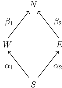
FIGURE 3.1. Commutative diagram for a collection of linear maps \alpha_1 , \beta_1 , \alpha_2 , and \beta_2 satisfying the crossing condition.
