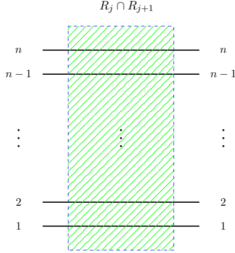
FIGURE 3.14. Intersection of the overlap R_j \cap R_{j+1} of two adjacent straps R_j and R_{j+1} in \mathbb{R}^2 with the front projection \Pi_{x,z}(\Lambda(\beta)) \subset \mathbb{R}^2 .
