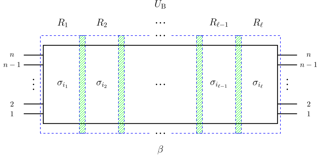
FIGURE 3.12. Region U_B in \mathbb{R}^2 decomposed into a collection \mathcal{R}_{\Lambda(\beta)} := \{R_i\}_{i=1}^{\ell} of \ell open vertical straps R_j in \mathbb{R}^2 .
