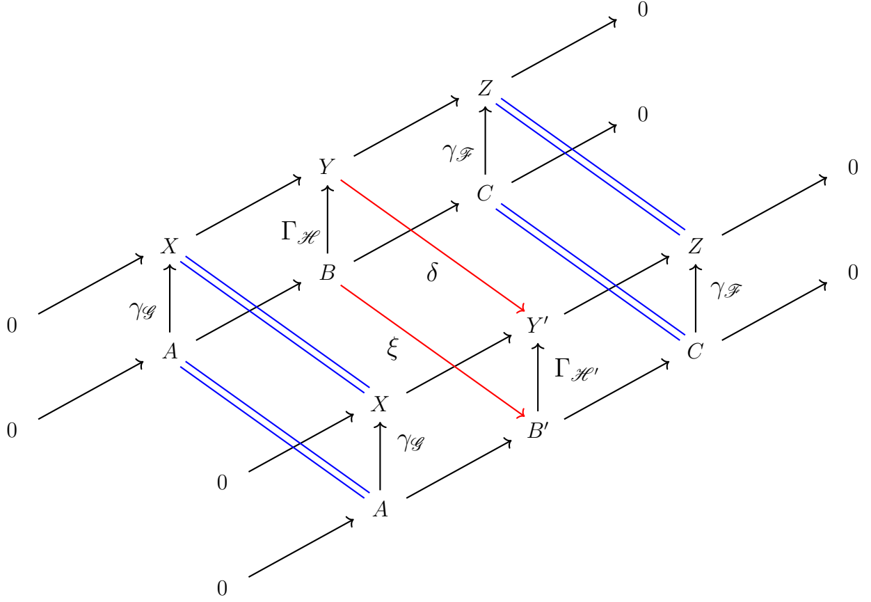
FIGURE 4.4. Two equivalent extensions \Gamma_{\mathcal{H}} and \Gamma_{\mathcal{H}'} of \gamma_{\mathcal{F}} by \gamma_{\mathcal{G}} .
