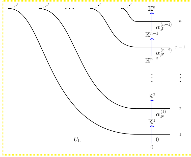
FIGURE 3.7. An object \mathcal{F} of the cohomological category H^\bullet(Sh_1(\Lambda(\beta), \mathbb{K})_0) on the region U_L .
