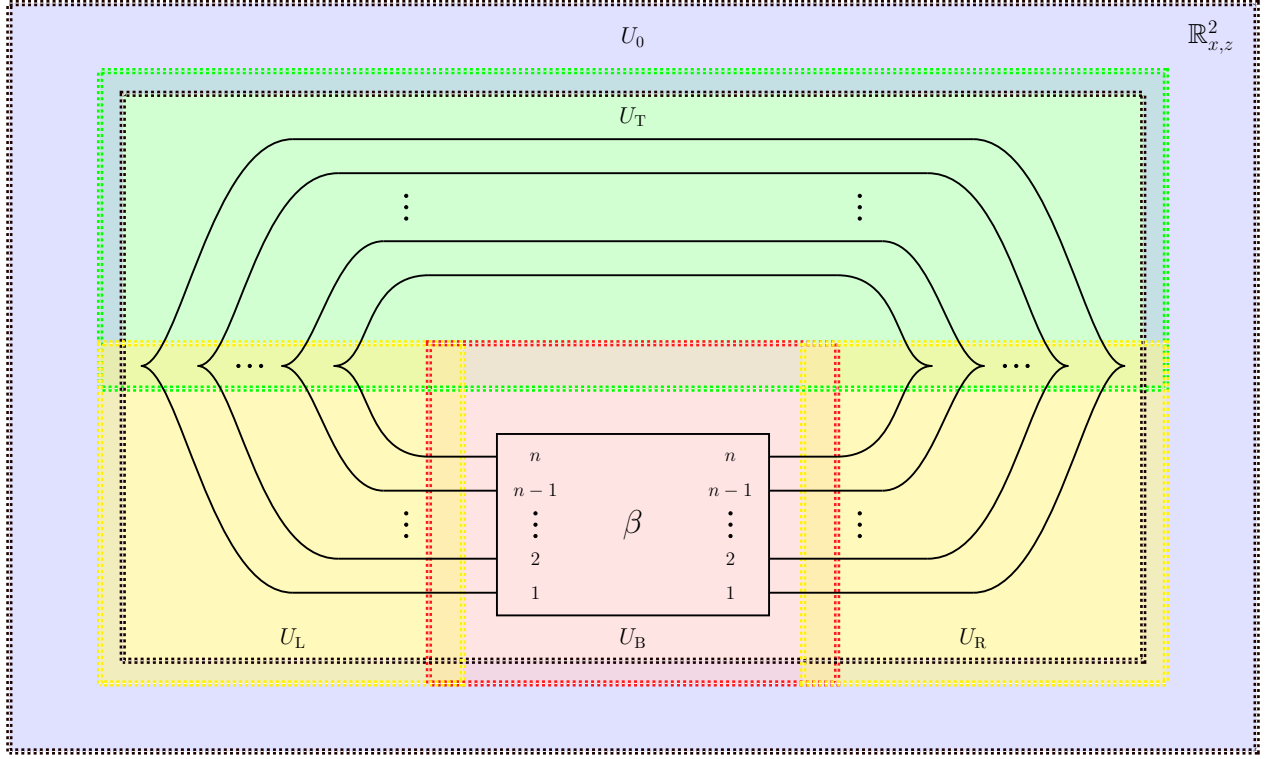
FIGURE 3.6. The front projection \Pi_{x,z}(\Lambda(\beta)) \subset \mathbb{R}^2 of the Legendrian link \Lambda(\beta) \subset (\mathbb{R}^3, \xi_{\text{std}}) , along with the finite open cover \mathcal{U}_{\Lambda(\beta)} = \{U_0, U_B, U_L, U_R, U_T\} of \mathbb{R}^2 . The regions U_L and U_R are shown in yellow, while U_0 , U_B , and U_T are depicted in purple, pink, and green, respectively.
