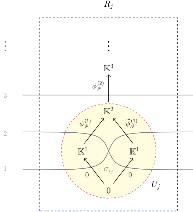
FIGURE 3.15. An object \mathcal{F} on the vertical strap R_j containing a crossing \sigma_{i_j} in the case k = i_j = 1 .
