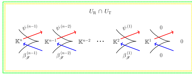
FIGURE 3.11. An object \mathcal{F} of the cohomological category H^\bullet(\mathcal{S}h_1(\Lambda(\beta), \mathbb{K})_0) on the intersection U_R \cap U_T .
