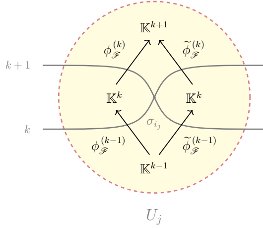
FIGURE 3.18. Commutative diagram for the linear maps that define a sheaf \mathcal{F} on the region U_j in the case k = i_j \geq 2 .
