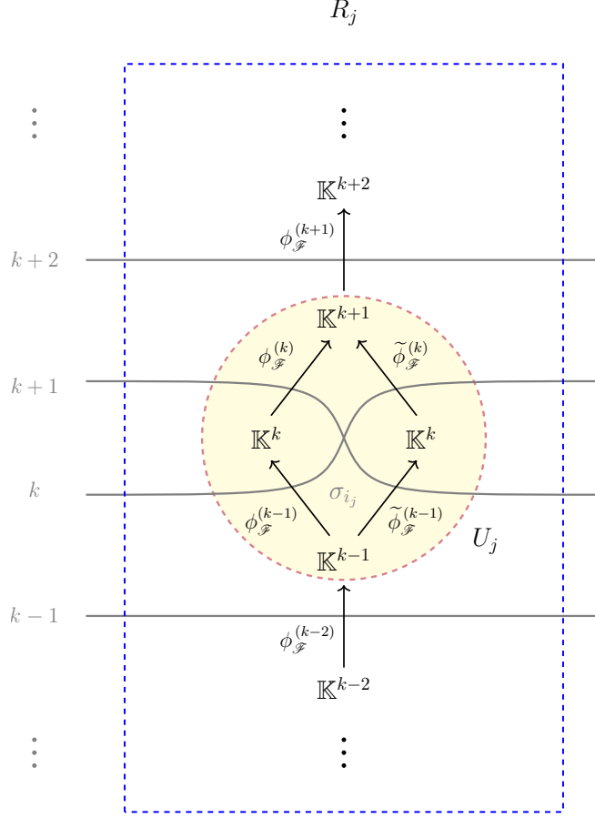
FIGURE 3.17. An object \mathcal{F} on the vertical strap R_j containing the crossing \sigma_{i_j} in the case k = i_j \geq 2 .
