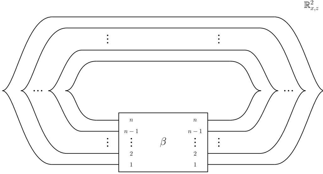
FIGURE 1.1. Front projection \Pi_{x,z}(\Lambda(\beta)) of the Legendrian link \Lambda(\beta) .
