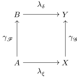
FIGURE 4.1. A morphism \lambda_{\xi, \delta} between \gamma_{\mathcal{F}} by \gamma_{\mathcal{G}} .
