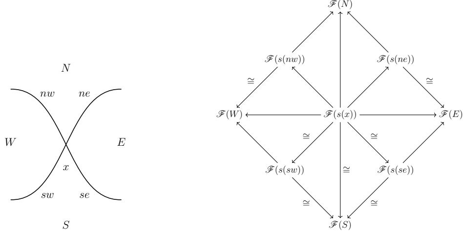
(a) Strata configuration near a crossing. (b) Micro-support condition near a crossing.
