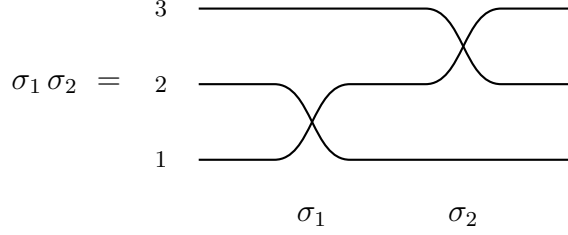
FIGURE 1.2. Braid diagram on three strands of the positive braid word \sigma_1 \sigma_2 \in \text{Br}_3^+ .
