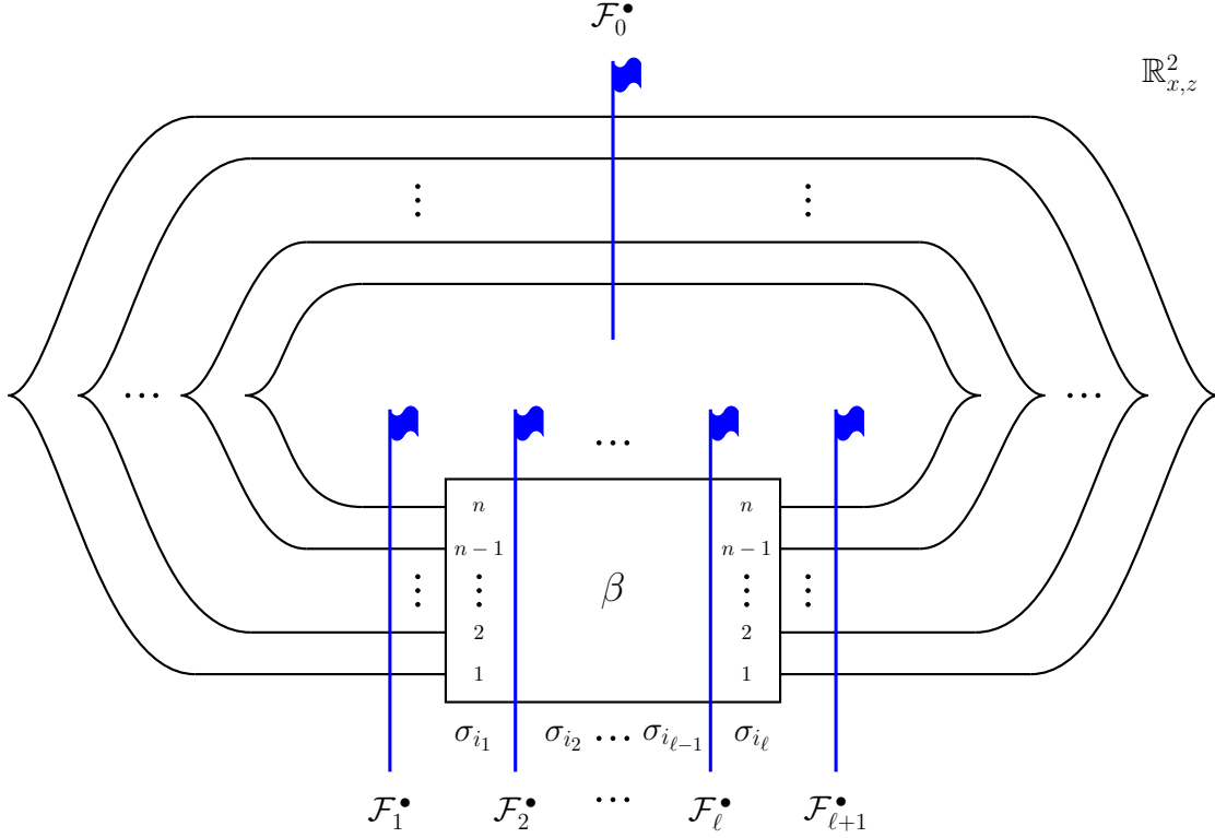
FIGURE 3.19. An object \mathcal{F} of the category H^\bullet(\mathcal{S}h_1(\Lambda(\beta), \mathbb{K})_0) .
