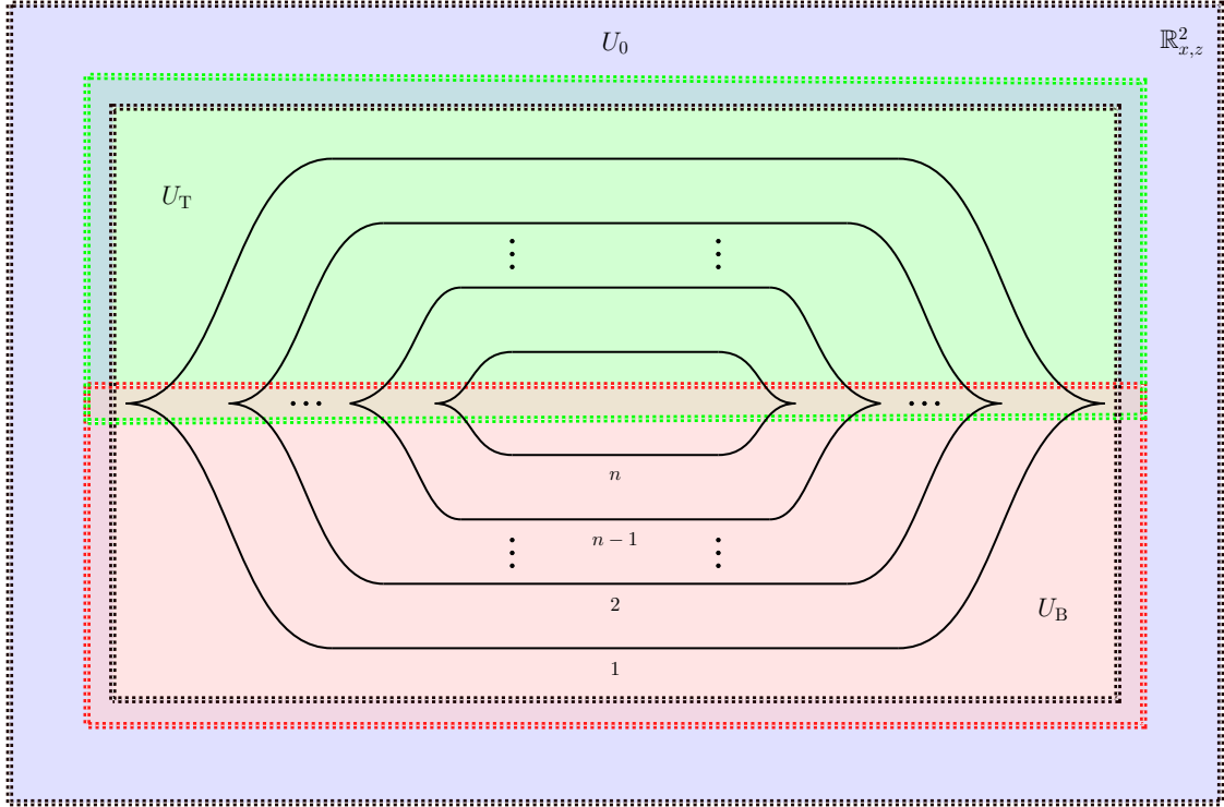
FIGURE 3.2. The front projection \Pi_{x,z}(\Lambda(e_n)) \subset \mathbb{R}^2 of the Legendrian link \Lambda(e_n) \subset (\mathbb{R}^3, \xi_{\text{std}}) , along with the finite open cover \mathcal{U}_{\Lambda(e_n)} = \{U_0, U_B, U_T\} of \mathbb{R}^2 . The regions U_0 , U_B , and U_T are depicted in purple, pink, and green, respectively.
