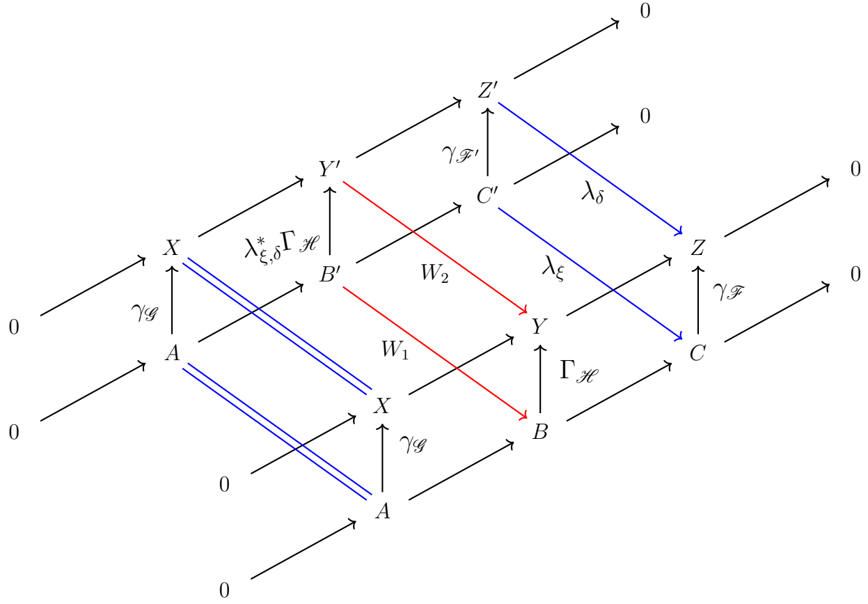
FIGURE 4.13. The pull-back \lambda_{\xi, \delta}^* \Gamma_{\mathcal{H}} of the extension \Gamma_{\mathcal{H}} of \gamma_{\mathcal{F}} by \gamma_{\mathcal{G}} via the morphism \lambda_{\xi, \delta} between \gamma_{\mathcal{F}'} and \gamma_{\mathcal{F}} .
