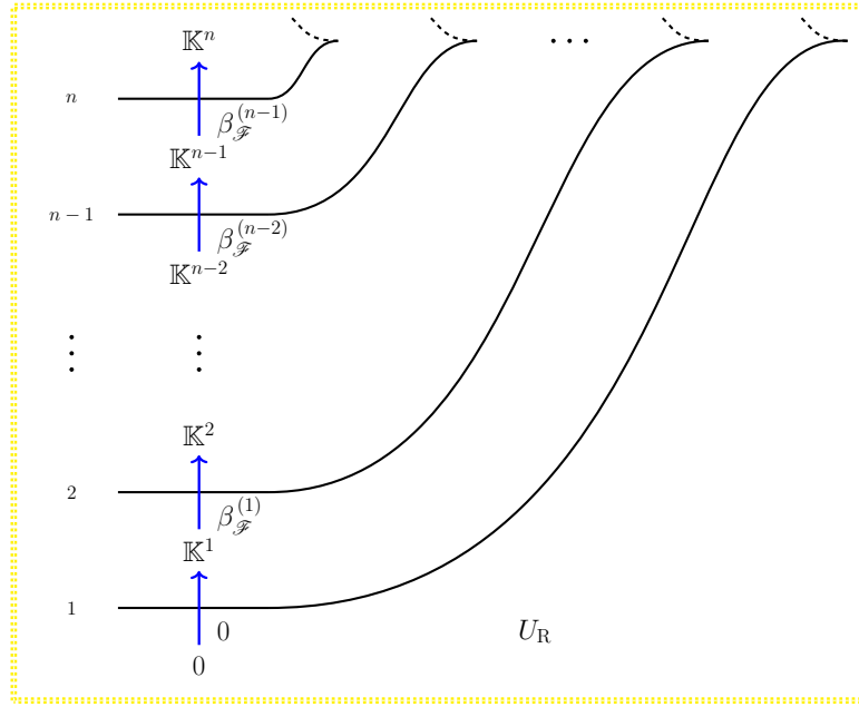
FIGURE 3.8. An object \mathcal{F} of the cohomological category H^\bullet(Sh_1(\Lambda(\beta), \mathbb{K})_0) on the region U_R .
