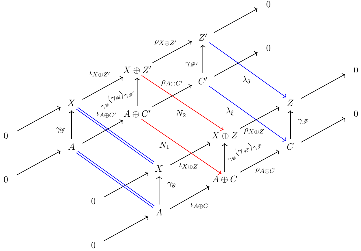
FIGURE 4.15. Commutative diagram between the block extensions \gamma_{\mathcal{G}} \langle \gamma_{\mathcal{R}} \rangle_{\gamma_{\mathcal{F}'}} and \gamma_{\mathcal{G}} \langle \gamma_{\mathcal{H}} \rangle_{\gamma_{\mathcal{F}}} .
