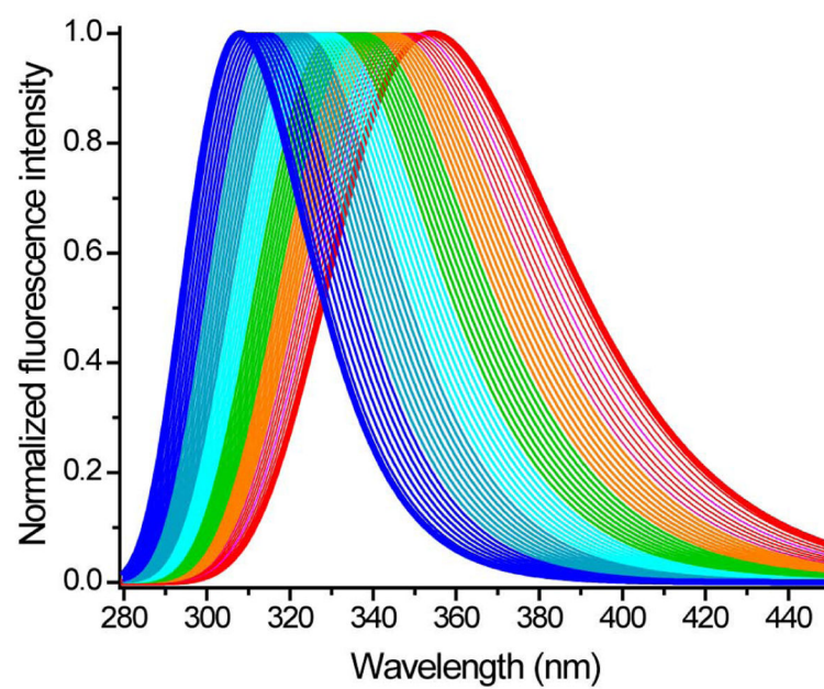
Figure 1. Simulated log-normal fluorescence spectra of Trp with various \lambda_{\text{max}} values. Normalized fluorescence spectra are derived from parameters and the formula described in the experimental methods section. The blue shift decreases the bandwidth of the spectrum.
