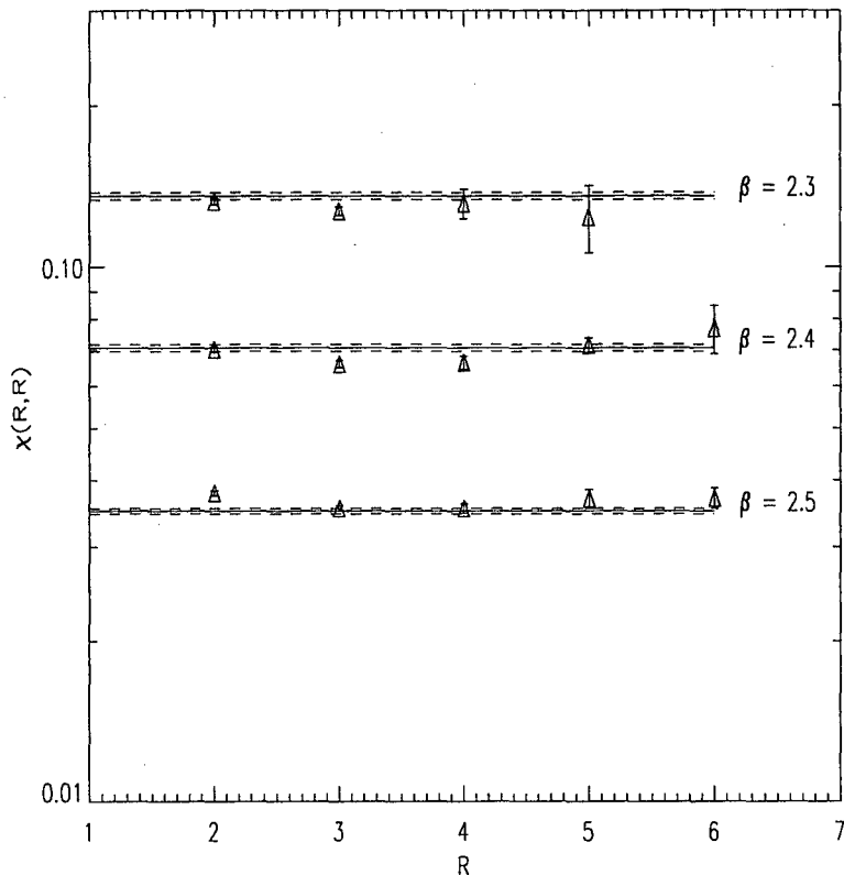
Figure 6: Center-projection Creutz ratios \chi(R, R) vs. R at \beta = 2.3, 2.4, 2.5 . Triangles are our data points. The solid lines show the value (at each \beta ) of the asymptotic string tension of the unprojected configurations, and the dashed lines, above and below each solid line, indicates the associated error bars, quoted in ref. [16].
