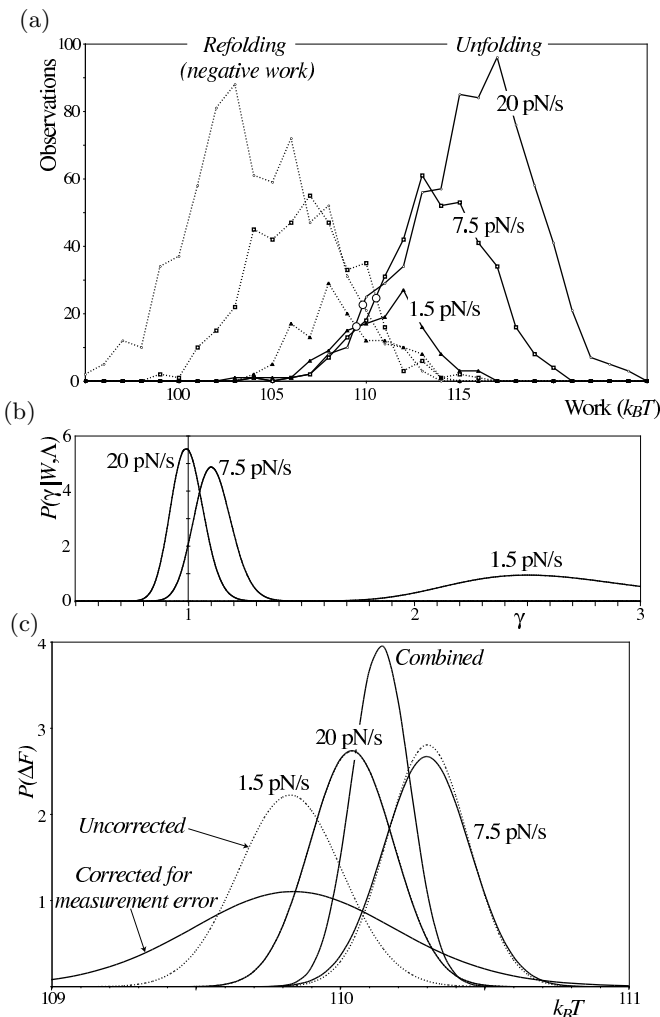
FIG. 5: (a) Histograms of work measurements for folding and unfolding an RNA hairpin at three different rates. Observations are binned into integers centered at 1 \text{ k}_B T intervals. This data corresponds to Fig. 2 of Collin et al. 2 . Note that Eq. (3) predicts that the folding and unfolding work distributions cross at the free energy change. (b) The posterior distribution of the error correction factor \gamma [Eq. (16)]. (c) Posterior free energy derived from the data in (a), both with [Solid line, Eq. (16)] and without [Dashed line, Eq. (11)] correction for measurement noise. Notice that the correction is substantial for the slowest experiment (1.5 pN/s), minor for the intermediate rate, and the corrected and uncorrected posteriors are indistinguishable (at this scale) for the fastest rate. The most reliable free energy estimate is obtained by combining the three separate noise corrected free energy posterior distributions.
