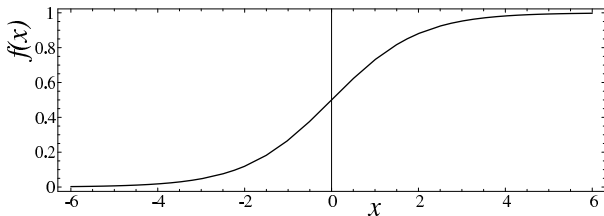
FIG. 3: The standard logistic function, f(x) = 1/(1 + e^{-x}) .
