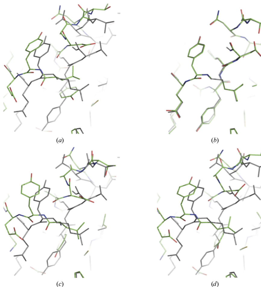
Figure 6 Structures after refinement of a severely distorted model, shown in (a), using different refinement protocols: (b) dual-space refinement, (c) refinement using minimization only and (d) combined refinement using minimization and simulated annealing. The best available refined model is shown in gray in all panels.
