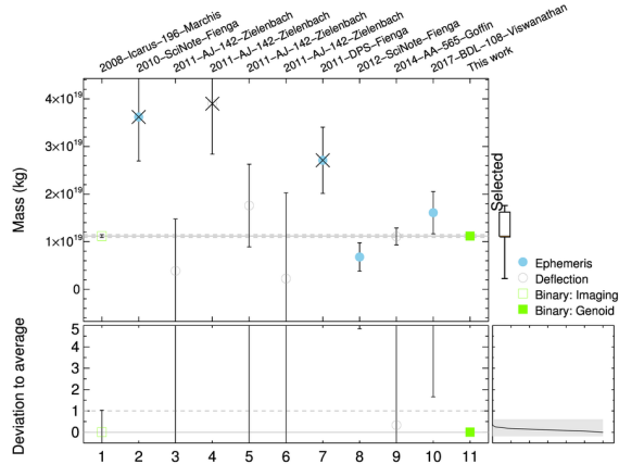
Figure B.1: Mass estimates of (107) Camilla gathered from the literature, see Table B.1 for details.
