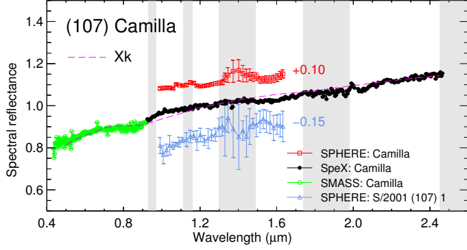
Figure 5: Visible and near-infrared spectrum of Camilla from IRTF (green and black dots) and SPHERE (red squares, offset by +0.1), and its moon S1 from SPHERE (blue triangles, offset by -0.15). Gray areas represent the wavelength ranges affected by water vapour in the atmosphere. All spectra were normalized to unity at one micron. Overplot to the IRTF spectra is the Bus-DeMeo Xk class.
