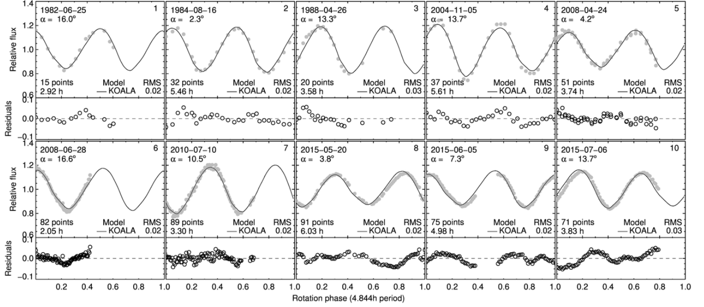
Figure 6: Examples of optical lightcurves of Camilla. For each epoch, the upper panel presents the observed photometry (grey spheres) compared with synthetic lightcurves generated with the shape model (black lines). The lower panel shows the residuals between the observed and synthetic flux. The observing date, number of points, duration of the lightcurve (in hours), phase angle ( \alpha ), and RMS residuals between the observations and the synthetic lightcurves are displayed. In most cases, measurement uncertainties are not provided by the observers but can be estimated from the spread of measurements. See Fig. C.1 for the entire data set.
