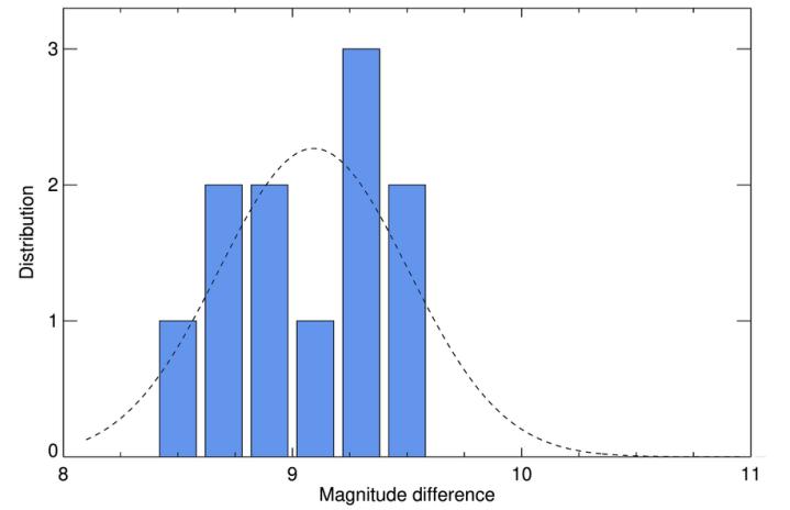
Figure 12: Distribution of the magnitude differences between Camilla and its second satellite S2. The dashed black line represents the normal distribution fit to our results, with a mean and standard deviation of 9.0 \pm 0.3 .
