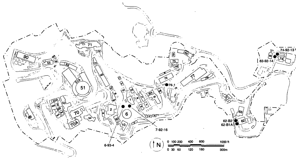
Figure 7-15. Locations of Monitoring Wells Downgradient from Present and Decommissioned Underground Storage Wells
