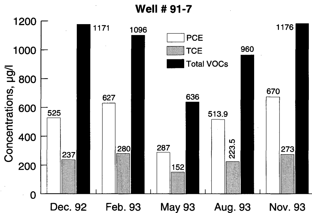
Figure 7-10. Time Variation of Contaminants in Well MW91-7
