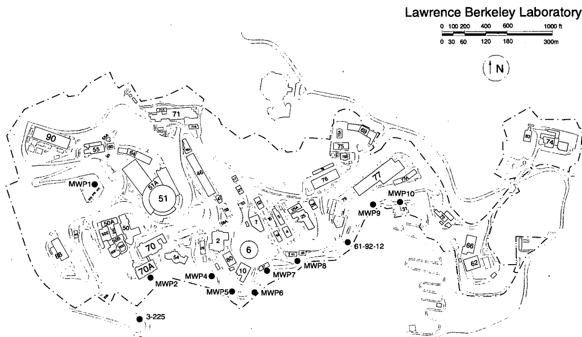
Figure 7-2. Approximate Locations of Peripheral Monitoring Wells
