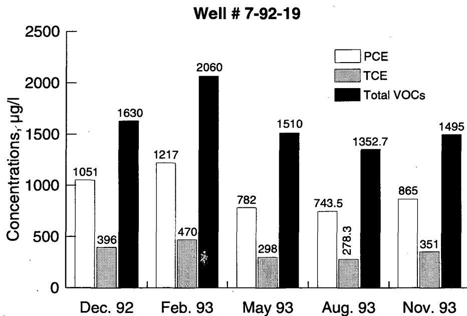
Figure 7-9. Time Variation of Contaminants in Well MW7-92-19
