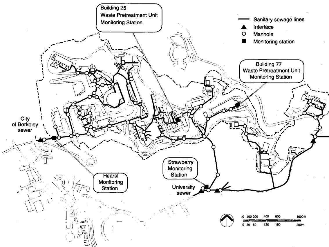
Figure 2-6. Sanitary Sewer System
