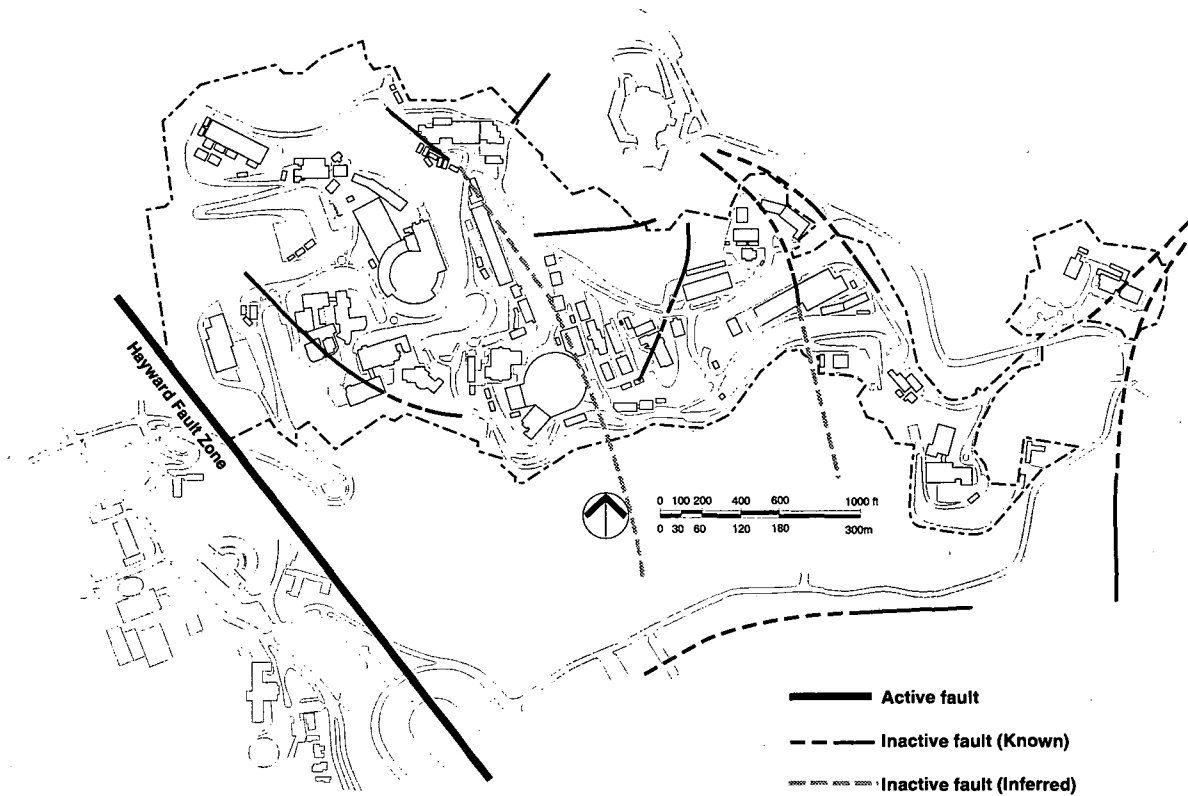
Figure 2-11. Mapped Faults
