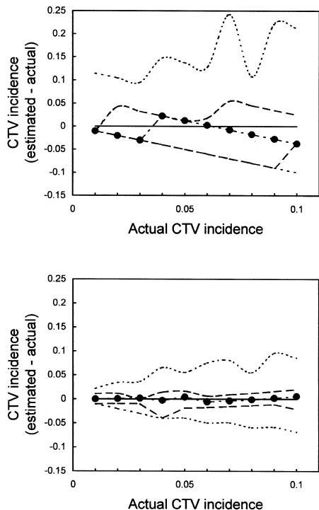
Fig. 3. Comparison of the CCTEA vs. HS sampling scheme. Figures represent the difference between observed and actual CTV incidence over a range (0.0 to 0.1) of actual CTV incidence. The top and bottom panels demonstrate, respectively, the incidence estimations resulting from the use of Equation 1 for the CCTEA and HS sampling schemes, respectively. The dotted intervals show the range covering all simulations (Lower dotted line in top panel is below the scale presented). The dashed intervals show the range covering the 25th to 75th percentiles. The dashed line joining the points shows the median value for the simulations. The solid horizontal line represents zero difference between observed and actual CTV incidence. Note the considerable improvement in mean estimations and reduced variance associated with the HS sampling scheme compared to the CCTEA scheme.
