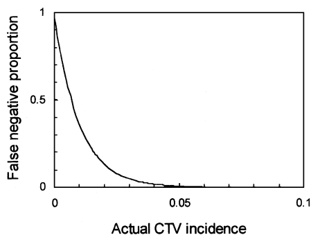
Fig. 5. The relationship between the proportion of false negative decisions and actual CTV incidence, if groves were classified as CTV-free on the basis of an assay of materials from 100 trees combined into a single group.
