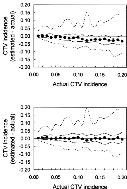
Fig. 4. Results of the simulation study of the HS sampling system when used to estimate the incidence of CTV for the CTV/ Toxoptera citricida pathosystem. Figures represent the difference between observed and actual CTV incidence over a range (0.0 to 0.2) of actual CTV incidence. The top and bottom panels demonstrate, respectively, the corrected ( n = 3.3 ) and uncorrected ( n = 4 ) incidence estimations resulting from the use of Equation 1. The dotted intervals show the range covering all simulations. The dashed intervals show the range covering the 25th to 75th percentiles. The dashed line joining the points shows the median value for the simulations. The solid horizontal line represents zero difference between observed and actual CTV incidence. Note the second panel, representing use of the modified Equation 1, provides apparently unbiased estimates of CTV incidence.
