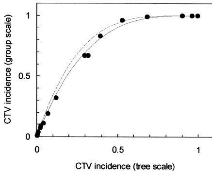
Fig. 2. The relationship between the incidence of CTV at the quadrat scale and its corresponding incidence at the single-tree scale. Data derived from disease assessments from CTV plots in northern Costa Rica are indicated by filled circles; the curve indicated by the dashed line is derived from the binomial distribution; the curve indicated by the solid line is derived from Equation 1.
