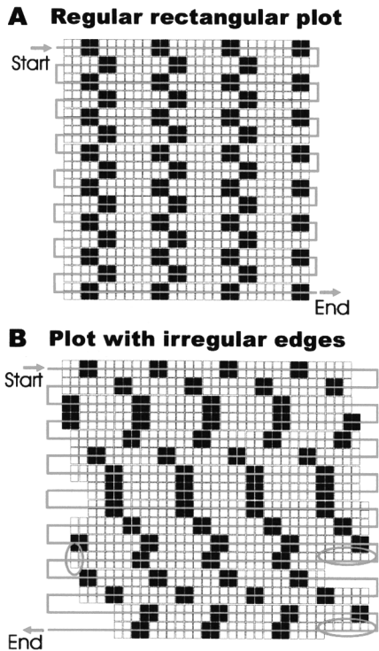
Fig. 1. Diagrammatic representation of the field implementation of the hierarchical sampling scheme. Position of individual trees is represented by black (sampled) or white (unsampled) squares. The gray line represents the path traversed by the field sampling team. The scheme requires the random selection of one of the first four groups of four trees as a starting point. In the examples above, the second group of four trees was randomly selected as a starting point. Leaf petioles are collected from each tree within a group and the collected materials are bulked. From this, the CTV status of the group is determined by ELISA. The incidence of CTV-positive groups is related to the incidence of CTV-positive trees, as described in the text by equation 1. A) Scheme for regular rectangular field. B) Scheme compensating for field with irregular boundaries.
