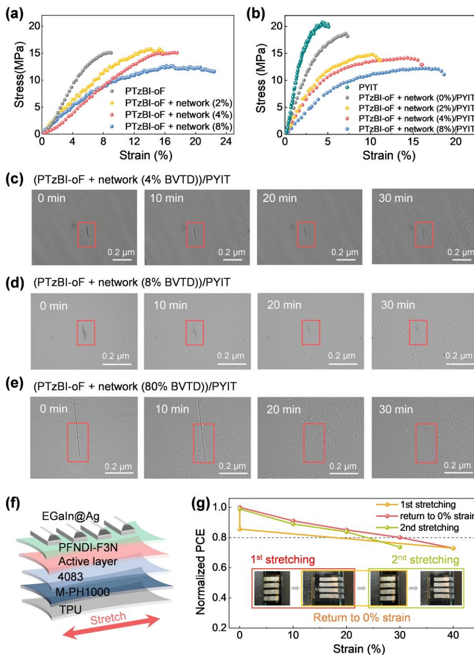
7 8 Fig. 5 Stress-strain curves of (a) neat PTzBI-oF films and (b) PTzBI-oF/PYIT blend 9 films incorporating a self-healable network with varying BVTD ratios (2%, 4%, and
