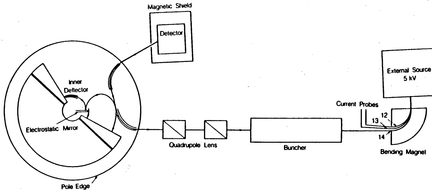
Figure 18 The scheme for radially injecting ions from an external ion source into the center of the cyclotron is shown in this figure. The beam from a conventional negative carbon ion source is sent through a bending magnet where the mass 12 and 13 beams are removed and measured. A buncher velocity modulates the beam so that the ions bunch at the first gap crossing. A deflector brings the beam into the magnet and directs it to an electrostatic mirror which bounces it through another deflecting channel and then into the dees where acceleration, focusing and extraction proceed as before. The bending magnet may be replaced by an ExB velocity selector which has the advantage of eliminating high velocity mass 12 and 13 ions which will be present in sputter ion source.
