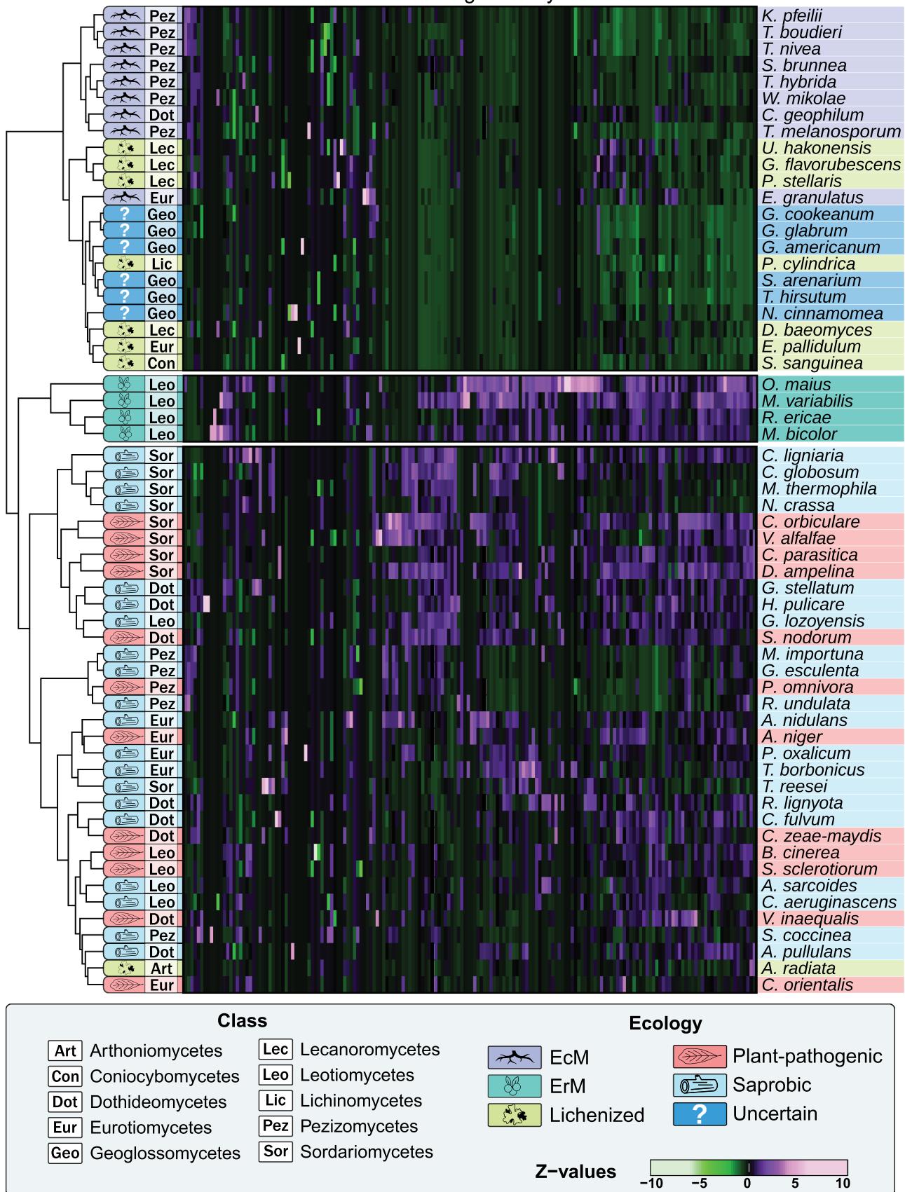
Figure 3. Members of Geoglossomycetes cluster with symbiotic fungi from Pezizomycotina based on CAZyme content. Heatmap and dendrogram were generated from 20 216 detected CAZyme-coding genes comprising 195 detected CAZyme families from 59 taxa. Values of CAZyme counts were centered prior to mapping, and unit variance scaling was applied to rows. Columns were clustered with Manhattan distance and Ward linkage.
