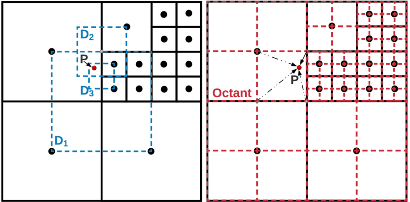
(a) Reconstruction with dual cells.
