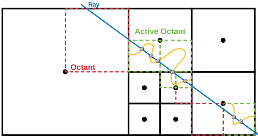
(b) Our “hybrid” implicit isosurface ray tracing.
