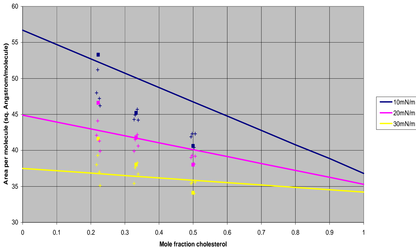
Figure 4B: Mean molecular area vs. composition. Experimental points are from the isotherms of Chol:egg SM mixtures. Crosses represent Chol mole fractions just around predicted critical concentrations of 0.22, 0.33 and 0.50 mole fractions. Squares are the exact Chol superlattice mole fractions of 0.22, 0.33 and 0.50. Solid lines represent ideal mixing of mean molecular area at the designated surface pressure and were calculated using Equation 2 in Materials and Methods.
