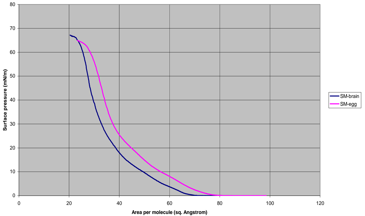
Figure 3: Pressure-area ( \Pi -A) isotherms of bovine brain SM and egg SM on pure water at 22°C
