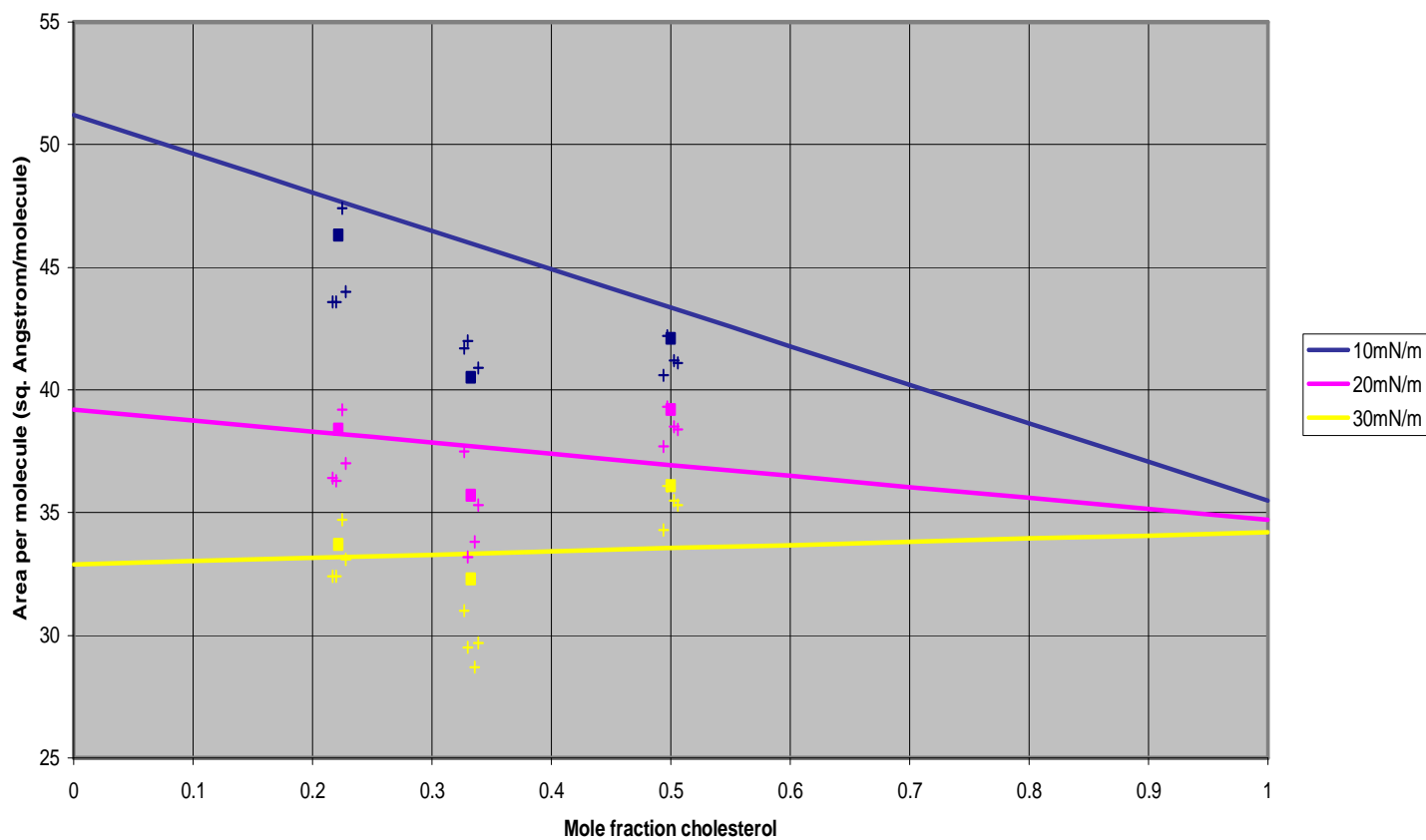
Figure 4A: Mean molecular area vs. composition. Experimental points are from the isotherms of Chol:brain SM mixtures. Crosses represent Chol mole fractions just around predicted critical concentrations of 0.22, 0.33 and 0.50 mole fractions. Squares are the exact Chol superlattice mole fractions of 0.22, 0.33 and 0.50. Solid lines represent ideal mixing of mean molecular areas at the designated surface pressures and were calculated using Equation 2 in Materials and Methods.
