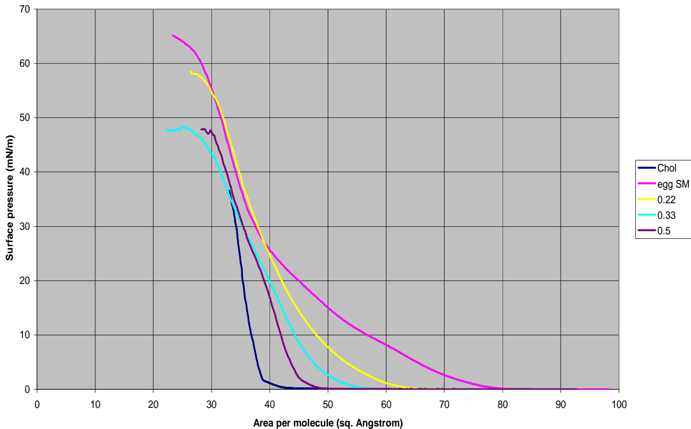
Figure 2: Pressure-area ( \Pi -A) isotherms of Chol, egg SM and mixtures of egg SM-cholesterol on pure water at 22°C. Cholesterol mole fractions are as indicated in the legend.
