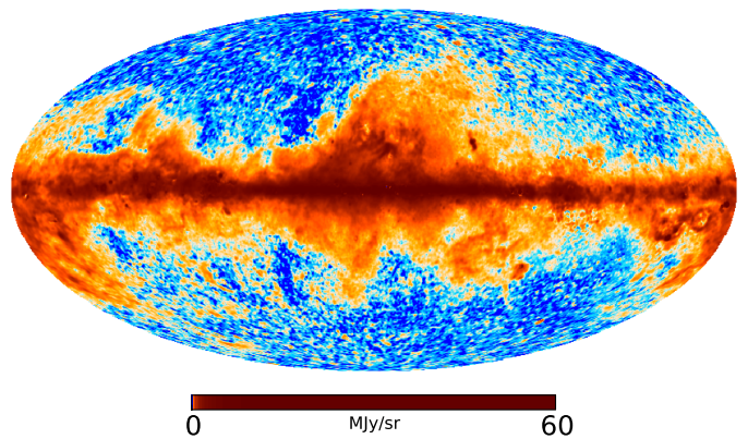
Fig. 8. Template of spinning dust intensity.
