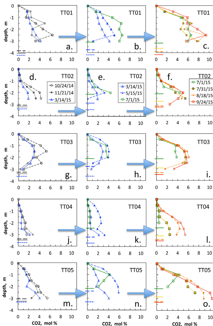
Fig. 6. Depth profiles of unsaturated zone \text{CO}_2 concentrations. Seasonal changes in profiles are displayed in left, middle, and right graphs for each of the five sites (sampling dates for all sites are indicated in panels d–f). Horizontal lines along the left axes indicate water table depths at the time of gas sampling.
