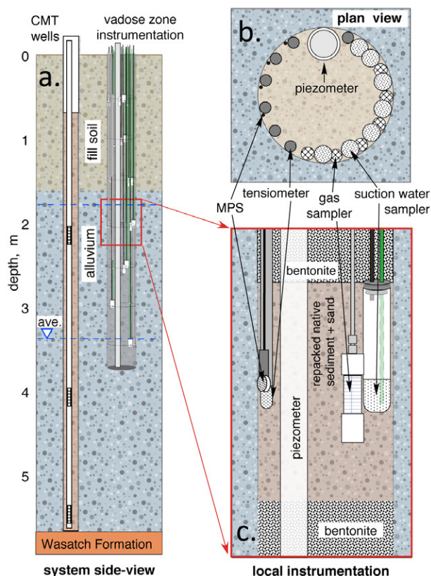
Fig. 2. Installation of borehole instruments. (a) Schematic cross-section of vadose zone instrumentation borehole and multilevel groundwater sampling wells. (b) Plan view of vadose zone instrument distributions along borehole wall. (c) Side view of vadose zone instruments within a given depth. (d) Instruments to be installed in a single borehole (the green pipe was only used to deliver backfill sediments and bentonite to depths greater than 2.5 m). (e) View down partially completed borehole. (f) Near-surface bentonite layer (0.3- to 0.2-m depth). (g) Completed instrumentation, showing tops of tensiometers, soil water samplers, gas samplers, Tensiometer, and several collars for soil surface CO 2 flux measurements.
