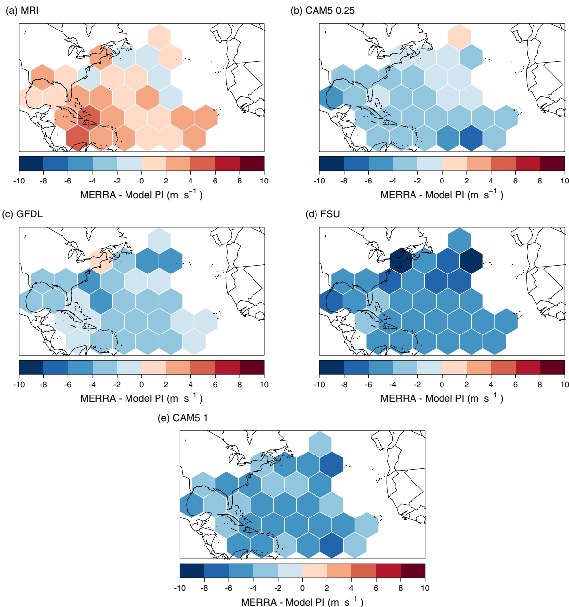
Figure 10. Difference maps depicting the difference in observed (MERRA)—simulated (model) per region maximum potential intensity (PI) in units of \text{m s}^{-1} for the (a) MRI-AGCM, (b) CAM5 0.25^\circ , (c) GFDL-HIRAM, (d) FSU-COAPS, and (e) CAM5 1^\circ models.
